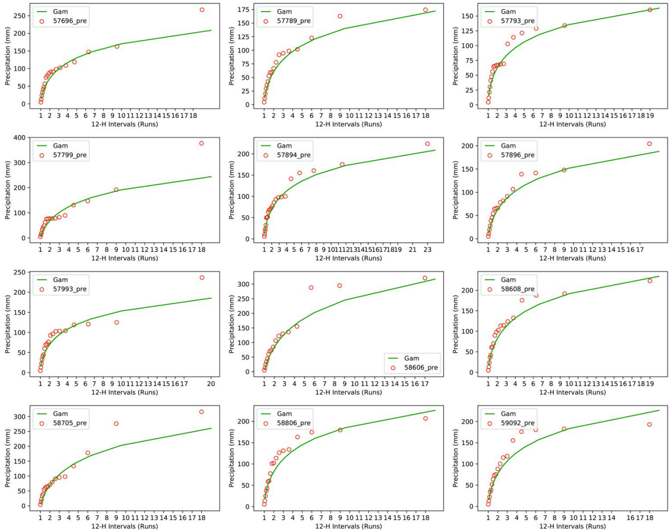
Figure 3 Cumulative precipitation of runs of events. The orange hollow points show observed precipitation events. The green lines represent their gamma estimates
