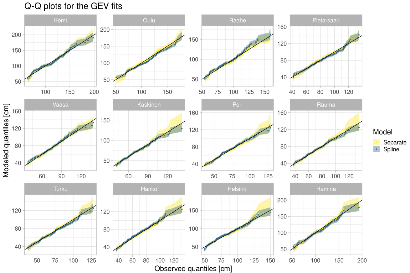
Figure 3. Quantile-quantile plots showing the modeled quantiles for tide gauge specific fits (Separate) and for Spline when plotted against the observed quantiles. Median values are given as points and the shading shows the 95% uncertainty range for the modeled quantiles. The diagonal line is also shown in each panel.
