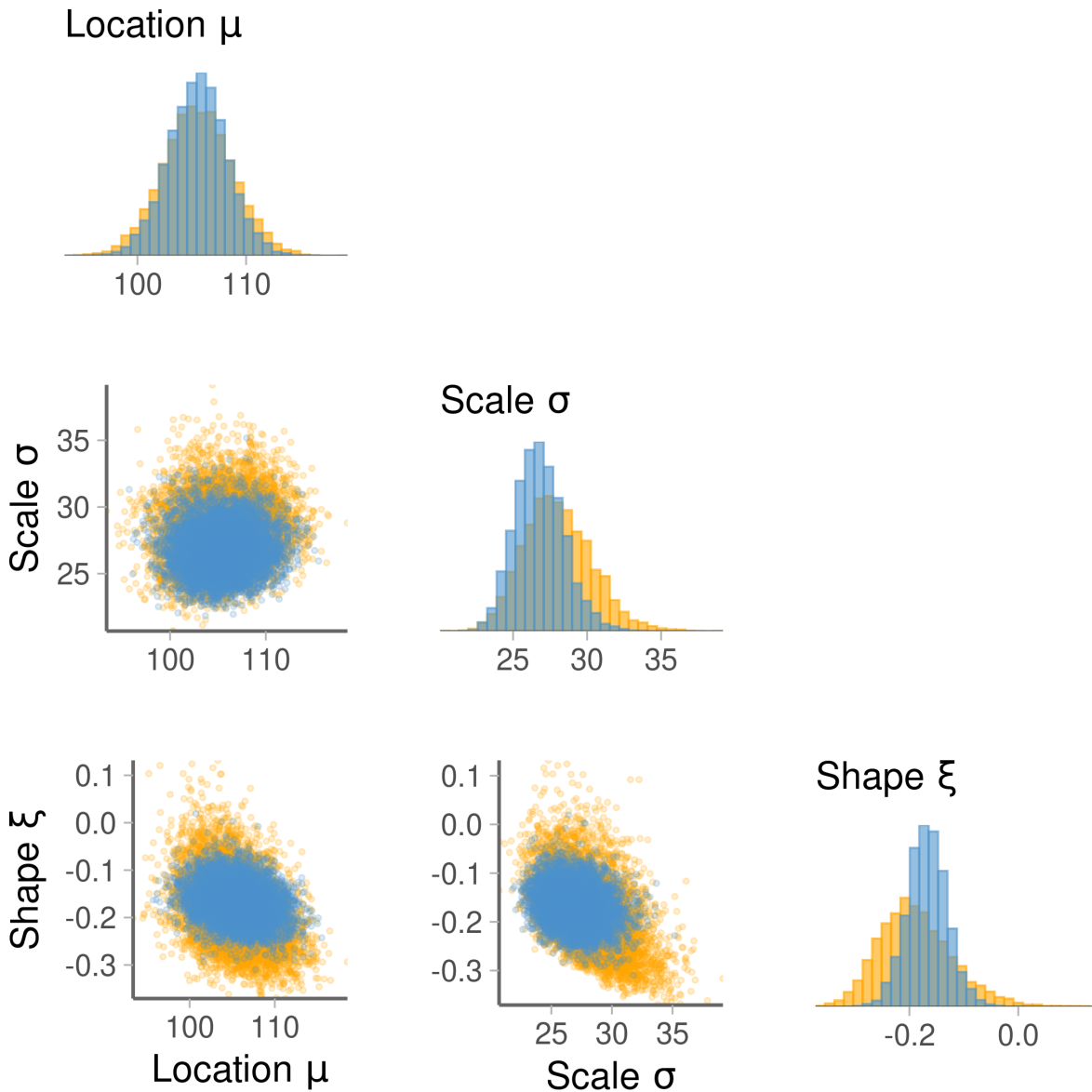
Figure 5. Example of posterior distributions for the GEV parameters in Kemi tide gauge obtained with (orange) Separate and (blue) Spline, respectively. Histograms of the three GEV parameters are shown on the diagonal and the corresponding bi-variate scatter plots on the lower triangle. The location and scale parameter values are given in centimeters.
