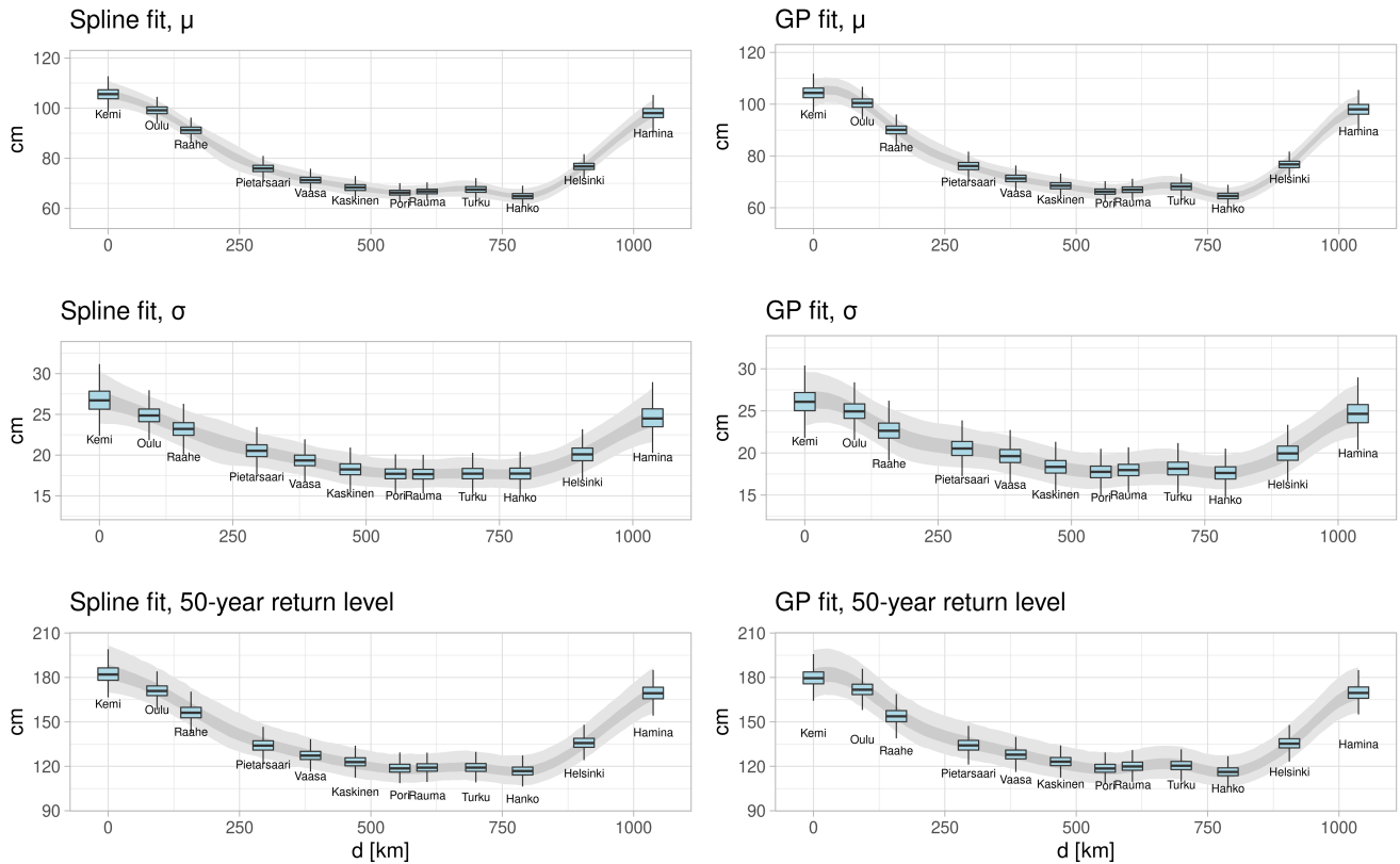
Figure 2. Illustration of the (left) spline and (right) Gaussian process fits for the (top) location and (middle) scale parameter with respect to the distance from Kemi tide gauge. Darker (light) shading denotes the interquartile (95 %) range of the parameter estimates. The figure also shows box-plots of the corresponding parameters at the tide gauge locations. The bottom row shows similar plots for the 50-year return level of annual maximum sea levels for both models. The box covers the interquartile range (IQR) and the median value is highlighted by the horizontal line. The length of the whiskers is one and half times the IQR.
