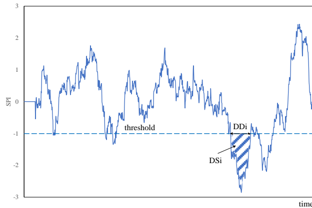
Figure 2. Drought characteristics identification using the ‘run theory’ (Yevjevich 1967).
