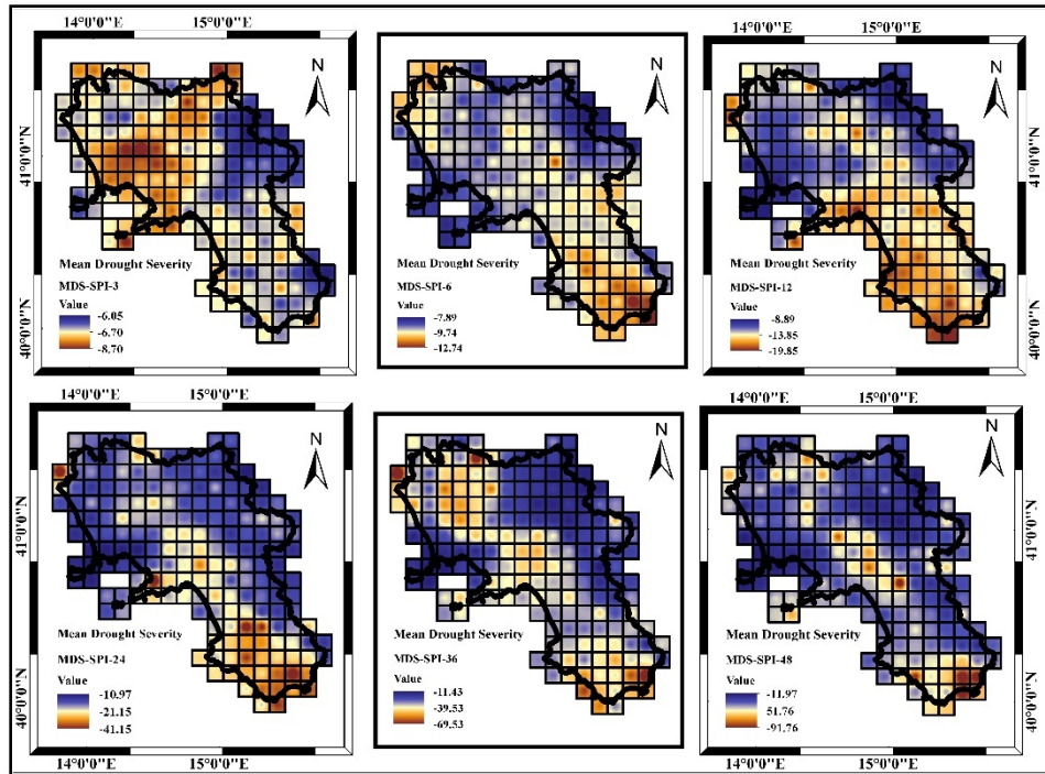
Figure 9: MDS (mean drought severity) for the different considered accumulation periods (SPI ≤ -1).
