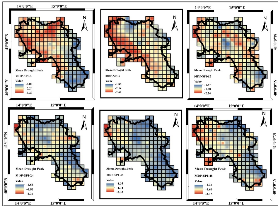
305 Figure 10: MDP (mean drought peak) for the different considered accumulation periods (SPI ≤ -1).
