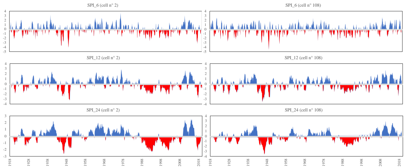
220 Figure 3. SPI_6, SPI_12 and SPI_24 for cell n°2 (southern area – left panel) and cell n° 108 (northern area – right area).
