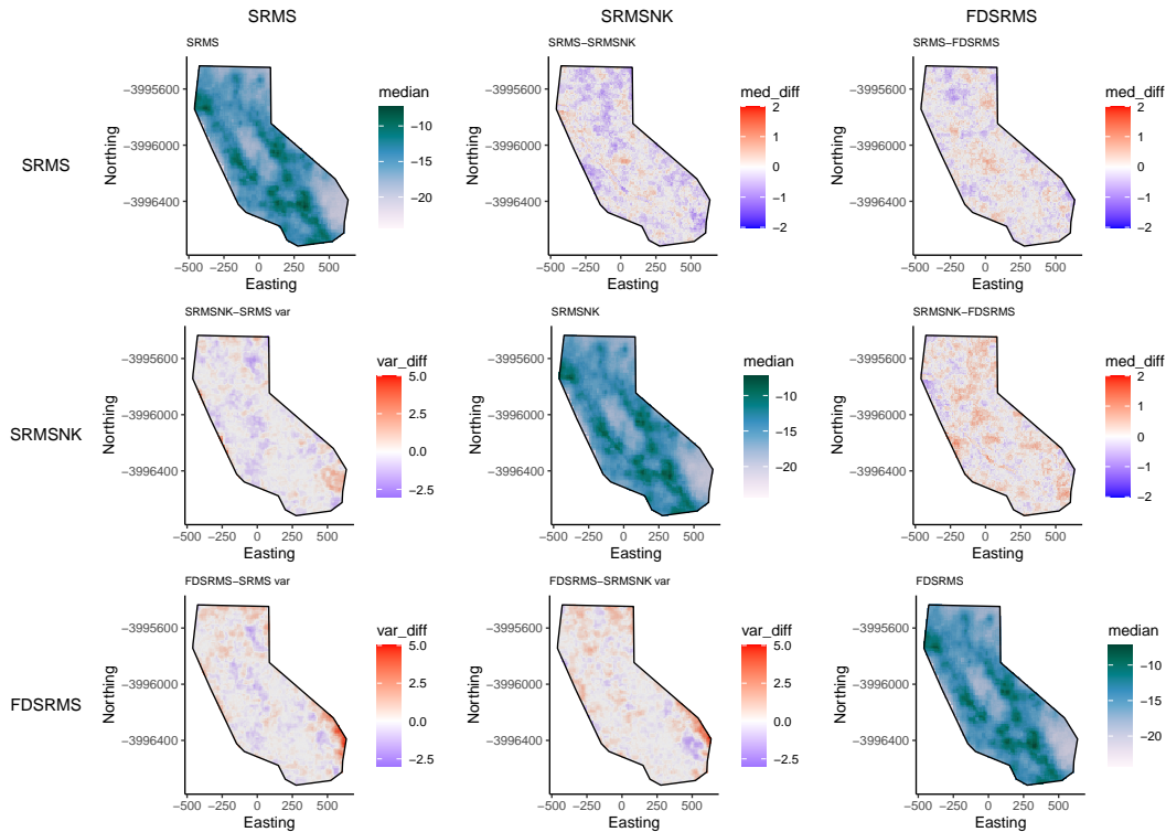
Figure 3. Posterior mean intensity Pairwise comparison of models for full catalogue models. The top-right side of the six-in-labru -plot shows differences in log median intensity and the lower left section shows the differences in model variances between the different models created with full . The median log intensities for each model are shown on the diagonal. Models include combinations of smoothed past seismicity ( topMS ), strain rate (SR), fault distance (FD) and declustered -fault slip rates ( bottomNK ) catalogues of events from 1985-2004.
