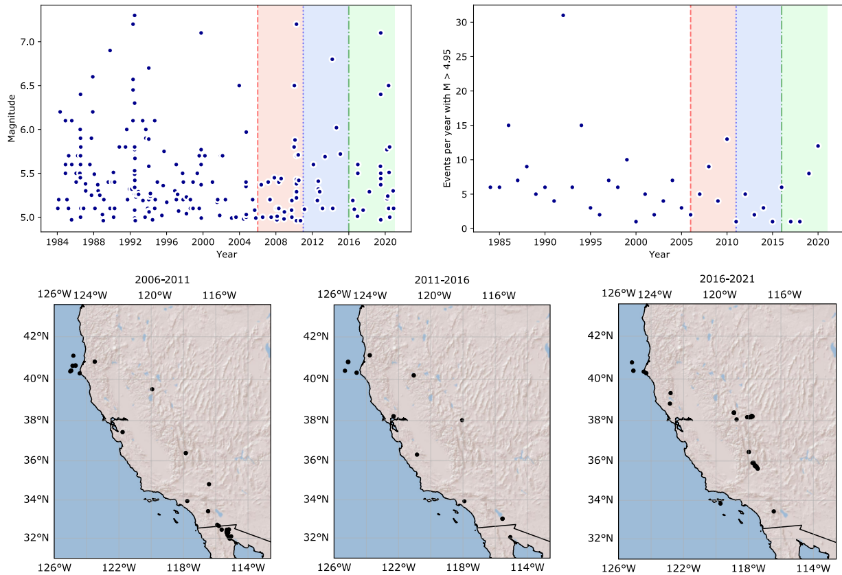
Figure 9. Top: Catalogue of events in California from 1985-2021. The period 1984-2004 is used for model construction, and the three testing periods are shown with red, blue and green backgrounds. The left panel shows the magnitude of events in time and the right the number of events in each year. Bottom: the comcat catalogues for the three five-year testing intervals.
