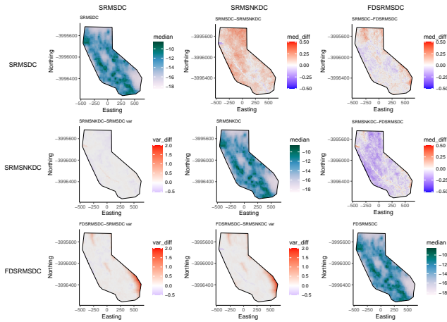
Figure 2: Pairwise comparison of models for declustered catalogue models. The top-right side of the plot shows differences in log median intensity and the lower left section shows the differences in model variances between the different models. The median log intensities for each model are shown on the diagonal. Models include combinations of smoothed past seismicity (MS), strain rate (SR), fault distance (FD) and fault slip rates (NK).
