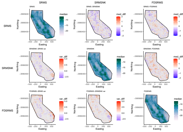
Figure 1: Pairwise comparison of models for full catalogue models. The top-right side of the plot shows differences in log median intensity and the lower left section shows the differences in model variances between the different models. The median log intensities for each model are shown on the diagonal. Models include combinations of smoothed past seismicity (MS), strain rate (SR), fault distance (FD) and fault slip rates (NK).
