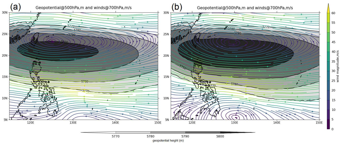
630 Figure 13: Geopotential height at 500hPa in geopotential meters shaded contour lines and winds (streamlines) at 700hPa averaged over the entire period of the simulation with (a) KF (corresponding to kfsnoffs1) and (b) TK (corresponding to tksnoffs1). The 6-hourly WRF output was interpolated to the coarser 6-hourly ERA5 grid using First-order Conservative Remapping through CDO remapcon function. CDO code available at https://code.mpimet.mpg.de/projects/cdo/
