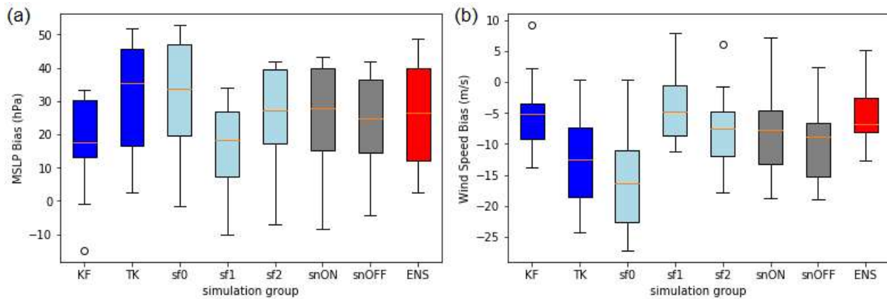
550 Figure 10: Mean biases for (a) MSLP in hPa and (b) maximum winds in ms-1 for each group of simulations: cumulus schemes KF and TK (blue bars), surface flux options (sf0, sf1, sf2) (light blue bars), spectral nudging ON and OFF (gray bars), and mean of the different experiments using four randomly selected EDA ensemble members (ENS) (red bars) as initial and boundary conditions.
