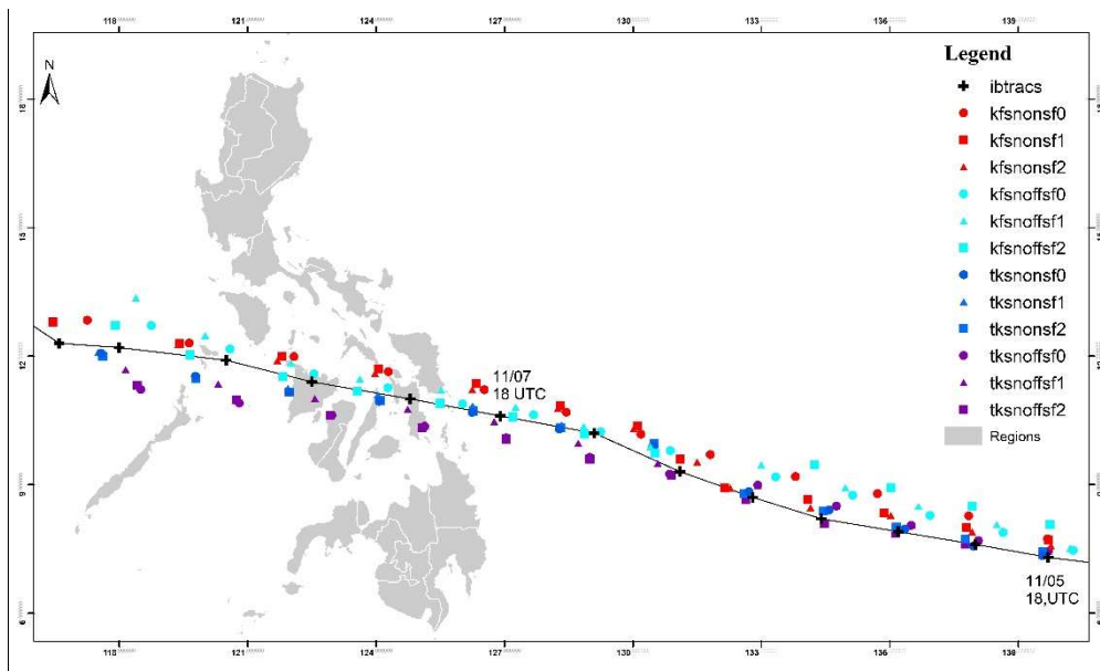
375 Figure 2: Simulated tracks compared with IBTRACS and the sensitivity experiments classified according to experiment groups: Kain-Fristch (KF) convection scheme; TK (TK) convection scheme; with spectral nudging (snON); without nudging (snOFF); surface flux option 0 (sf0); option 1(sf1); and option 2 (sf2).
