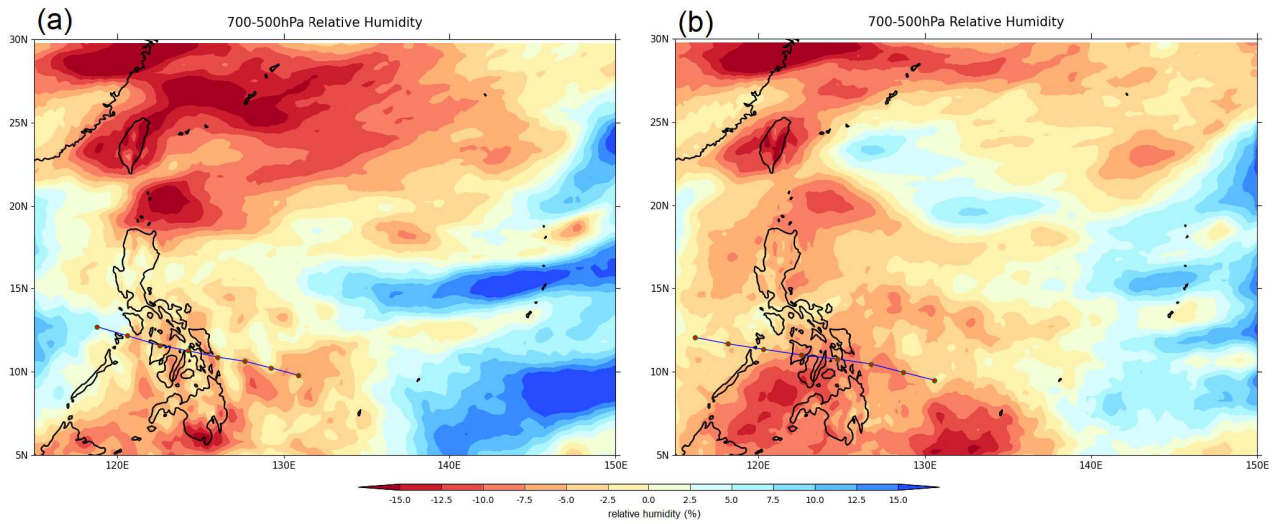
645 Figure 14: The difference of the simulated Mid-tropospheric (700-500hPa) Relative Humidity averaged over the entire period of the simulation with (a) KF (corresponding to kfsnoffs1) and (b) TK (corresponding to tksnoffs1) from ERA5. The 6-hourly WRF output was interpolated to the coarser 6-hourly ERA5 grid using First-order Conservative Remapping through CDO remapcon function. CDO code available at https://code.mpimet.mpg.de/projects/cdo/
