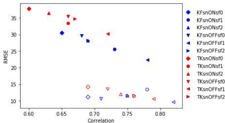
460 Figure 6: RMSE vs CC for minimum sea level pressure in hPa (filled) and for maximum winds in ms-1 (not filled) for the sensitivity experiments
