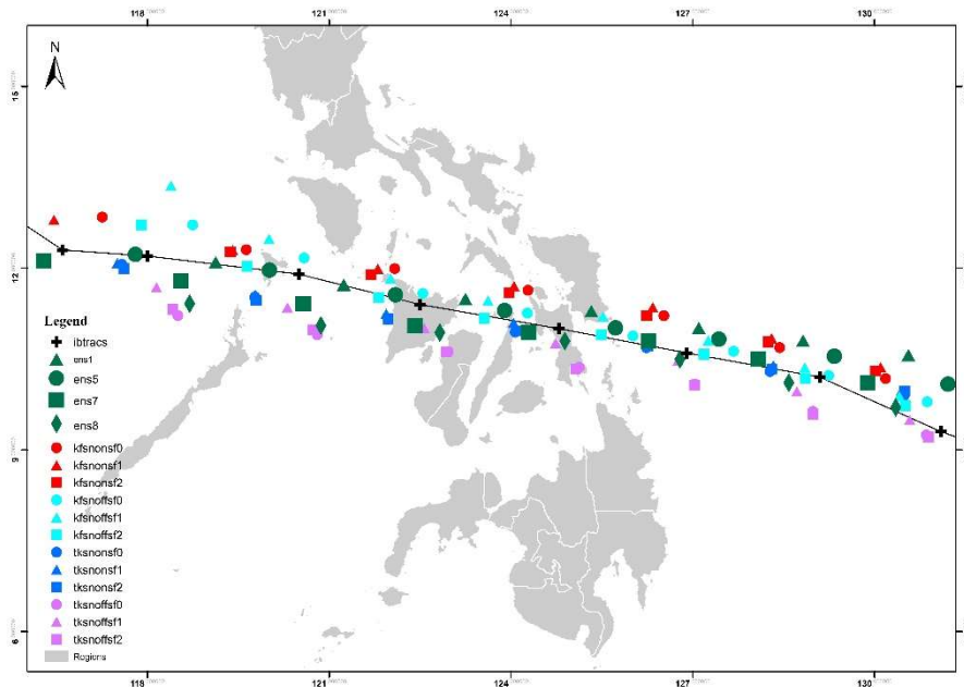
540 Figure 9: Simulated tracks of the four randomly selected EDA Ensemble Members (green) compared with IBTRaCS and the sensitivity experiments classified according to experiment groups: Kain-Fristch (KF) convection scheme; TK (TK) convection scheme; with spectral nudging (snON); w nudging (snOFF); surface flux option 0 (sf0); option 1 (sf1); and option 2 (sf2).
