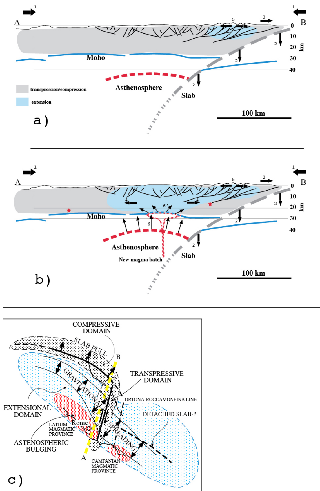
Figure 12 a-b) Interpretative geodynamic cross-section and (c) map of central Italy, explaining the superimposition of two competitive stress-field (extension and transpression) in this region (see text for explanations). Red stars are the hypocenters of the two earthquakes occurred in this region with fault plane solution showing anti-apenninic (NE-SW) P -axis.
