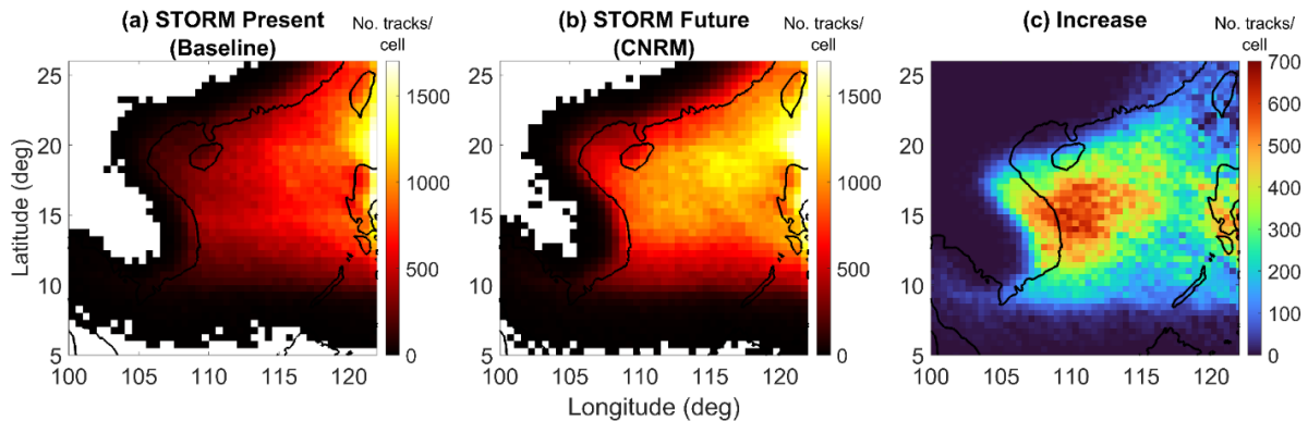
Figure 5 - Track density = the number of Saffir Simpson category 1-5 TC tracks passing through each 0.5^\circ \times 0.5^\circ grid cell within each ~35 year period. Left: Baseline STORM track density of Saffir Simpson Category 1+ (i.e., excluding Tropical Storms), Middle: CNRM-CM6-1 climate model- Future STORM track density, of Saffir Simpson Category 1+, and Right: The cyclone track density difference between them.
