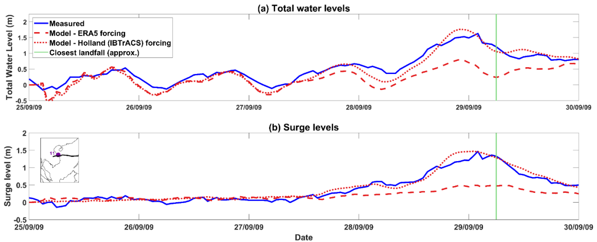
Figure 4 – (a) measured and modelled total water levels, and (b) measured and modelled storm surges at Son Tra (site 11 in Fig.1) for Typhoon Ketsana, which made landfall at approximately 6am UTC on 29 th September 2009 (green vertical line). 345 Modelled total water level and surges using ERA5 (red dashed) and Holland Model (red dotted) wind and pressure fields against measured data (blue).
