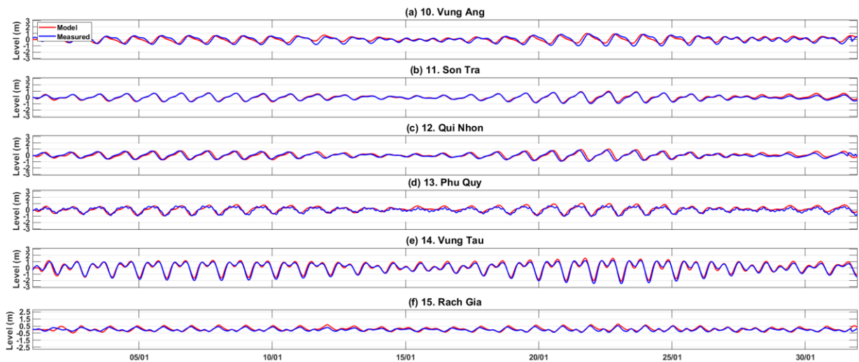
250 Figure 3 - Comparison of modelled (red) and measured (blue) astronomical tidal time series (January 2019) at six Vietnamese tide gauge station locations (see Fig.1 for locations).
