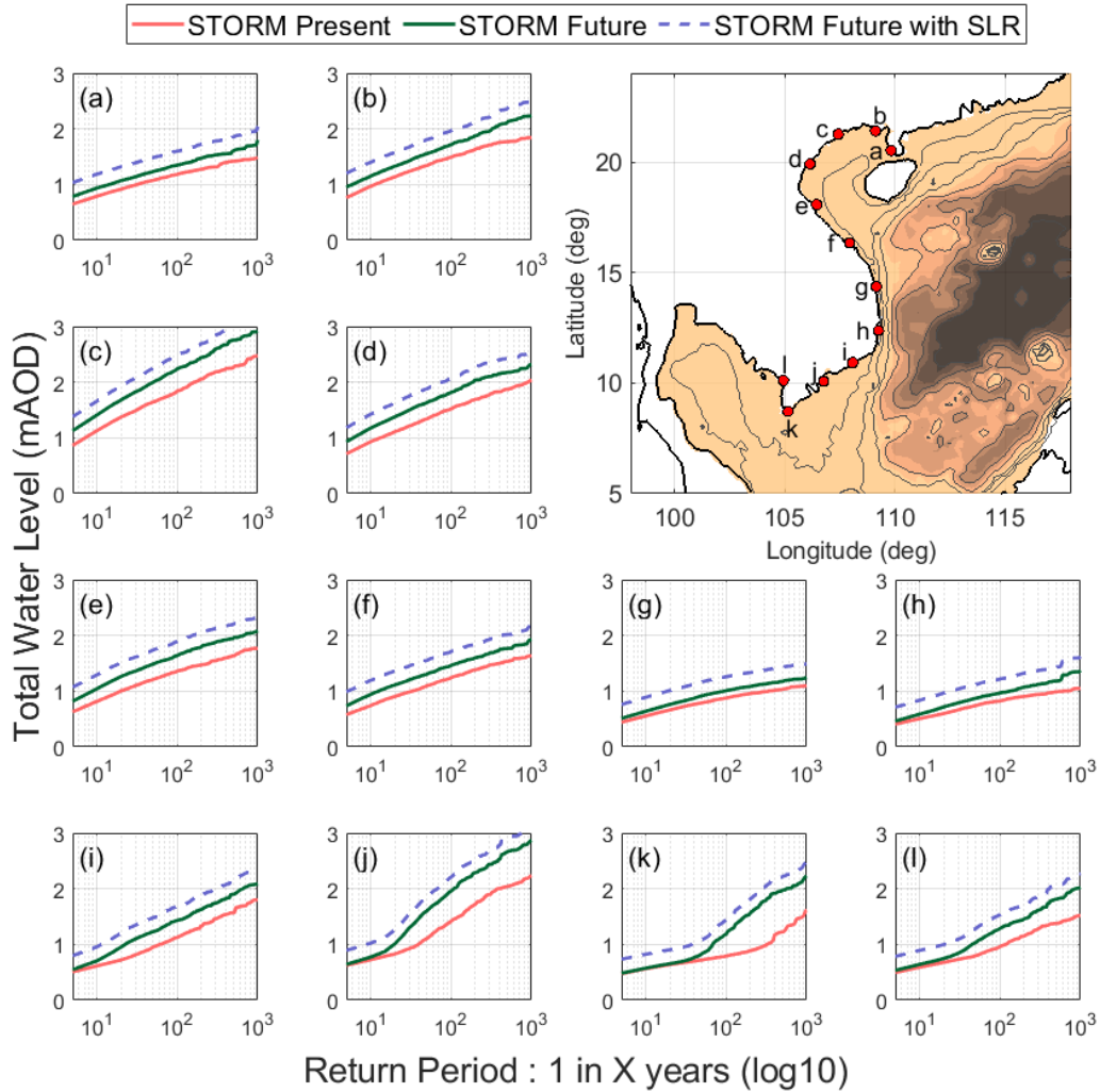
Figure 8 - The relationship between past/present baseline (red) and future (green) total water level return period (Log scale, 1:X years) at equidistant locations at and around the Vietnam and South China coastline. Future return periods with 0.25 mean sea level rise, due to climate change by 2050, is shown with a dashed blue line.
