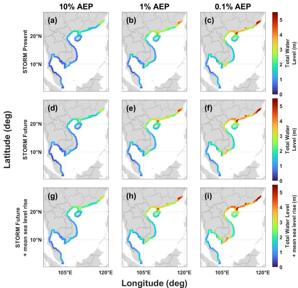
570 Figure 7 - The 10% AEP (a,d,g), 1% AEP (b,e,h) and 0.1% AEP (c,f,i) total water level (tide + surge heights) for the China, Vietnam, Cambodia, Thai and Malaysian coastlines in the model. First row: STORM baseline data (1980-2018); second row: CNRM-CM6-1 climate model STORM Future data (2015-2050) total water levels; third row: CNRM-CM6-1 climate model STORM Future data total water levels with 0.25m addition for rising mean sea levels up to 2050.
