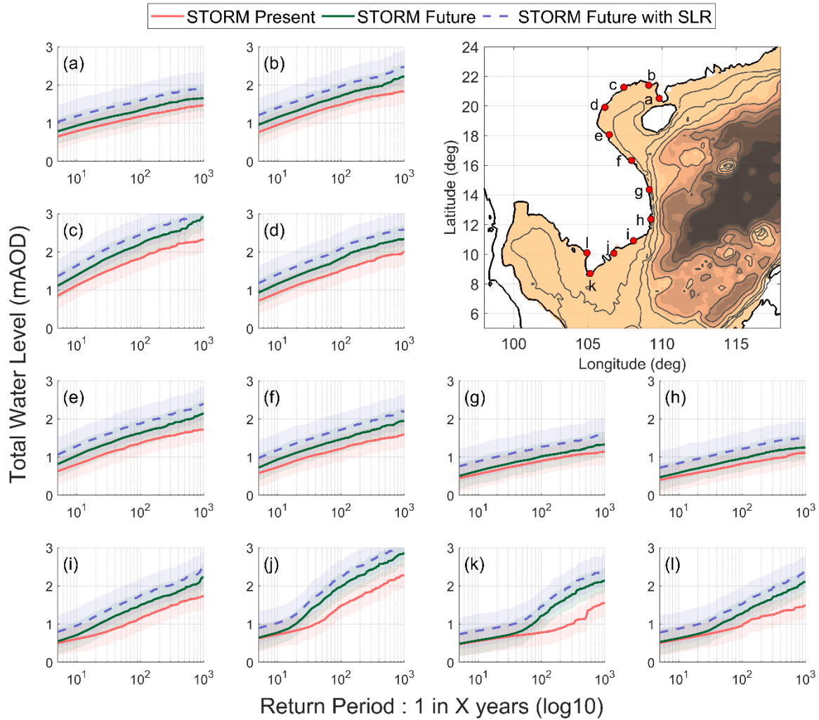
Figure 8 - The relationship between past/present baseline (red) and future (green) total water level return period (Log scale, 1:X years) at equidistant locations at and around the Vietnam and South China coastline. Future return periods with 0.25 mean sea level rise, due to climate change by 2050, is shown with a dashed blue line. Shaded areas indicate the 95 th percent confidence level around each mean total water level return period value.
