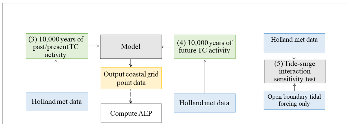
Figure A53 – MIKE 21 hydrodynamic model configuration for (3) past/present scenario; the (4) future scenario and (5) testing the model sensitivity to tide-surge interactions (see Section 3).
