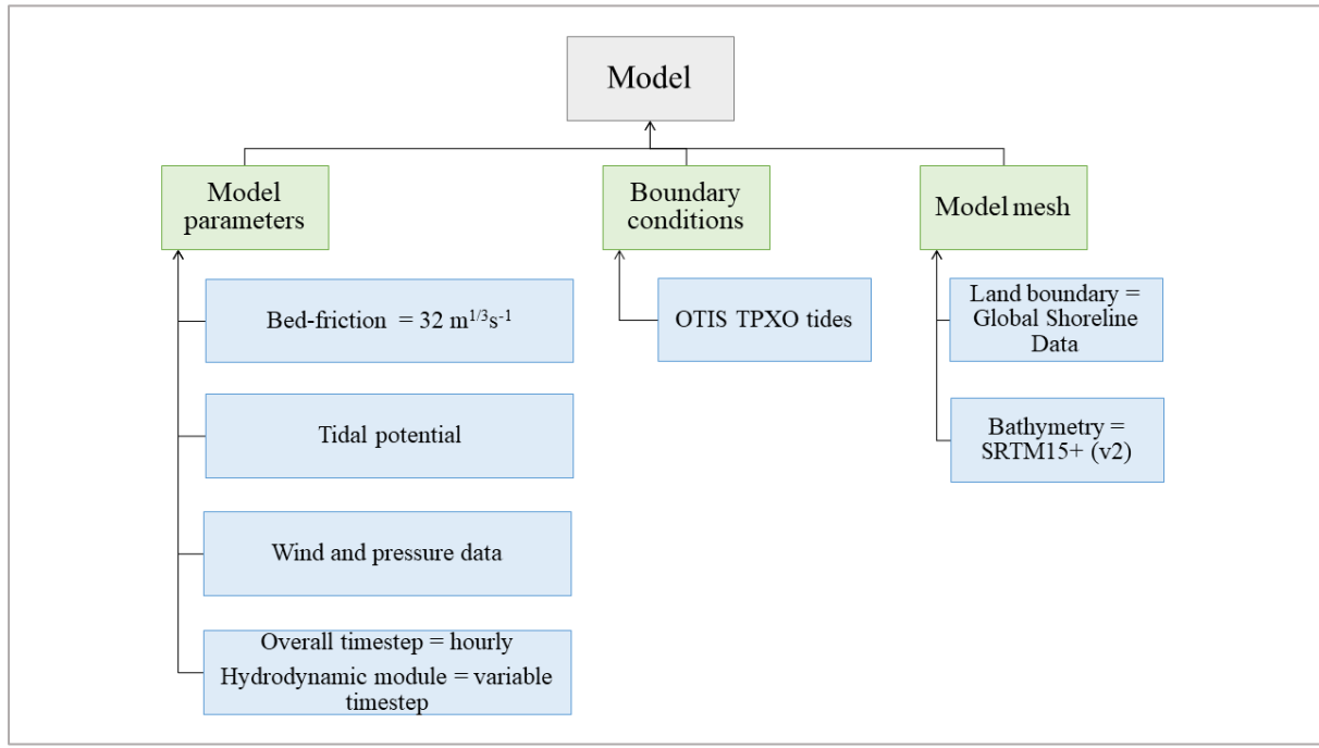
Figure S1-A1 – The basic model configuration
