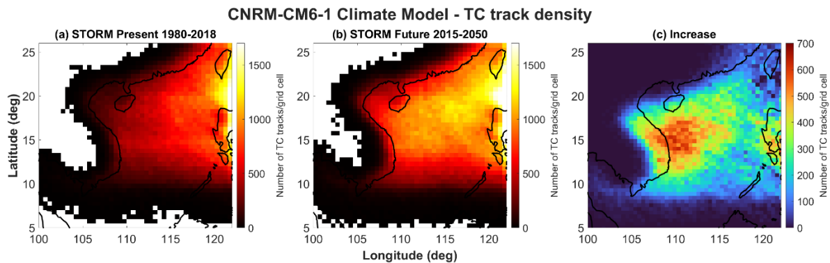
415 Figure 5 - Track density = the number of Saffir Simpson category 1-5 TC tracks passing through each 0.5^\circ \times 0.5^\circ grid cell within each ~35 year period. Left: Baseline STORM Past/Present track density of Saffir Simpson Category 1+ (i.e., excluding Tropical Storms), Middle: CNRM-CM6-1 climate model- Future -STORM Future track density, of Saffir Simpson Category 1+, and Right: The cyclone track density difference between them.
