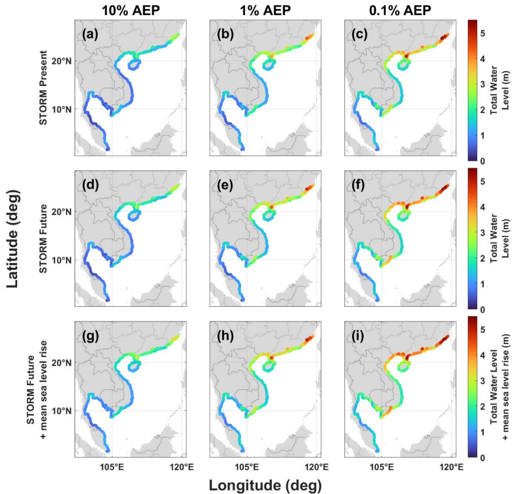
580 Figure 7 - The 10% AEP (a,d,g), 1% AEP (b,e,h) and 0.1% AEP (c,f,i) total water level (tide + surge heights) for the China, Vietnam, Cambodia, Thai and Malaysian coastlines in the model. First row: STORM baseline data (1980-2018); second row: CNRM-CM6-1 climate model STORM Future data (2015-2050) total water levels; third row: CNRM-CM6-1 climate model STORM Future data total water levels with 0.25m addition for rising mean sea levels up to 2050.
