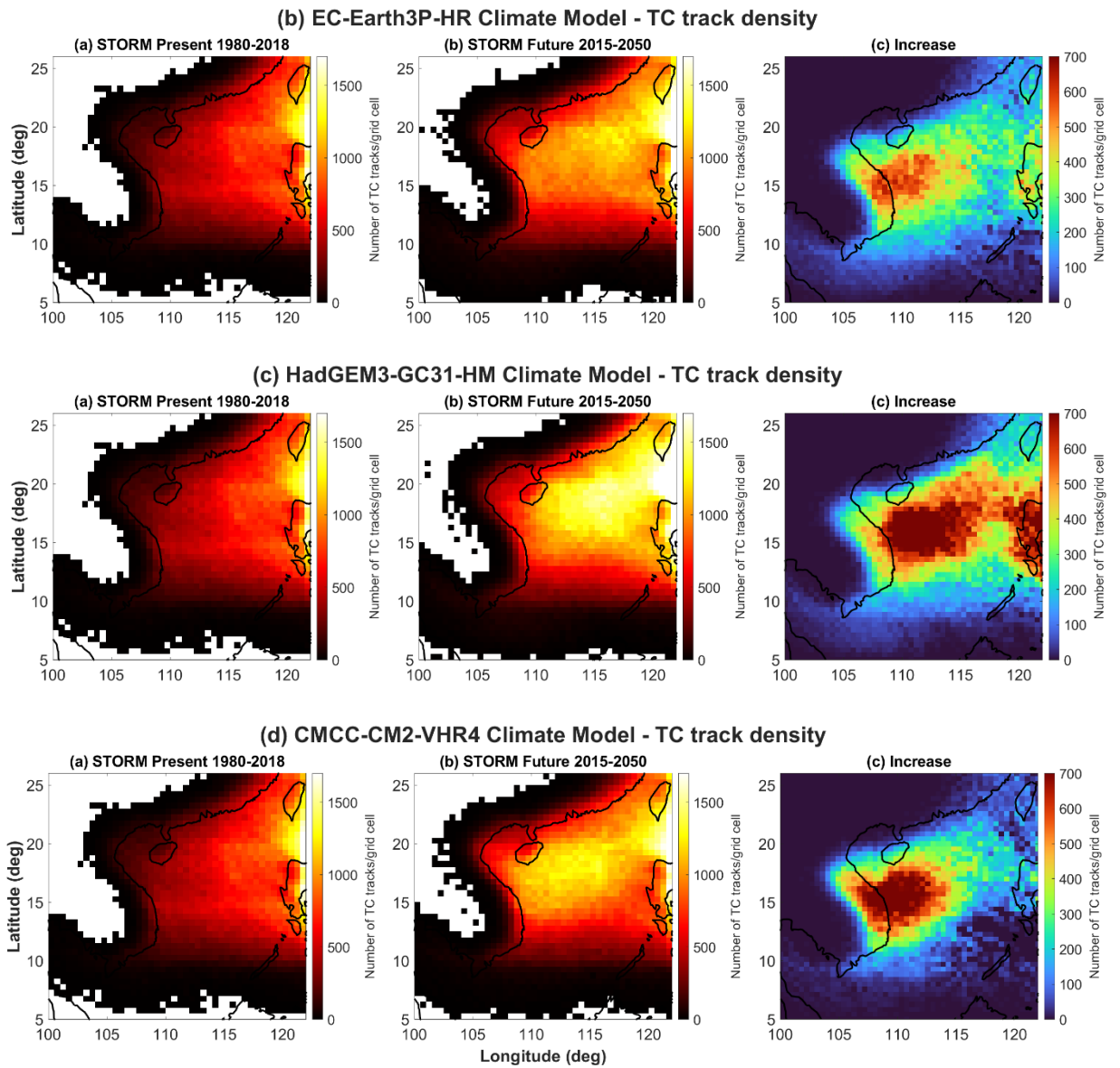
Figure A58 – To contrast with Figure 5 in the manuscript, here are the number of Saffir Simpson Category 1+ (i.e., excluding Tropical Storms) TCs that pass through a grid cell over a ~35 year period represented by STORM Past/Present (1980-2018, left column); and STORM Future (2015-2050, central column) for three alternative climate models. Right column: the difference between STORM past/present and STORM future (i.e. the projected increase). (b) EC-Earth 3P-HR climate model, (c) HadGEM3-GC31-HM climate model, (d) CMCC-CM2-VHR4 climate model.
