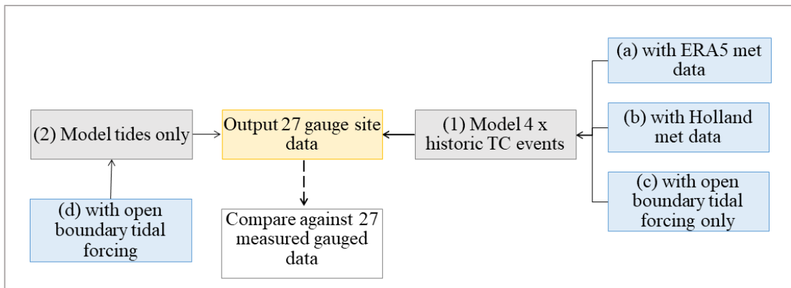
Figure A52 – Model validation. The storm surge validation process is described in section 2.3 of the paper; we use different wind and pressure input data to simulate historic TC events, using (1,a) ERA5; (1,b) Holland formula or (1,c) no meteorological forcing data. Separately, validation of astronomical tides is illustrated in schematic (2,d) with a tides-only model simulation, as described in Section 3 below, and in section 2.2 of the paper.
