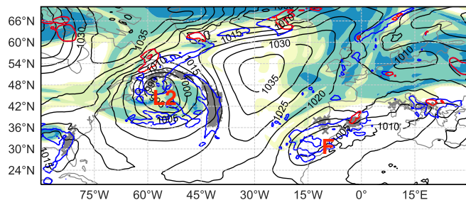
(e) 08 Jan 2021 00 UTC
