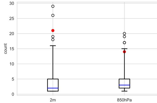
Figure 3. Boxplot of the duration of cold spells over Spain in the winters 1979-2019. Values are number of days with continuous minimum temperatures below 0^{\circ}\text{C} at 2 m and 850 hPa, respectively, in the area enclosed by the 5 mm snowfall contour in Fig. 1a. The blue lines denote the median, the boxes the inter-quartile range, the whiskers the 1st and 99th percentiles, and the open circles the outliers. The red circles denote the cold spell duration in early January 2021.
