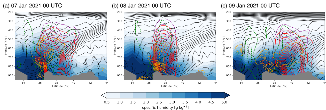
Figure 8. Vertical cross sections from 33^{\circ}\text{N} to 44^{\circ}\text{N} along 3^{\circ}\text{W} at (a) 00 UTC 07 January, (b) 00 UTC 08 January, and (c) 00 UTC 09 January 2021. Shown are equivalent potential temperature (black), specific humidity (blue shading), vertical motion (green; for -1 , -0.5 , 0.5 , and 1 \text{ Pa s}^{-1} ), rain water content (yellow), ice water content (purple), snow water content (red), and liquid water content (orange). The latter four variables are shown in intervals between 0.05 \text{ g kg}^{-1} and 0.55 \text{ g kg}^{-1} in 0.05 \text{ g kg}^{-1} increments.
