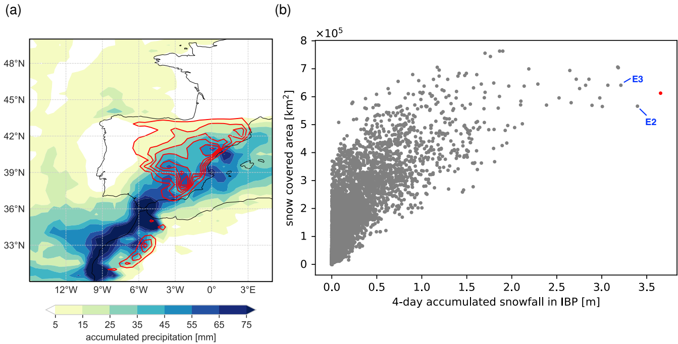
Figure 1. (a) Precipitation accumulated from 00 UTC 07 January to 00 UTC 11 January 2021 (from ECMWF short-range forecasts). The red contours denote the accumulated snowfall in this period, starting from 5 mm in 10 mm increments. (b) 4-day accumulated snowfall vs. snow covered area of all winters from 1979 to 2019 in the Iberian Peninsula (IBP), based on the method described in Sect. 2.3. The red point represents the period 07-10 January 2021 (Filomena), label E2 marks the period 02-05 January 1997 and E3 the period 28-31 January 1986.
