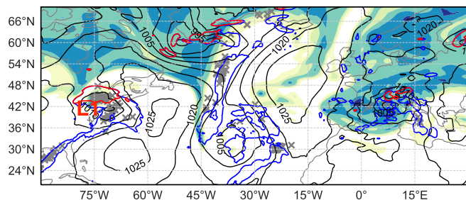
(c) 06 Jan 2021 00 UTC
