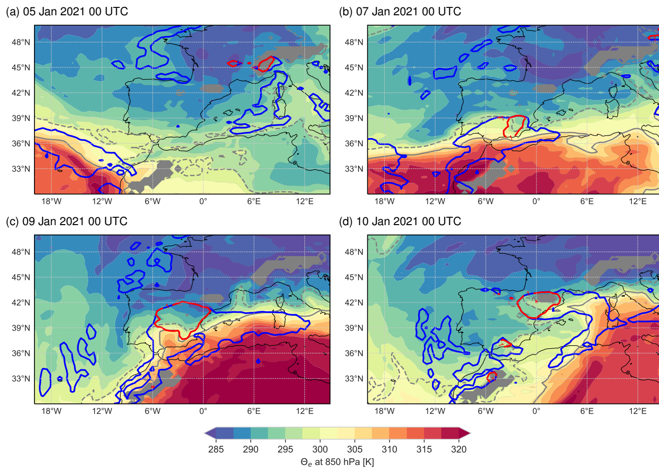
Figure 7. Maps with equivalent potential temperature ( \theta_e ) at 850 hPa (colour shading), 1-h total accumulated precipitation (blue contours for 1 mm), and 1-h accumulated snowfall (red contours for 1 mm). Panels are valid at (a) 00 UTC 05 January, (b) 00 UTC 07 January, (c) 00 UTC 09 January, and (d) 00 UTC 10 January 2021. The grey lines denote the anomaly of \theta_e at 850 hPa (solid: +4K, dashed: -4K), which is calculated with respect to a 21-day running mean.
