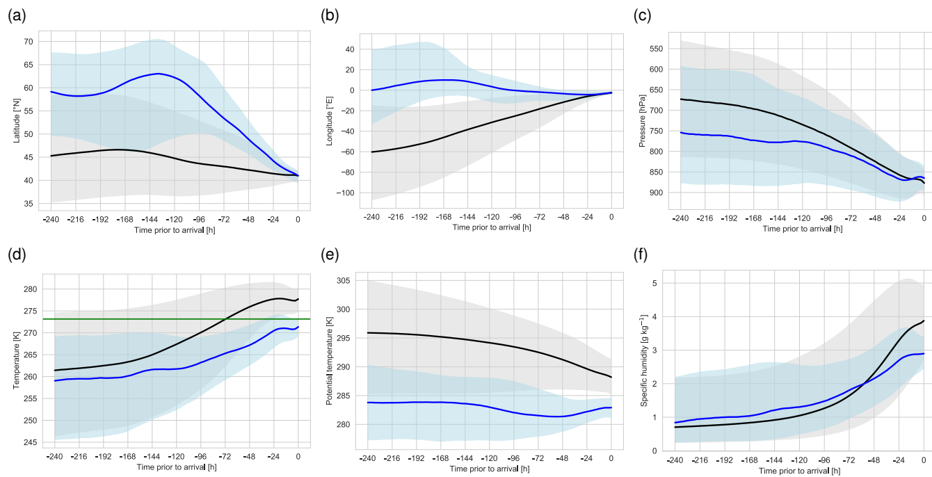
Figure 5. Time series along backward trajectories from Spain of (a-c) latitude, longitude, and pressure and (d-f) temperature, potential temperature and specific humidity. The grey colours denote values for the climatology and the blue colours for the cold spell in early January 2021. The bold lines denote the median and the shading the inter-quartile range. The green line in (d) marks a temperature of 0 °C.
