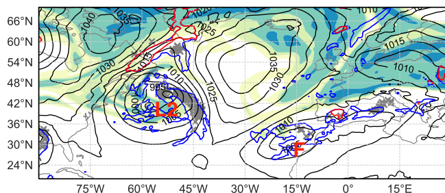
(f) 09 Jan 2021 00 UTC
