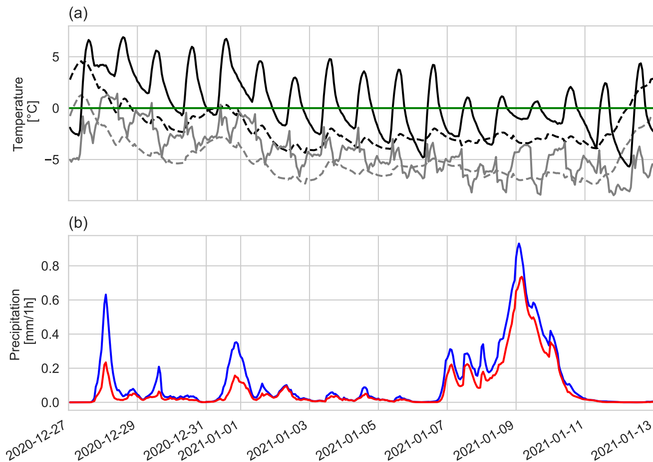
Figure 2. (a) Temporal evolution of 2-m temperature (solid) and 850-hPa temperature (dashed) over Spain from 27 December 2020 to 13 January 2021. Grey lines show anomalies. (b) Temporal evolution of precipitation (blue) and snowfall (red). All values are averaged over the area enclosed by the 5 mm snowfall contour in Fig. 1a.
