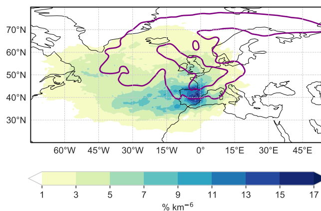
Figure 4. Location of air parcels three days prior to their arrival in the snowfall area over Spain (see text for details). The colour shading represents the climatological origin of near-surface air in late December and early January, and the purple lines ( 1 and 17\% \text{ km}^{-6} ) represent the origin of air associated with the cold spell in late December 2020 and early January 2021.
