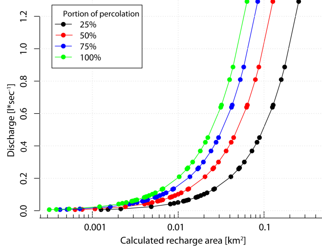
Figure 5. Estimated size of recharge area based on average discharge and annual water input of 643 mm (Pfeiffer et al., 2021). The recharge area size was derived from equation 2 for four different infiltration ratios I_c (25%, 50%, 75% and 100%).
