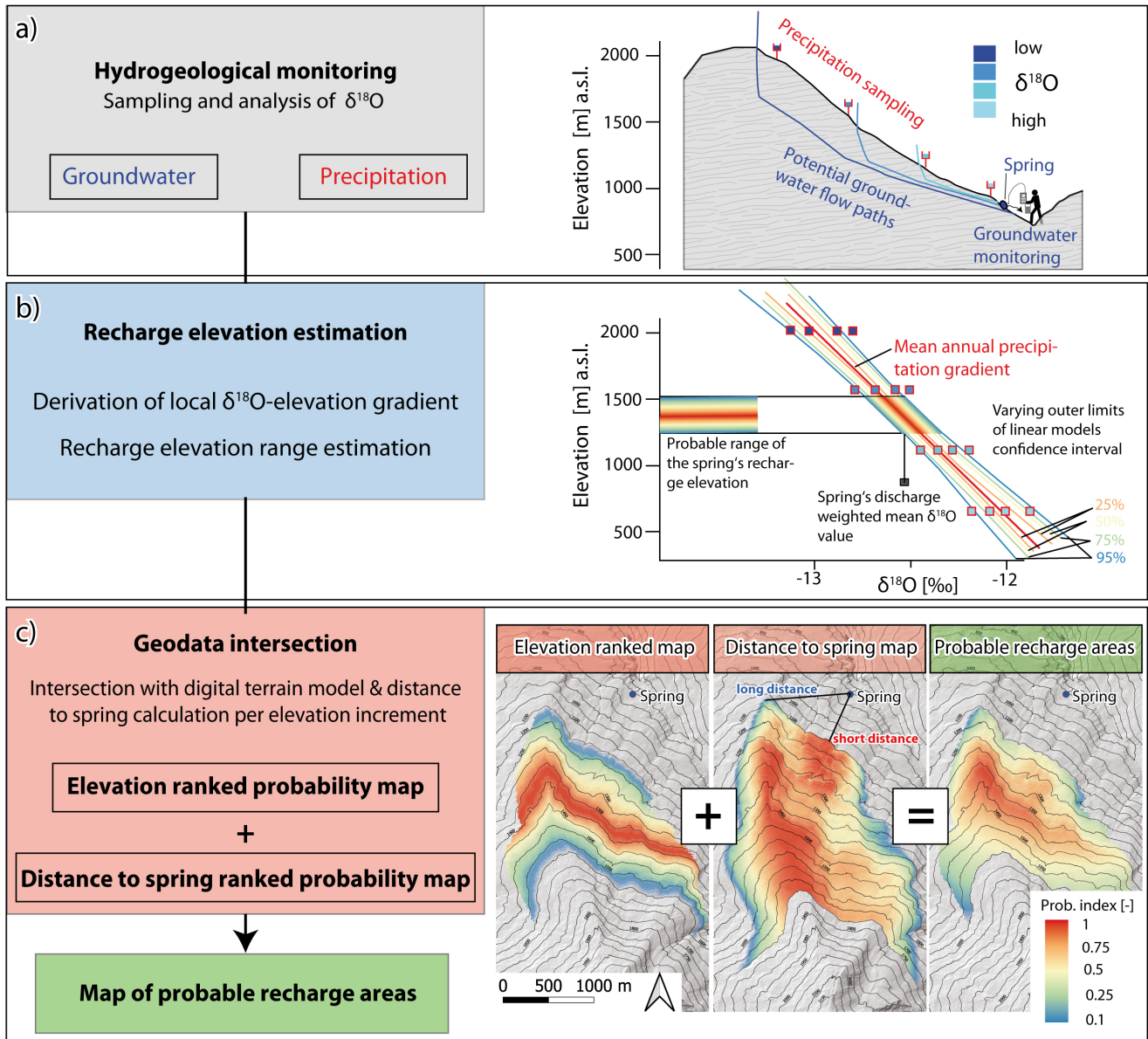
Figure 3. Proposed workflow for deriving maps of probable recharge areas including a) Hydrogeological monitoring b) recharge elevation estimation and c) geodata intersection (DTM source: Federal State of Tyrol).
