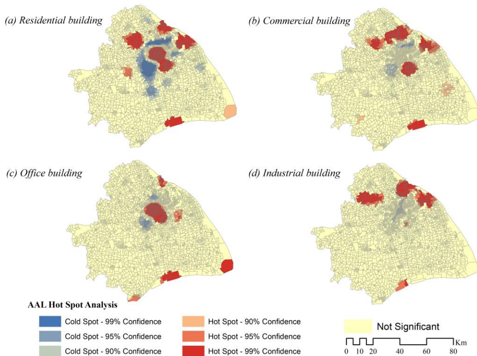
265 Figure 8. The hot spot analysis of the AAL for buildings at sub-district level in Shanghai.
