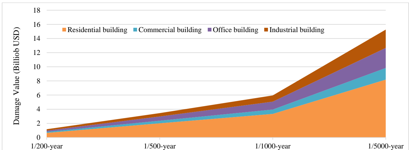
265 Figure 7. Probability-damage curve of extreme flooding for residential, commercial, office, and industrial buildings.
