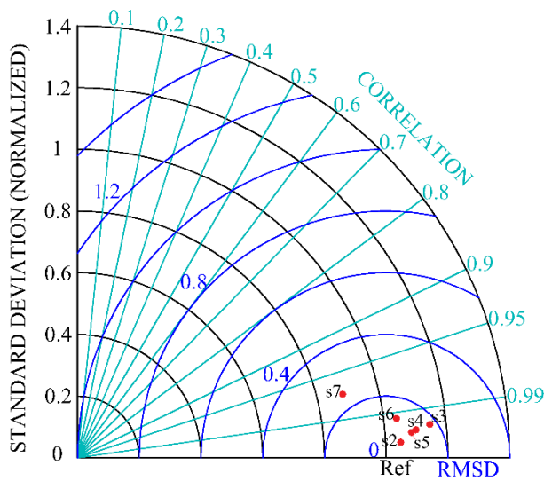
Figure 29: Taylor diagram of hydrodynamic pressures at x = 10 \text{ m} and z = 2.1 \text{ m} , taking as reference the data series of the finest resolution of \Delta p = 0.1 \text{ m} .
