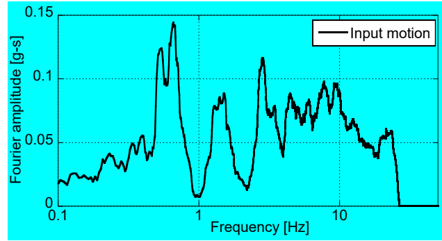
Figure 16: Frequency content of the input ground motion.
