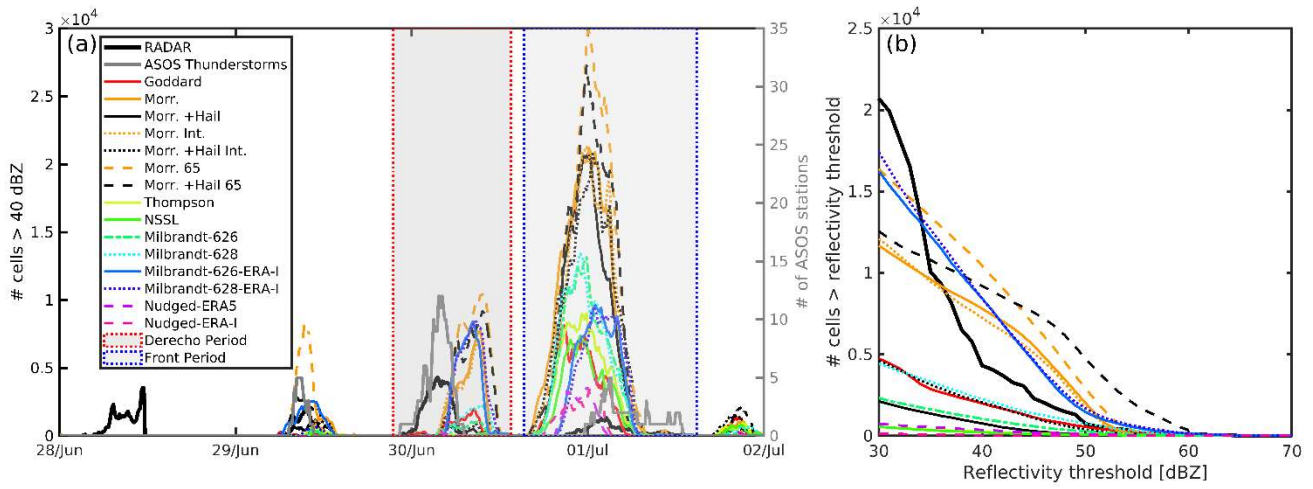
1035 Figure 4: (a) Time series of number of grid cells in domain d03 with composite reflectivity (cREF) > 40 dBZ from RADAR and the 15 WRF ensemble members. The number of the 34 ASOS stations in domain d03 reporting thunderstorms is shown in grey (right axis). The timing of the (Derecho period: 29-Jun-2012 21:30:00 to 30-Jun-2012 13:30:00) and the frontal passage (Front period: 30-Jun-2012 15:20:00 to 01-Jul-2012 14:50:00) are denoted by the grey backgrounds. (b) The number of grid cells in domain d03 where output from each WRF ensemble member or the RADARs exceeded the specified threshold during the time step within the derecho period when the maximum number of grid cells exceeded the threshold. For example, in the RADAR observations there is a single 10-minute period during which approximately 5000 grid cells exhibit a value above 40 dBZ.
