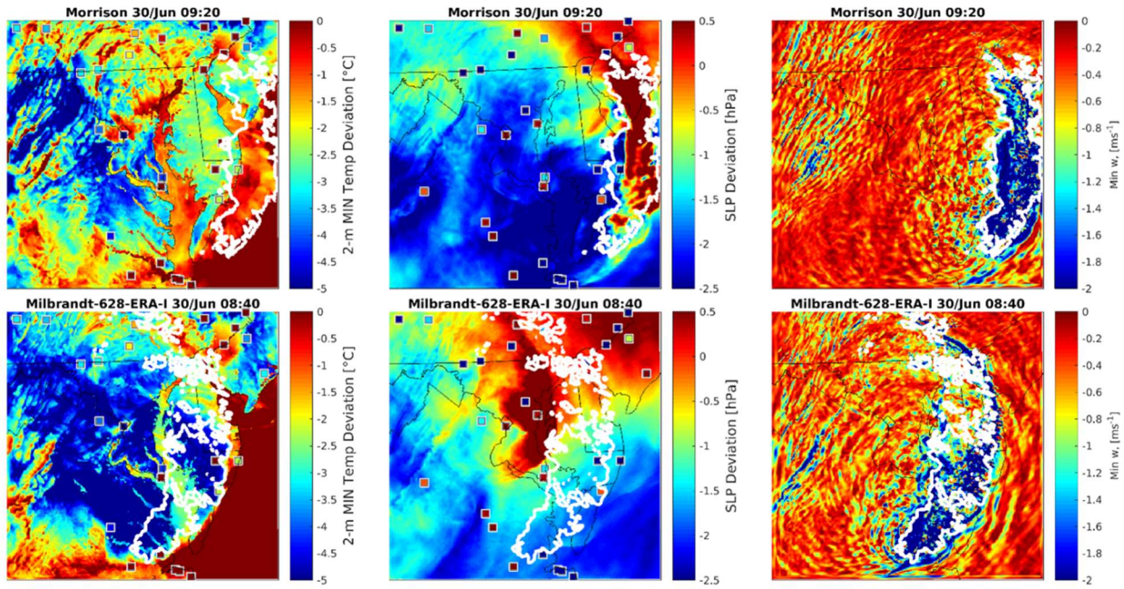
Figure 14: WRF cold pool diagnostics at t_p from two of the model skillful ensemble members: Morrison (upper row) and Milbrandt-628-ERA-I (lower row). The metrics shown are 2 m temperature anomaly (left), sea level pressure anomaly (center) and largest negative velocity (right) for the WRF ensemble members. The title indicates the time step associated with t_p , i.e. when the maximum spatial coverage of cREF > 40 dBZ is simulated. Grid cells with cREF > 40 dB at t_p is outlined by the white contour.
