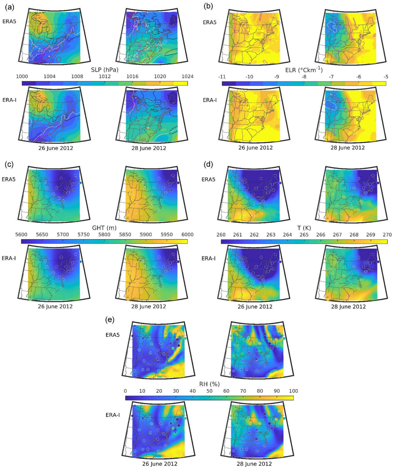
1025 Figure 3: (a) Spatial maps of sea level pressure (colored surface) generated by WRF real from the ERA5 and ERA-Interim reanalysis 1030 products used to provide the model LBC and initial conditions. The black, red, and magenta lines are 2-m temperature of 295 K, 300 K, and 305 K respectively. The white line represents specific humidity at 2-m of 12.5 g/kg. (b) Filled contours of lapse rates (700-500 hPa) with the -9^{\circ}\text{C}/\text{km} highlighted by the white outline. Also shown by the magenta isoline is the area in which the RH increased by 20% over this layer. (c) 500 hPa geopotential height in meters. (d) 500 hPa temperature in Kelvin. (e) 500 hPa relative humidity in %. Plots in (c), (d), and (e) contain rawinsonde observations (filled circles). In all the plots, WRF real output is used from all 3 domains.
