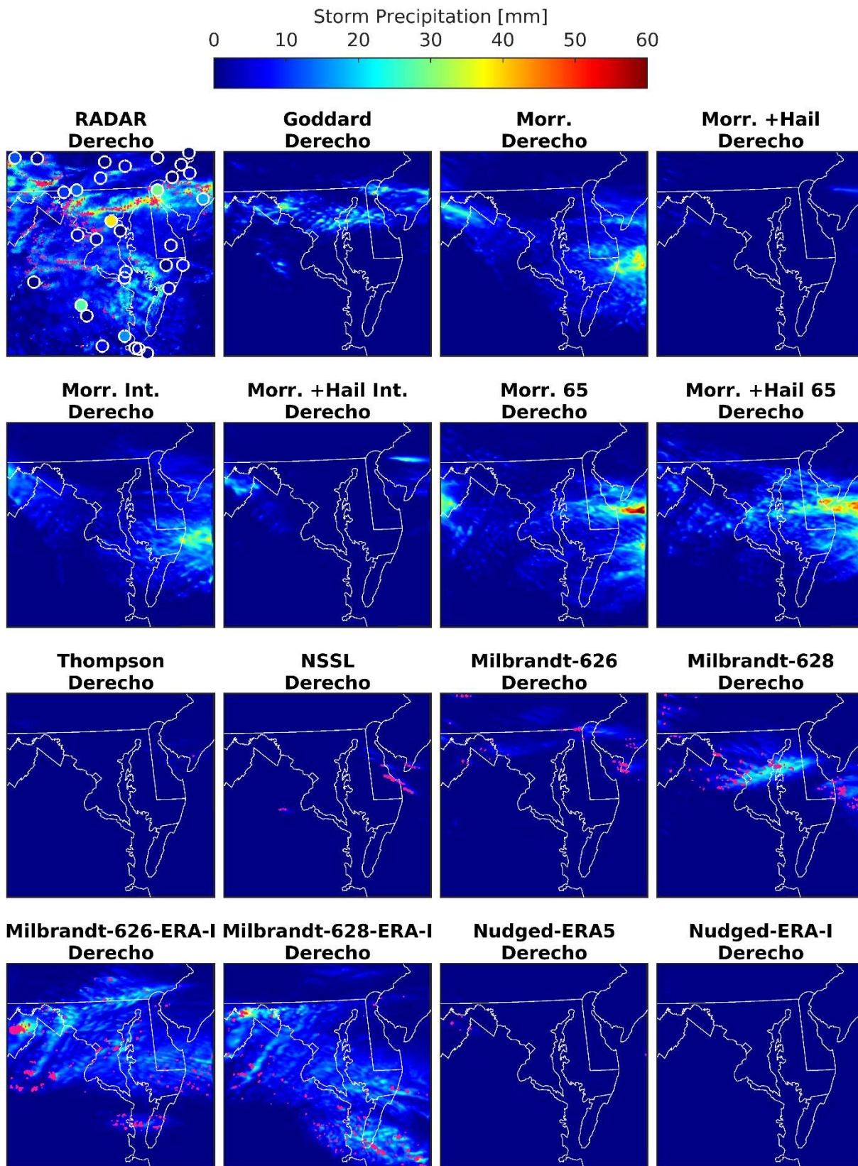
1055 Figure 7: Total accumulated precipitation (mm) from RADAR observations and each WRF ensemble member during the Derecho period. Grid cells with MESH>25mm are marked in magenta.
