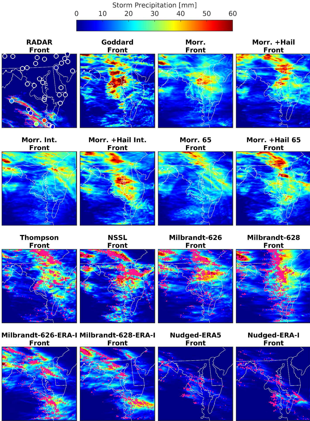
Figure 8: Total accumulated precipitation (mm) from RADAR and each WRF ensemble member during the Front period. Grid cells with MESH>25mm are marked in magenta.
