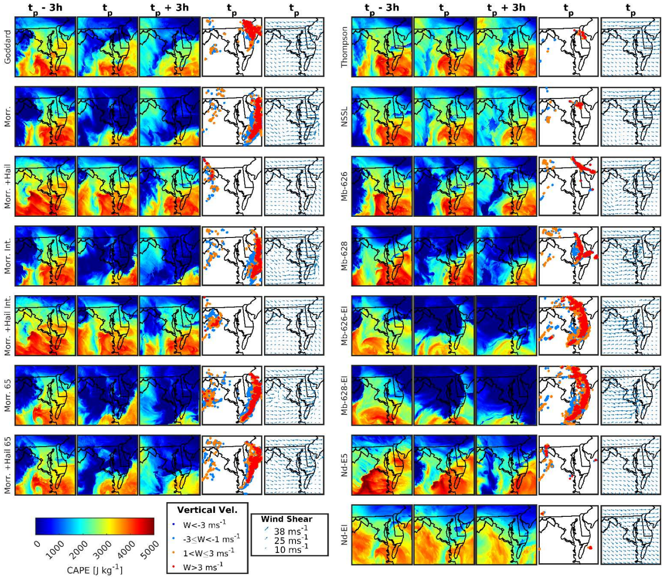
Figure 13: MU-CAPE, vertical velocities, and wind shear within domain d03 for each WRF ensemble member. The left three columns show MU-CAPE for each member at t_p - 3 hours, t_p (i.e. the time of peak spatial extent of cREF > 40 dBZ during the Derecho Period) and t_p + 3 hours. The fourth column shows the vertical wind speed ( W ) at 5000 m a.g.l at t_p . |W| within individual grid cells greatly exceeds 3 \text{ ms}^{-1} (values range from -10 to +10 \text{ ms}^{-1} ) these classes have been subjectively selected to capture the major regions of up and downdrafts. The right column shows the total wind shear between ground and 6000 m ( S_6 , see definition in section 2.3). Larger versions of these maps have been provided in supplementary materials (Figures SM2-4, 5 and 7).
