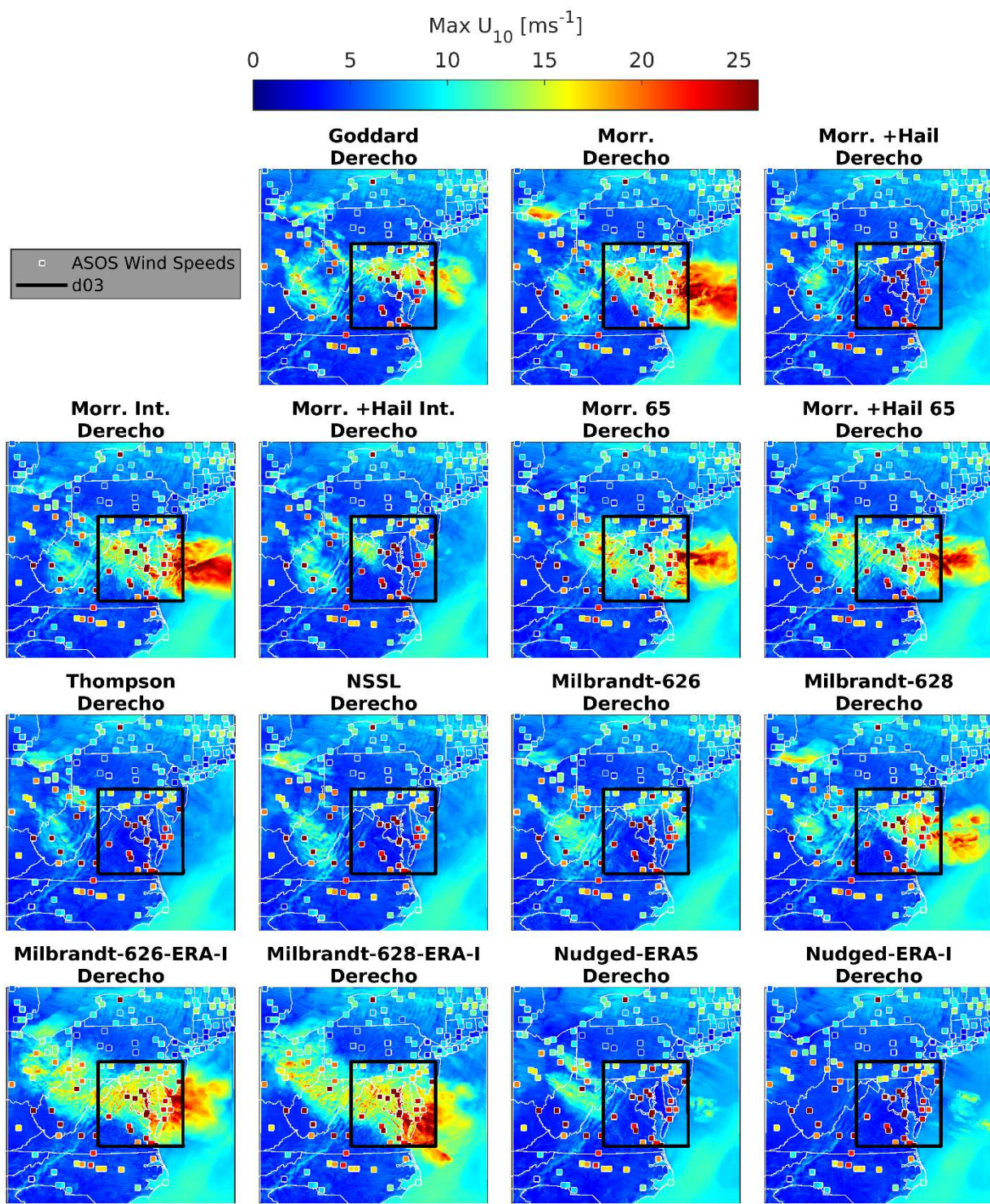
1080 Figure 11: Maximum wind speeds ( \text{ms}^{-1} ) at the model time step of 3.33 sec in d03 (outlined in black) and 10 seconds in d02 for each ensemble member during the Derecho period. Maximum 3-second wind gusts ( \text{ms}^{-1} ) at each ASOS station are shown by the square markers. The colorbar is truncated to aid legibility at the maximum value from any WRF ensemble member. Multiple ASOS stations reported wind gusts above 25.7 \text{ ms}^{-1} .
