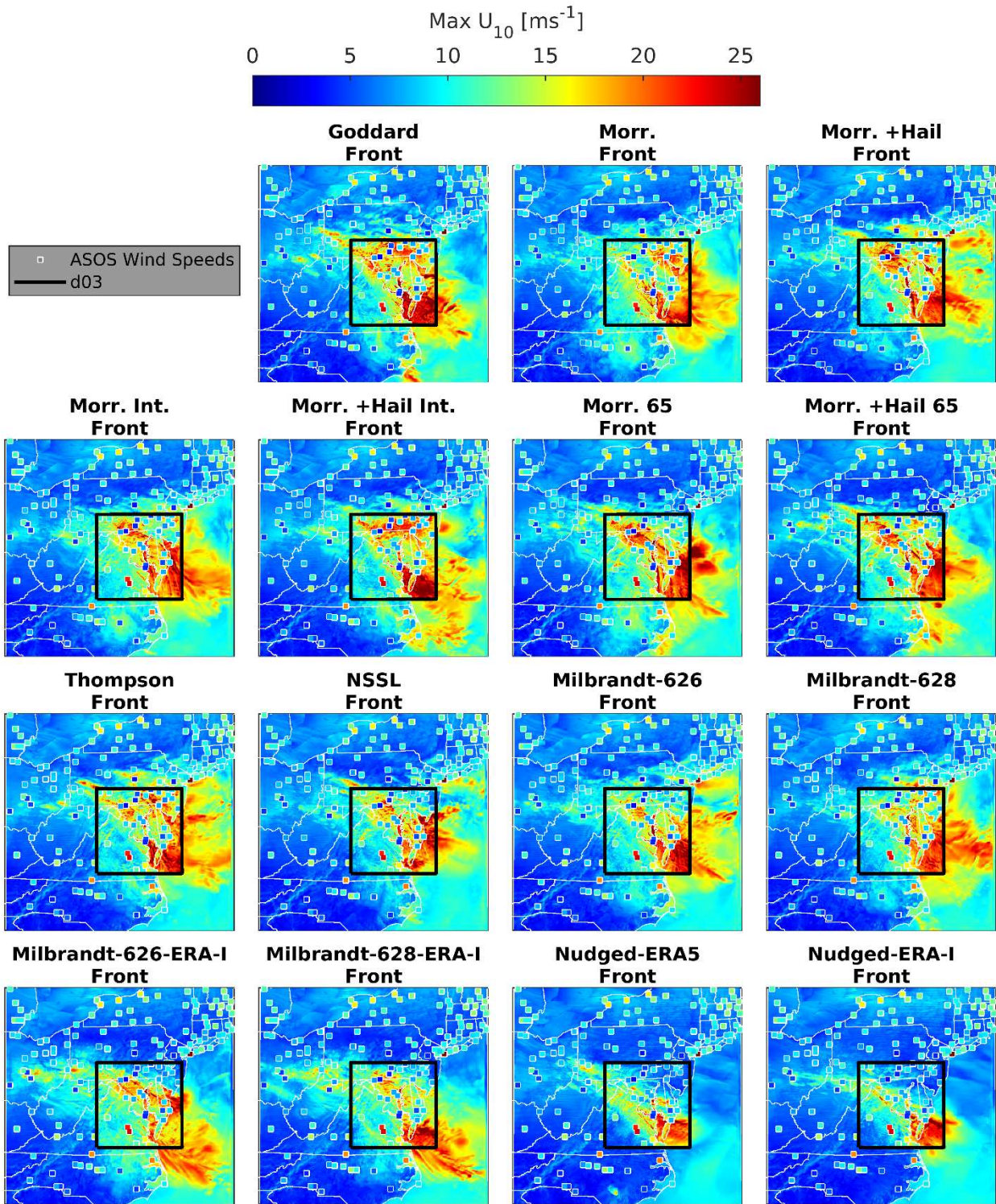
1085 Figure 12: Maximum wind speeds ( \text{ms}^{-1} ) at the model time step of 3.33 sec in d03 (outlined in black) and 10 seconds in d02 for each ensemble member during the Front period. Maximum 3-second wind gusts ( \text{ms}^{-1} ) at each ASOS station are shown by the square markers. The colorbar is as used in Figure 11 to aid comparisons.
