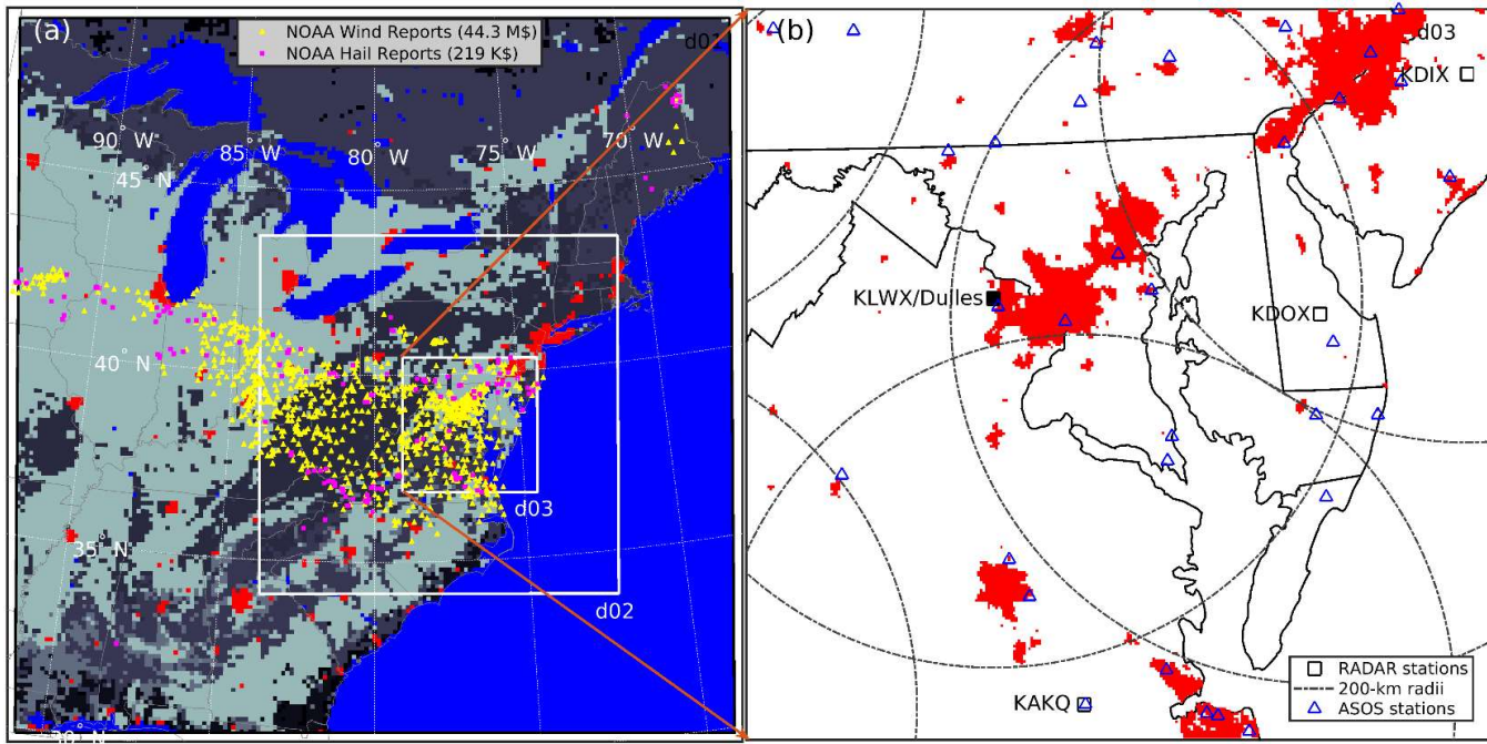
1010 Figure 1: a) Map of the WRF simulation domains; d01, d02, d03 with land use classes shown, where blue indicates water and red, developed areas (shown in both panels), different shades of grey denote different non-urban land use. The yellow markers indicate wind reports in the NOAA Storm Data publication during 29 and 30 June 2012, the magenta denotes reports of hail. The total amount of property damage in the NOAA Storm Data publication from wind and hail within the study area in this two-day period is given in the upper legend of (a) and are 2012$ 44.3 million and 2012$ 291,000 respectively. b) Locations of RADAR (black squares, the black circles 1015 denote the 200 km radii from which data are presented here) and ASOS stations 1 (blue triangles) in d03. Dulles Airport is within 3 km of KLWX and both are denoted by the same filled, black square.
