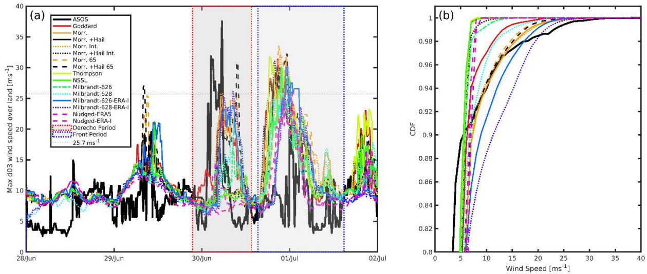
1070 Figure 10: (a) Time series of maximum wind gust in each 10-minute period at any ASOS station and any WRF land grid cell in domain d03, for each ensemble member (see maps in Figures 11 and 12). The timing of the (Derecho period: 29-Jun-2012 21:30:00 to 30-Jun-2012 13:30:00) and the frontal passage (Front period: 30-Jun-2012 15:20:00 to 01-Jul-2012 14:50:00) are denoted by the grey backgrounds. The horizontal grey line denotes a wind speed of 25.7 \text{ ms}^{-1} which is used by the NWS to define a damaging wind gust. (b) Spatiotemporal (every grid cell and all time steps) cumulative density functions (CDFs) of ASOS wind gusts and WRF wind speeds in d03 during the Derecho period. To aid legibility only the upper 20% of values are shown.
