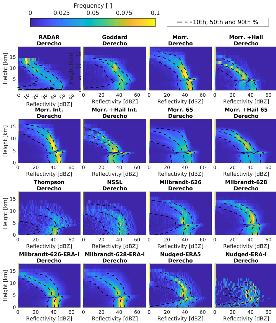
Figure 89: Probability distributions of base reflectivity from RADAR and derived RADAR reflectivity from each WRF ensemble member at each model height at t_p during the Derecho period. The plot shows the frequency with which a given reflectivity is observed at a given height in output for all domain d03 grid cells where cREF > 40 dBZ. Dotted lines show the 10 th , 50 th and 90 th percentile reflectivity at each height.
