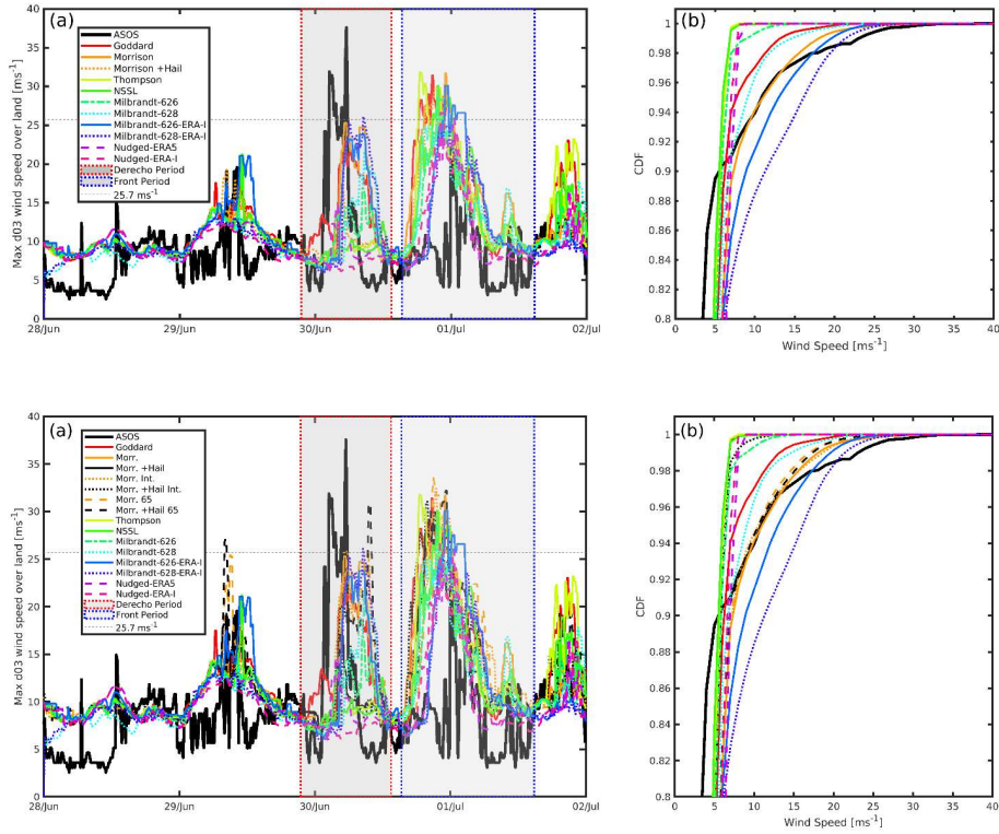
1090 Figure 910: (a) Time series of maximum wind gust in each 10-minute period at any ASOS station and any WRF land grid cell in domain d03, for each ensemble member (see maps in Figures 110 and 121). The timing of the (Derecho period: 29-Jun-2012 21:30:00 to 30-Jun- 2012 13:30:00) and the frontal passage (Front period: 30-Jun-2012 15:20:00 to 01-Jul-2012 14:50:00) are denoted by the grey backgrounds. The horizontal grey line denotes a wind speed of 25.7 ms -1 which is used by the NWS to define a damaging wind gust. (b) 1095 Spatiotemporal (every grid cell and all time steps) cumulative density functions (CDFs) of ASOS wind gusts and WRF wind speeds in d03 during the Derecho period. To aid legibility only the upper 20% of values are shown.
