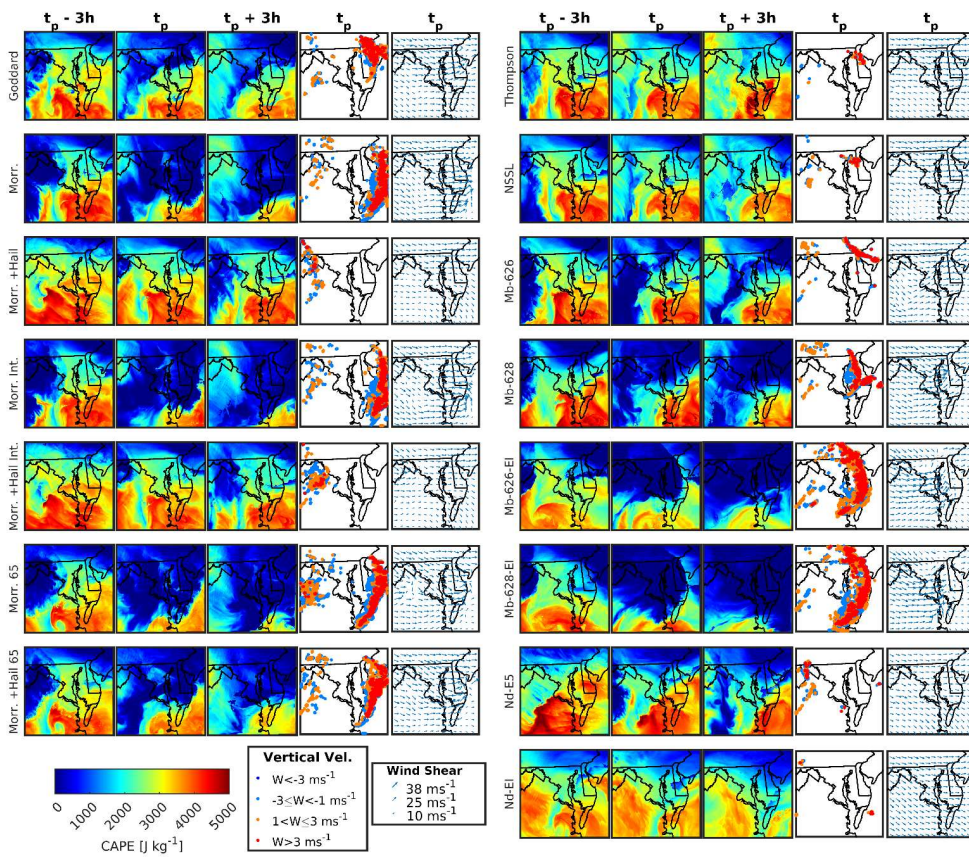
Figure 1335: MU-CAPE, vertical velocities, and wind shear within domain d03 for each WRF ensemble member. The left three columns show MU-CAPE for each member at t_p - 3 hours, t_p (i.e. the time of peak spatial extent of cREF > 40 dBZ during the Derecho Period) and t_p + 3 hours. The fourth column shows the vertical wind speed ( W ) at 5000 m a.g.l at t_p . |W| within individual grid cells greatly exceeds 3 \text{ ms}^{-1} (values range from -10 to +10 \text{ ms}^{-1} ) these classes have been subjectively selected to capture the major regions of up and downdrafts. The right column shows the total wind shear between ground and 6000 m ( S_6 , see definition in section 2.3). Larger versions of these maps have been provided in supplementary materials (Figures SM2-4, 56 and 7).
