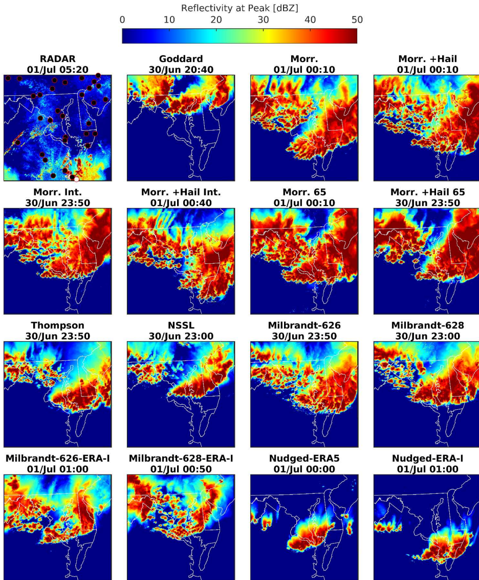
Figure 56: Composite reflectivity (cREF) in domain d03 at t_p (the time when values from the maximum number of grid cells exceeded 40 dBZ) during the Front period from RADAR and each WRF ensemble member (times are noted in panel titles). The RADAR panel includes markers showing the presence (white) and absence (black) of thunderstorm reports from ASOS stations in domain d03 in the hour surrounding 05:20 UTC 1 July 2012.
