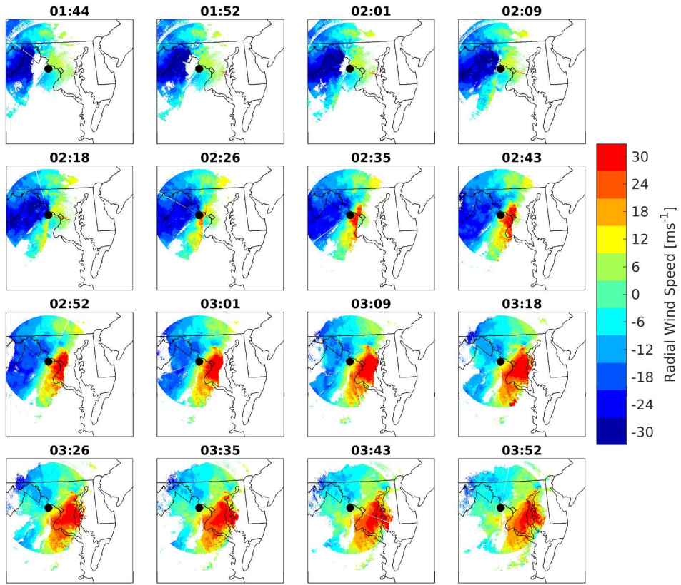
1040 | Figure 2: Radial wind speeds from the NWS RADAR deployed at Sterling, VA (station code KLWX, shown as a black circle) the closest RADAR station to Washington Dulles airport, sampled for every second scan from the lowest elevation angle ( 0.5^\circ ) for about a 2-hour period surrounding the period of highest recorded wind speeds at the airport.
