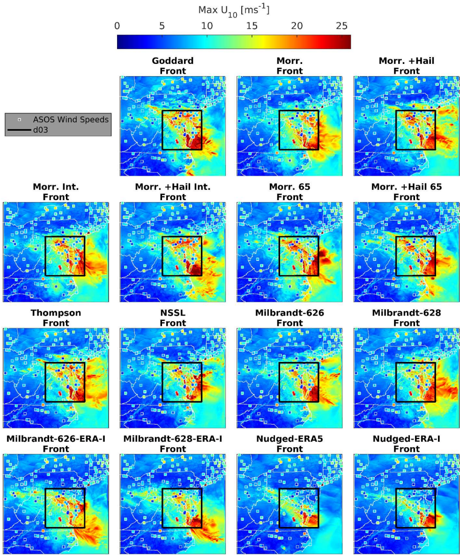
Figure 4412: Maximum wind speeds ( \text{ms}^{-1} ) at the model time step of 3.33 sec in d03 (outlined in black) and 10 seconds in d02 for each ensemble member during the Front period. Maximum 3-second wind gusts ( \text{ms}^{-1} ) at each ASOS station are shown by the square markers. The colorbar is as used in Figure 40-11 to aid comparisons.
