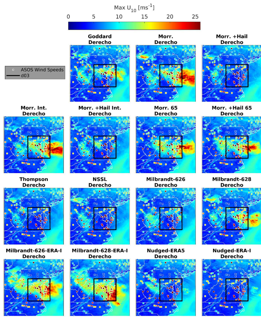
100 Figure 1011: Maximum wind speeds ( \text{ms}^{-1} ) at the model time step of 3.33 sec in d03 (outlined in black) and 10 seconds in d02 for each ensemble member during the Derecho period. Maximum 3-second wind gusts ( \text{ms}^{-1} ) at each ASOS station are shown by the square markers. The colorbar is truncated to aid legibility at the maximum value from any WRF ensemble member. Multiple ASOS stations reported wind gusts above 25.7 \text{ ms}^{-1} .
