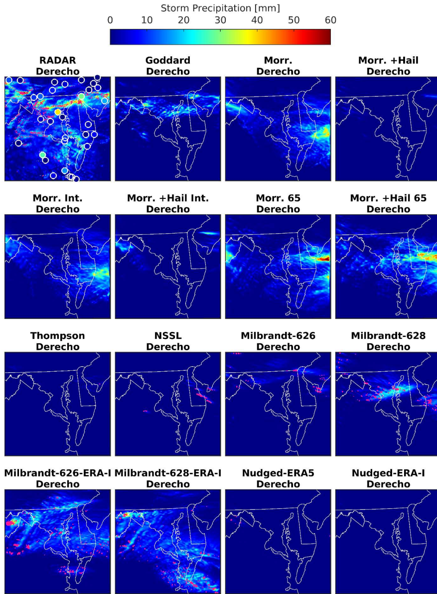
Figure 67: Total accumulated precipitation (mm) from RADAR observations and each WRF ensemble member during the Derecho period. Grid cells with MESH>25mm are marked in magenta.
