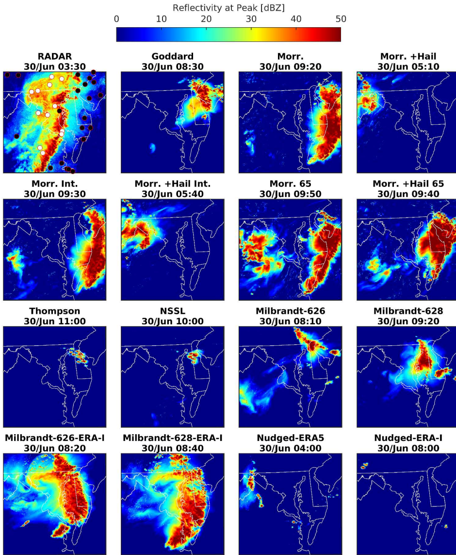
Figure 45: Composite reflectivity (cREF) in domain d03 at t_p (the time when values from the maximum number of grid cells exceeded 40 dBZ) during the Derecho period from RADAR and each WRF ensemble member (times are noted in panel titles). The RADAR panel includes markers showing the presence (white) and absence (black) of thunderstorm reports from ASOS stations in domain d03 in the hour surrounding 03:30 UTC 30 June 2012.
