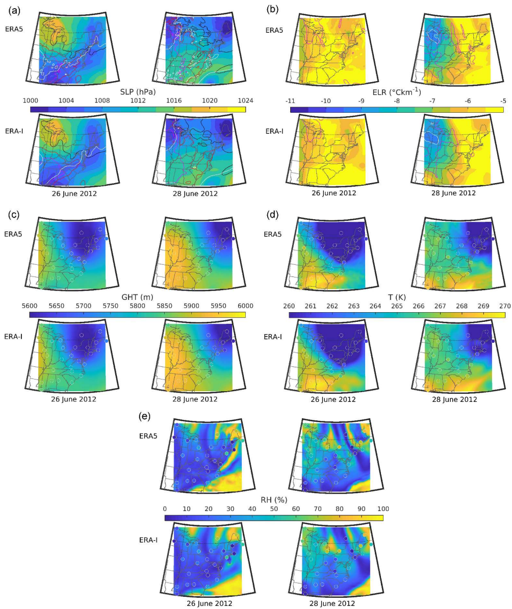
110 Figure 12: (a) Spatial maps of sea level pressure (colored surface) generated by WRF-real from the ERA5 and ERA-Interim reanalysis products used to initialize the model LBC and initial conditions. The black, red, and magenta lines are 2-m temperature of 295 K, 300 K, and 305 K respectively. The white line represents specific humidity at 2-m of 12.5 g/kg. (b) Filled contours of lapse rates (700-500 hPa) with the -9^{\circ}\text{C}/\text{km} highlighted by the white outline. Also shown by the magenta isoline is the area in which the RH increased by 20% over this layer. (c) 500 hPa geopotential height in meters. (d) 500 hPa temperature in Kelvin. (e) 500 hPa relative humidity in %. Plots in (c), 115 (d), and (e) contain rawinsonde observations (filled circles). In all the plots, WRF-real output is used from all 3 domains.
