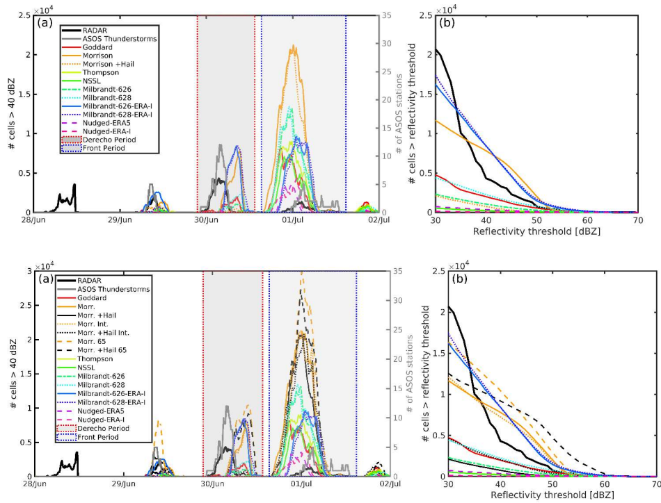
Figure 34: (a) Time series of number of grid cells in domain d03 with composite reflectivity (cREF) > 40 dBZ from RADAR and the 15 WRF ensemble members. The number of the 34 ASOS stations in domain d03 reporting thunderstorms is shown in grey (right axis). The timing of the (Derecho period: 29-Jun-2012 21:30:00 to 30-Jun-2012 13:30:00) and the frontal passage (Front period: 30-Jun-2012 15:20:00 to 01-Jul-2012 14:50:00) are denoted by the grey backgrounds. (b) The number of grid cells in domain d03 where output from each WRF ensemble member or the RADARs exceeded the specified threshold during the time step within the derecho period when the maximum number of grid cells exceeded the threshold. For example, in the RADAR observations there is a single 10-minute period during which approximately 5000 grid cells exhibit a value above 40 dBZ.
