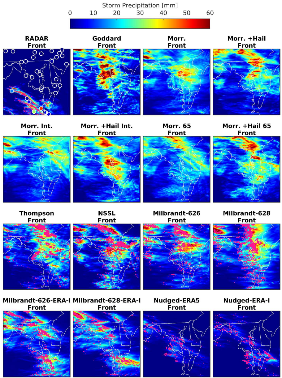
Figure 78: Total accumulated precipitation (mm) from RADAR and each WRF ensemble member during the Front period. Grid cells with MESH>25mm are marked in magenta.
