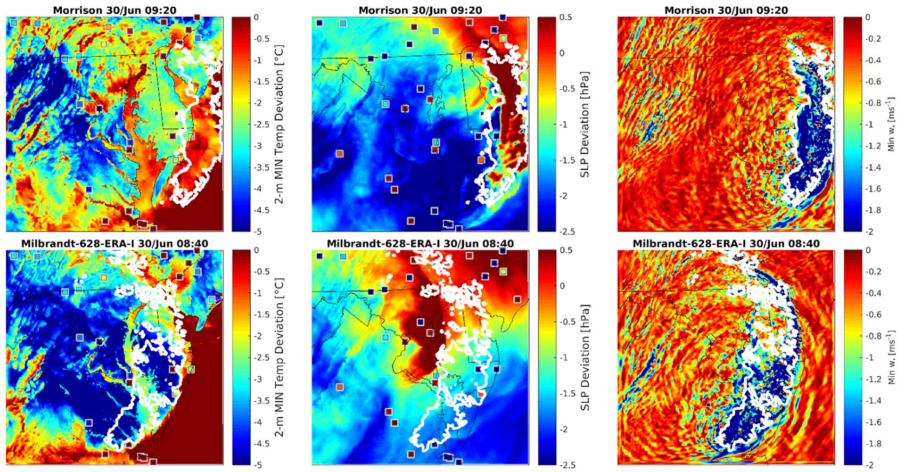
145 Figure 1446: WRF cold pool diagnostics at t_p from two of the model skillful ensemble members: Morrison (upper row) and Milbrandt-628-ERA-I (lower row). The metrics shown are 2 m temperature anomaly (left), sea level pressure anomaly (center) and largest negative velocity (right) for the WRF ensemble members. The title indicates the time step associated with t_p , i.e. when the maximum spatial coverage of cREF > 40 dBZ is simulated. Grid cells with cREF > 40 dB at t_p is outlined by the white contour.
