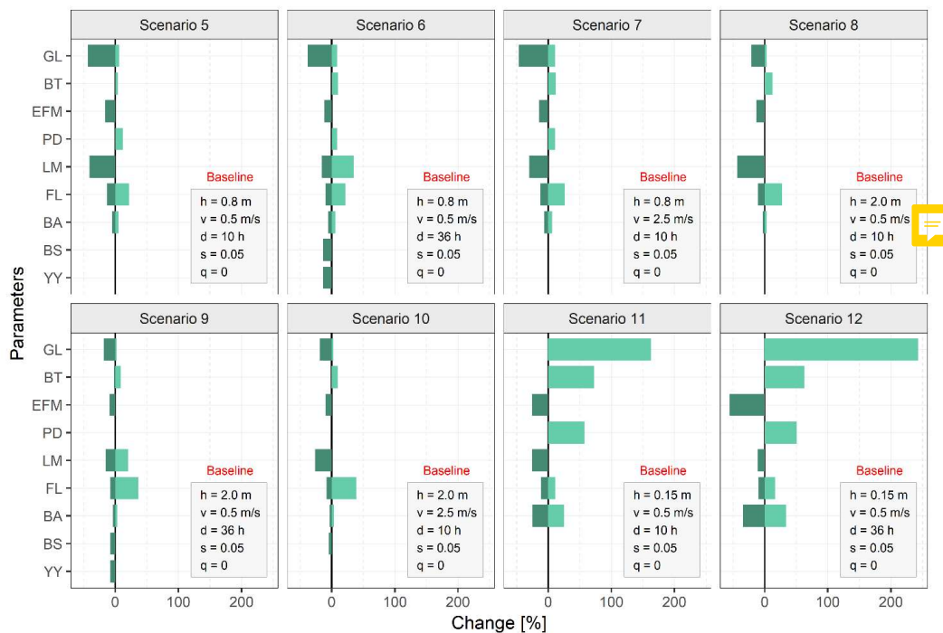
365 Figure 10: Results of the sensitivity analysis for the building parameters (dark green: negative change; light green: positive change).
