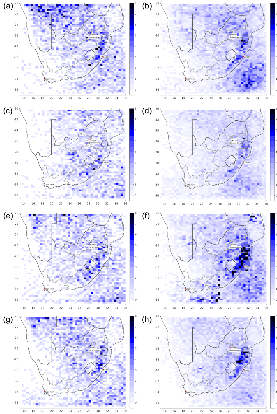
Figure 14. Spatial patterns of annual event distribution for single years (left) and the stochastic event set (right) for the years (a, b) 2005/06, (c, d) 2006/07, (e, f) 2007/08, and (g, h) 2008/09.
