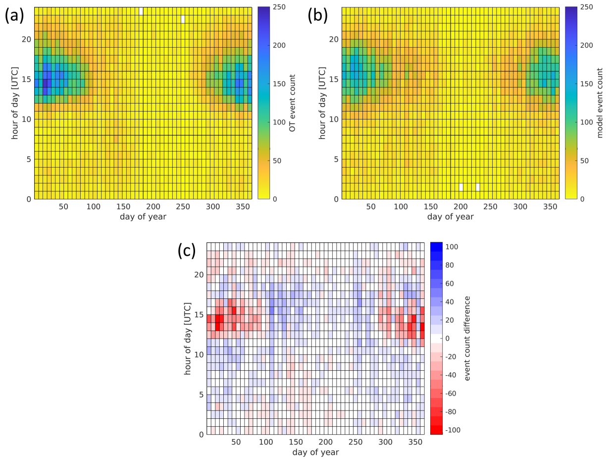
Figure 9. Distribution of potential hail events in time of day and day of year: (a) historic events 2005–2018; (b) stochastic model events; and (c) difference between the two for the events shown in Fig. 8. Days of the year are counted from January 1st. The grid shown in all Figs. represents 1 hour and 7 days.
