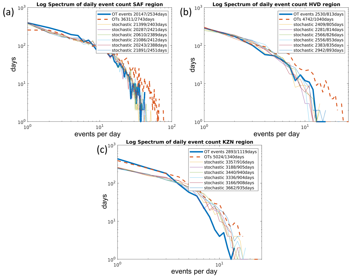
Figure 16. As Fig. 15, but comparing subsets of the stochastic event set to the historic OT event set (as well as the set containing events lasting only one time step) for each region. (a) South Africa, (b) Highveld, (c) KwaZulu-Natal. Numbers indicate the total count and total number of days on which these occurred for each set.
