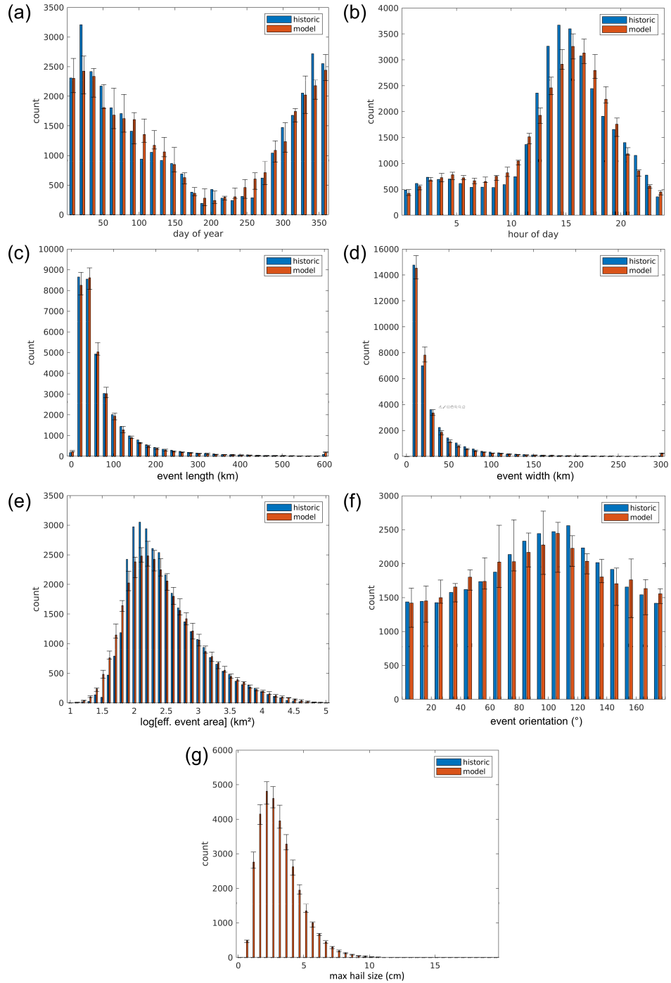
Figure 10. Distributions for properties of historic and stochastic events. With modeled events, (error) bars indicate the median (spread) among 7 independent samples of 14 years' length. Each set of bars represents 14 days, 1 hour, 20 km in length, 10 km in width, 0.1 on the log scale of part (e) and 10^\circ in orientation. Since hail severity information is essentially unknown for the historic events, blue bars are missing in (g).
