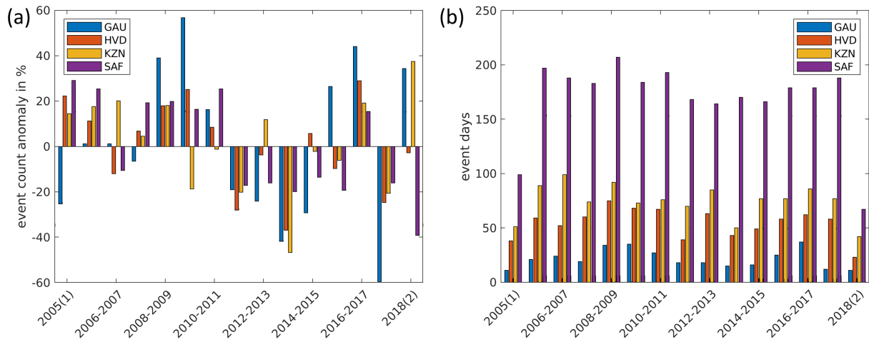
Figure 13. Time series of event count anomaly: (a) deviation of the annual sum from the 14-year mean) and (b) event days per year (July–June) for regions Gauteng (GAU, regional annual mean event count 35), Highveld (HVD, 152), KwaZulu-Natal (KZN, 181) and South Africa (SAF, 1259). The July–June period is considered more appropriate as the Austral summer season is not split among years. For the 2004/2005 period, only events in 2005 are covered; likewise 2018/2019 covers only the last 6 months of 2018. When computing the event count anomalies for these years, the overall repartition of events to half years was taken into account.
