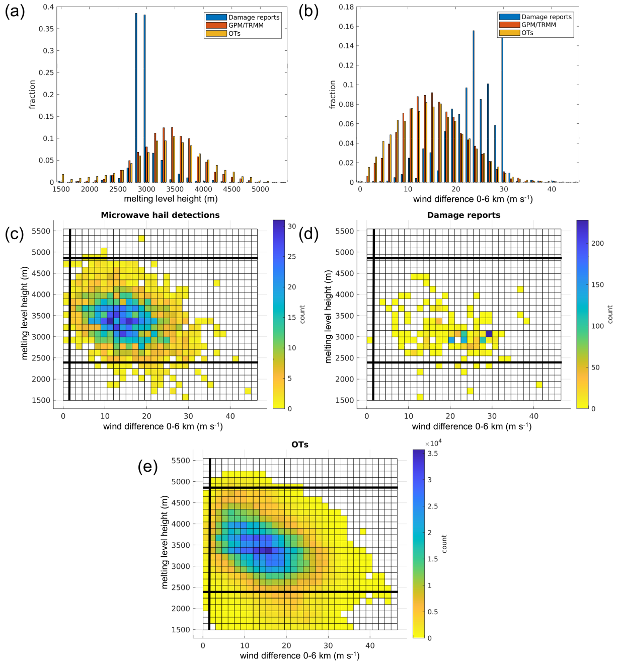
Figure 5. Distribution of ERA-5 0–6 km wind difference and melting level height in hail claims (1984–2017), passive microwave detections (1998–2019), and OTs (2005–2018) for South Africa and Lesotho. Top row: probability distribution; Bottom row: bi-variate histogram for 0–6 km wind difference and freezing level (bold lines indicate the selected filter thresholds; see text for further details). Only situations with positive CAPE in ERA-5 were used for these computations.
