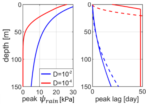
595 Figure A1: Maximum rainfall response in function of depth and its time lag for the synthetic recharge (Fig. 2). The time lag caps at 48 days, maximum duration between the end of the recharge (2 days) and the length of the time vector (50 days). Dashed lines represent theoretical characteristic response times t_c = z^2/D , in comparison to the times of maximum response computed from the model.
