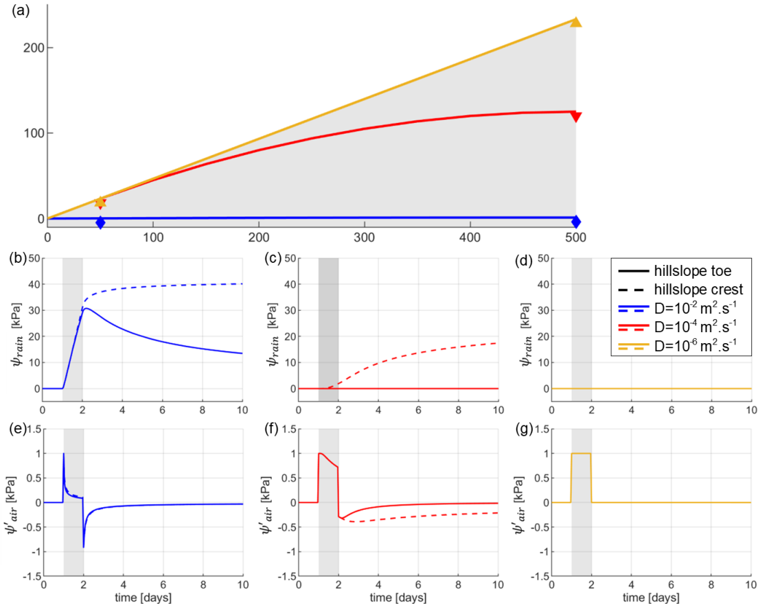
255 Figure 4: Initial state of the water table in the hillslope (a) after a static recharge of 10^{-9} m s^{-1} and investigated points at the crest and toe of the hillslope. Temporal evolution of \psi_{rain} (b), (c) & (d) and \psi'_{air} (e), (f) & (g) in response to the synthetic forcing (Fig. 2), at several diffusivities. Solid lines represent atmospheric and rainfall effects at the toe of the hillslope, at x = 50 m , and dashed lines the effect at the crest of the hillslope at x = 500 m .
