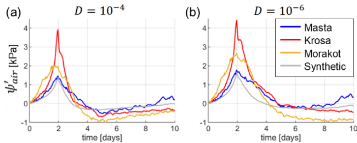
600 Figure A2: Atmospheric induced pore pressures \psi'_{air} for each typhoon event in the finite hillslope model, 5m under the topography (a) at a diffusivity of 10^{-4} m^2 s^{-1} , and (b) at a diffusivity of 10^{-6} m^2 s^{-1} . At these diffusivities, the hillslope is fully saturated from its initial state. Therefore, no rainfall effects are associated with the events, and \psi'_{air} is the same at the toe and the crest of the hillslope.
