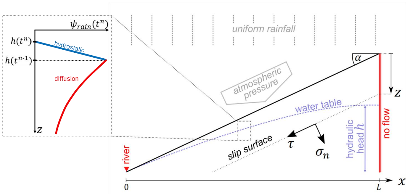
110 Figure 1: Geometry of the considered hillslope. The water table (in blue) forms a quadratic surface between the two boundaries conditions (in red). The stability is evaluated with a Mohr-Coulomb criterion along a slope-parallel slip. The atmospheric pressure and rainfall infiltration are applied uniformly along the slope. The zoomed-in section shows the implementation of the diffusion of pore pressure due to the raise of water table between two consecutive timesteps.
