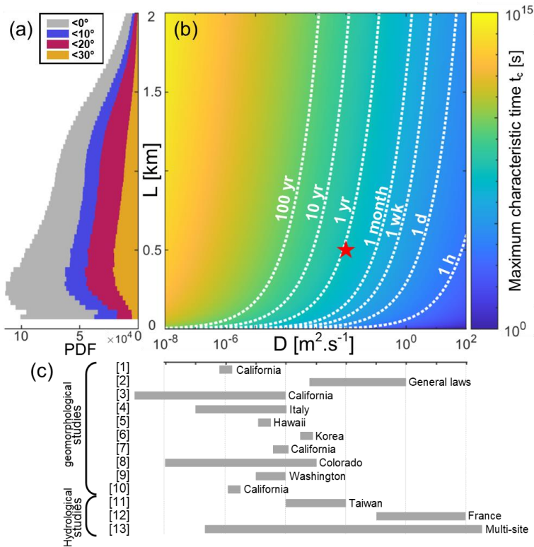
550 Figure 8: Maximum characteristic timescale of hillslopes response depending on diffusivity D and hillslope length L . The histogram (a) shows the repartition of hillslopes lengths in Taiwan, extracted from a 30 \times 30 m DEM. The maximum characteristic hillslope response time L^2/D is presented in (b), with the point corresponding to the values used in this study highlighted. Values of diffusivity found in literature are displayed in (c). Sources from the diffusivity graph (c) are: [1] (Iverson, 2000); [2](Goren and Aharonov, 2007); [3](Handwerger et al., 2013); [4](Berti and Simoni, 2012); [5](Reid, 1994); [6](Kim et al., 2010); [7](Hu et al., 2019); [8](Schulz 555 et al., 2009); [9](Baum et al., 2010); [10](Finnegan et al., 2021); [11](Chien-Yuan et al., 2005); [12](Jiménez-Martínez et al., 2013); [13](Pacheco, 2013). Hillslope length in Taiwan is measured by considering the nearest hydrological distance between crests and rivers, considering that the transition between rivers and hillslope occurs at 0.9 \text{ km}^2 .
