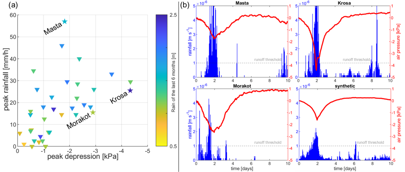
310 Figure 5: (a) Typhoons over Taiwan sorted in function of their maximum rainfall intensity and atmospheric pressure drop. The hydrological context is represented by the colorscale, showing the cumulated rainfall over the 6 months prior the event. (b) Timeseries of rainfall and atmospheric pressure changes of the 3 typhoons and the synthetic event created from the average of every typhoon.
