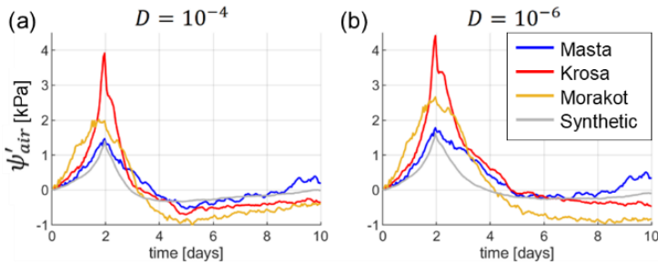
600 Figure A2: Atmospheric induced pore pressures \psi'_{air} for each typhoon event in the finite hillslope model, 5m under the topography (a) at a diffusivity of 10^{-4} \text{ m}^2 \text{ s}^{-1} , and (b) at a diffusivity of 10^{-6} \text{ m}^2 \text{ s}^{-1} . At these diffusivities, the hillslope is fully saturated from its initial state. Therefore, no rainfall effects are associated with the events, and \psi'_{air} is the same at the toe and the crest of the hillslope.
