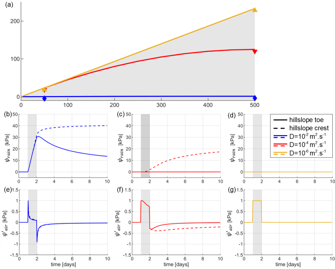
255 Figure 4: Initial state of the water table in the hillslope (a) after a static recharge of 10^{-9} \text{ m s}^{-1} and investigated points at the crest and toe of the hillslope. Temporal evolution of \psi_{rain} (b), (c) & (d) and \psi'_{air} (e), (f) & (g) in response to the synthetic forcing (Fig. 2), at several diffusivities. Solid lines represent atmospheric and rainfall effects at the toe of the hillslope, at x = 50 \text{ m} , and dashed lines the effect at the crest of the hillslope at x = 500 \text{ m} .
