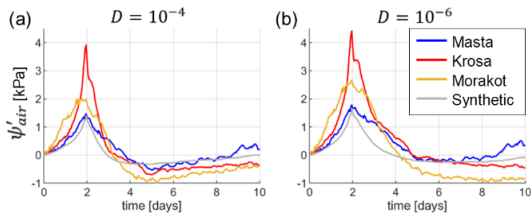
Figure A2: Atmospheric induced pore pressures \psi'_{air} for each typhoon event in the finite hillslope model, 5m under the topography (a) at a diffusivity of 10^{-4} m^2 s^{-1} , and (b) at a diffusivity of 10^{-6} m^2 s^{-1} . At these diffusivities, the hillslope is fully saturated from its initial state. Therefore, no rainfall effects are associated with the events, and \psi'_{air} is the same at the toe and the crest of the hillslope.
