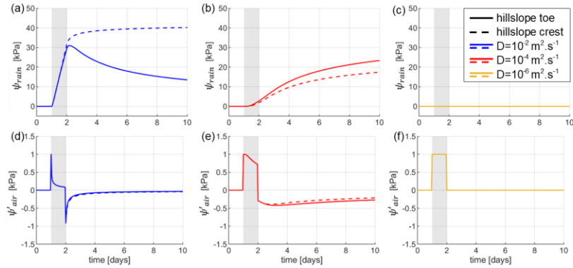
245 Figure 3: Temporal evolution of \psi_{rain} (a), (b) & (c) and \psi'_{air} (d), (e) & (f) in response to the synthetic forcing (Fig. 2), at several diffusivities. Solid lines represent atmospheric and rainfall effects at the toe of the hillslope, at x = 50 m , and dashed lines the effect at the crest of the hillslope at x = 500 m . Note the difference of scale on the y-axis for a, b and c compared to d, e and f.
