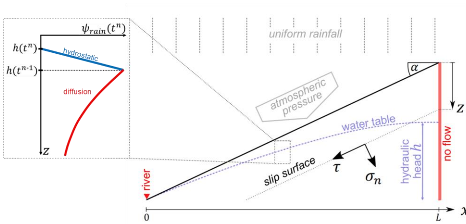
Figure 1: Geometry of the considered hillslope. The water table (in blue) forms a quadratic surface between the two boundary conditions (in red). The stability is evaluated with a Mohr-Coulomb criterion along a slope-parallel slip. The atmospheric pressure and rainfall infiltration are applied uniformly along the slope. The zoomed-in section shows the implementation of the diffusion of pore pressure due to the raise of water table between two consecutive timesteps.
