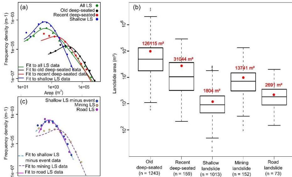
465 Figure 5: Landslide (LS) area characteristics. (a, c) Landslide frequency-area distributions for each landslide category. (b) Boxplots showing the distribution of landslide area for each landslide category. Boxplots show the lower and upper quartiles and median. The whiskers of each box represent 1.5 times the interquartile range. The average area of the landslides (red dots) is provided for each boxplot and the outliers beyond whiskers are shown as dots. The number of landslides in each category is shown in brackets.
