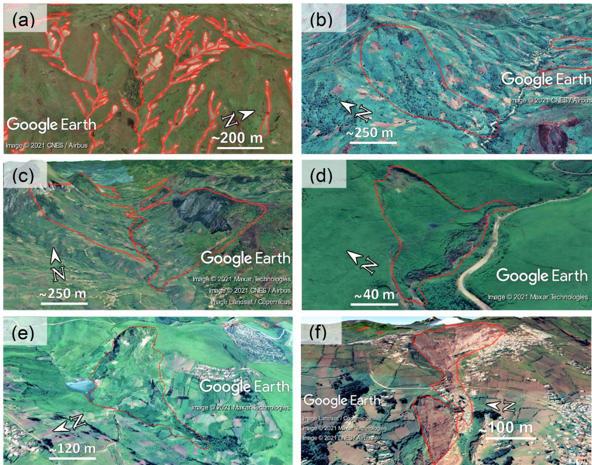
Figure 4: Examples of landslide types (according to Varnes' new classification – Hungr et al., 2014). (a) Cluster of recent debris avalanches and debris flows triggered during an intense rainfall event (25/10/2014) in the vicinity of Kalehe (-2.041°S, 28.874°E); the image illustrates a part of the landslides clustered event 2 shown on Fig. 3a). The source areas of these shallow landslides are identified. (b) Old earthflow (-2.053°S, 28.660°E). (c) Old rock slides/rock avalanches/ with path-dependent rockfalls (-2.007°S, 28.708°E). (d) Recent deep-seated rotational slide that occurred in 2002 (-1.530°S, 28.708°E). (e) Recent deep planar slide that occurred in 1994 and created a dammed lake (-1.521°S, 28.977°E). (f) Recent slides, flows and avalanches associated with mining activities that occurred from 2013 onwards (-1.563°S, 28.885°E).
