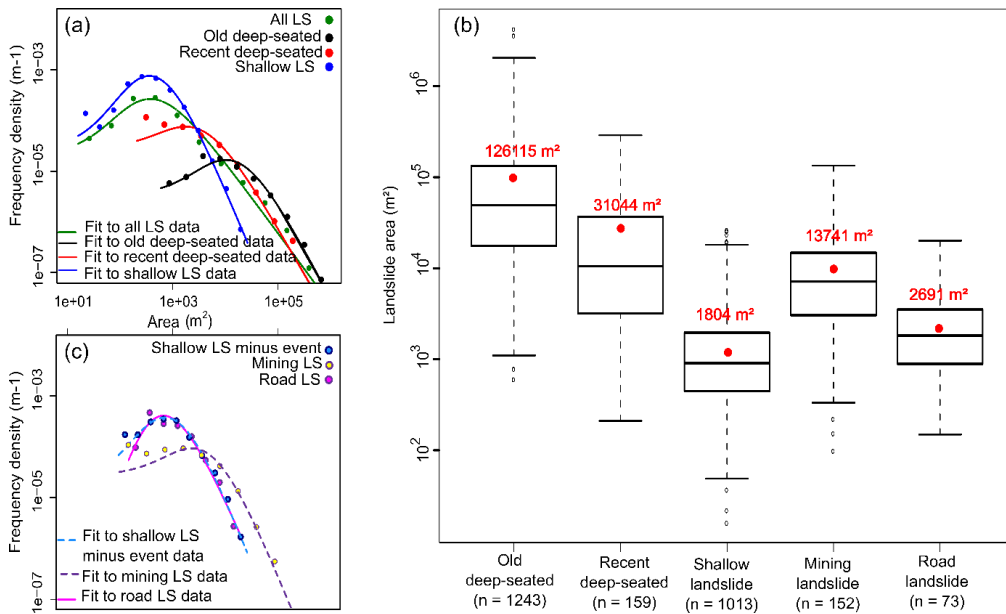
Figure 5: Landslide (LS) area characteristics. (a, c) Landslide frequency-area distributions for each landslide types. (b) Boxplots showing the distribution of landslide area for each landslide type. Boxplots show the lower and upper quartiles and median. The whiskers of each box represent 1.5 times the interquartile range. The average area of the landslides (red dots) is provided for each boxplot and the outliers beyond whiskers are shown as dots. The number of landslides in each class is shown in brackets.
