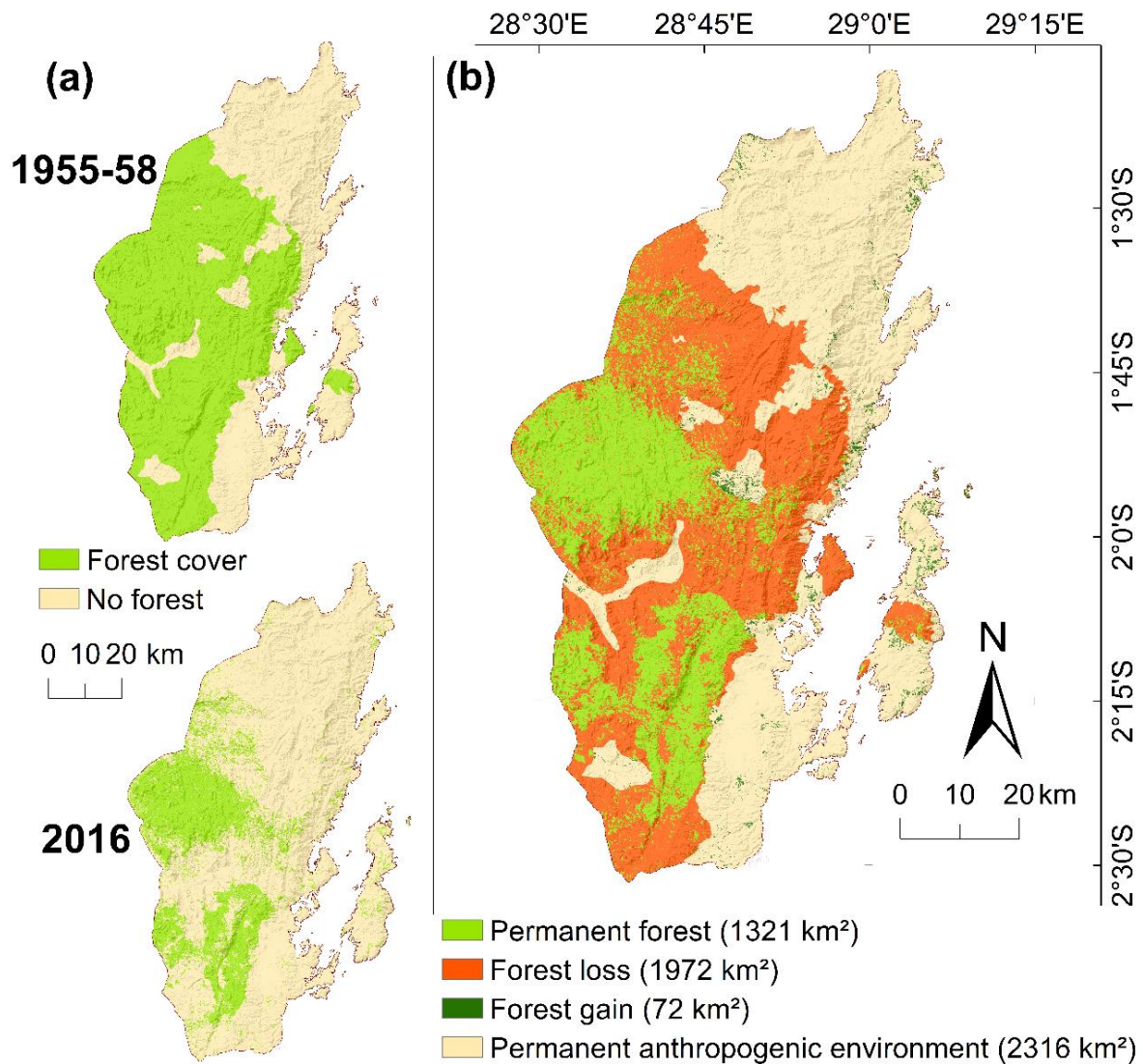
220 Figure 2: Forest cover dynamics over the last 60 years. (a) Forest cover in 1955-58 and 2016; (b) Areas of forest cover change between 1955-58 and 2016. Details for the images used in this figure are in Table 1.
