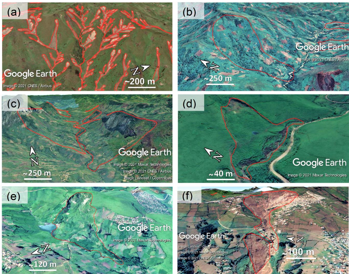
400 Figure 4: Examples of landslide types (according to Varnes' new classification – Hungr et al., 2014). (a) Cluster of recent debris avalanches, flowslides and debris flows triggered during an intense rainfall event (25/10/2014) in the vicinity of Kalehe (-2.041°S, 28.874°E). The landslide source areas are identified. (b) Old earthflow (-2.053°S, 28.660°E). (c) Old rock slides/rock avalanches/ with path-dependent rock falls (-2.007°S, 28.708°E). (d) Recent deep-seated rotational slide that occurred in 2002 (-1.530°S, 28.708°E). (e) Recent deep planar slide that occurred in 1994 and created a dammed lake (-1.521°S, 28.977°E). (f) Recent slides, flows and avalanches associated with mining activities that occurred from 2013 onwards (-1.563°S, 28.885°E). 405
