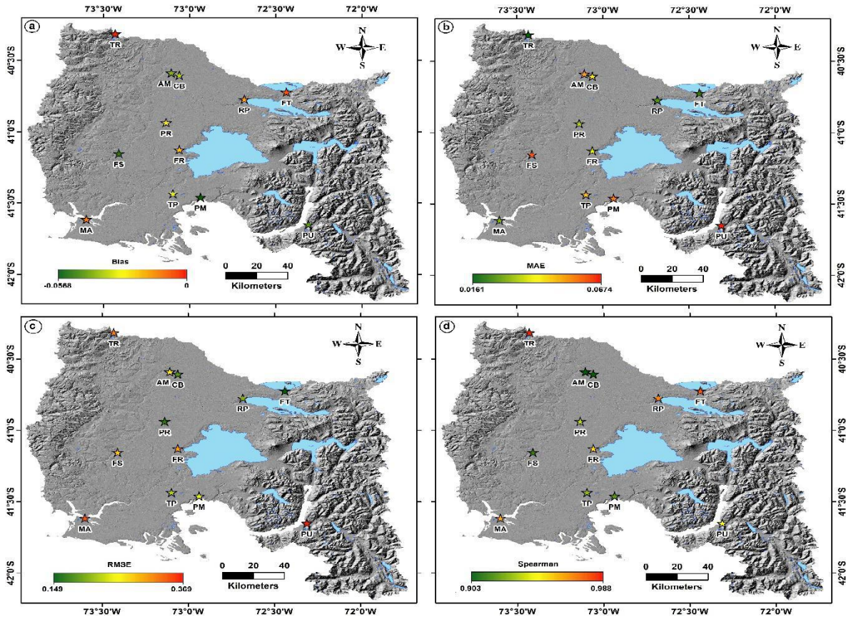
180 Figure 4 Spatial distribution of model corrected at weather stations using best results (PP_M4a). a) BIAS of the simulation in comparison with stations; b) MAE of the simulation in comparison with stations; c) RMSE of the simulation in comparison with stations; d) Spearman of the simulation in comparison with stations. Hillshade based on SRTM data.
