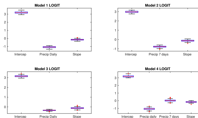
Figure 5. Distribution of estimators for each model with Logit distribution.
