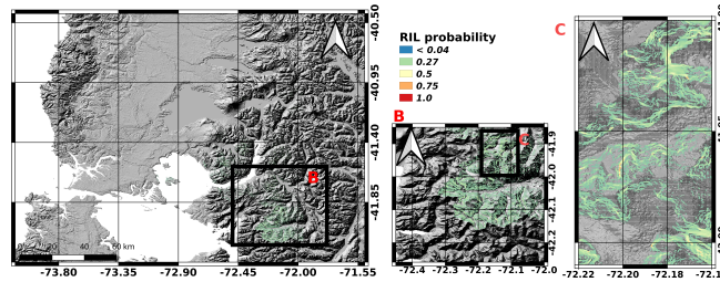
Figure 10. Zones susceptible to RIL for January 08, 2017. Results using Model 1 (probit). Hillshade based on SRTM data.
