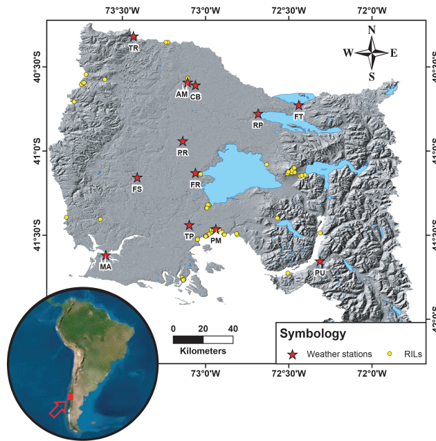
Figure 1. Study area in the Southern Andes Zone and the northern part of the Patagonian Andes. RIL events in the area are highlighted in yellow dots and red stars mark the meteorological stations available. Hillshade based on SRTM data.
