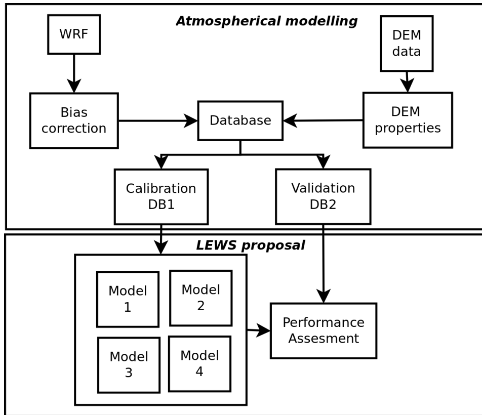
105 Figure 2 Short methodological description. The first phase explained in detail in section 3.1 and the second stage explained in sections 3.2 and 3.3.
