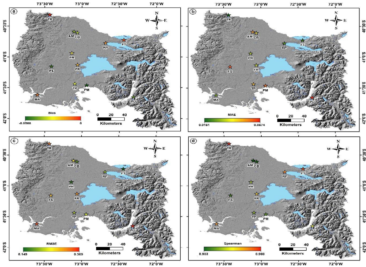
205 Figure 4 Spatial distribution of model corrected at weather stations using best results (PP_M4a). a) BIAS of the simulation in comparison with stations; b) MAE of the simulation in comparison with stations; c) RMSE of the simulation in comparison with stations; d) Spearman correlation coefficient of the simulation in comparison with stations. Hillshade based on SRTM data.
