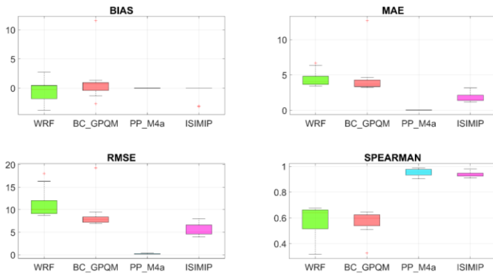
Figure 3 Precision and Reliability Indicators. Bias (mm), MAE (mm), RMSE (mm) and Spearman correlation coefficient. WRF is the uncorrected model, while the other models are the different methodologies used for correction by Meteolab.
