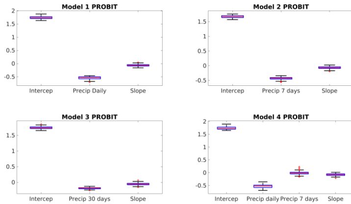
Distribution of estimators for each model with Probit distribution.
