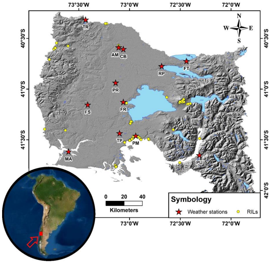
90 Figure 1 Study area in the Southern Andes Zone and the northern part of the Patagonian Andes. RIL events in the area are highlighted in yellow dots and red stars mark the meteorological stations available. Hillshade based on SRTM data.
