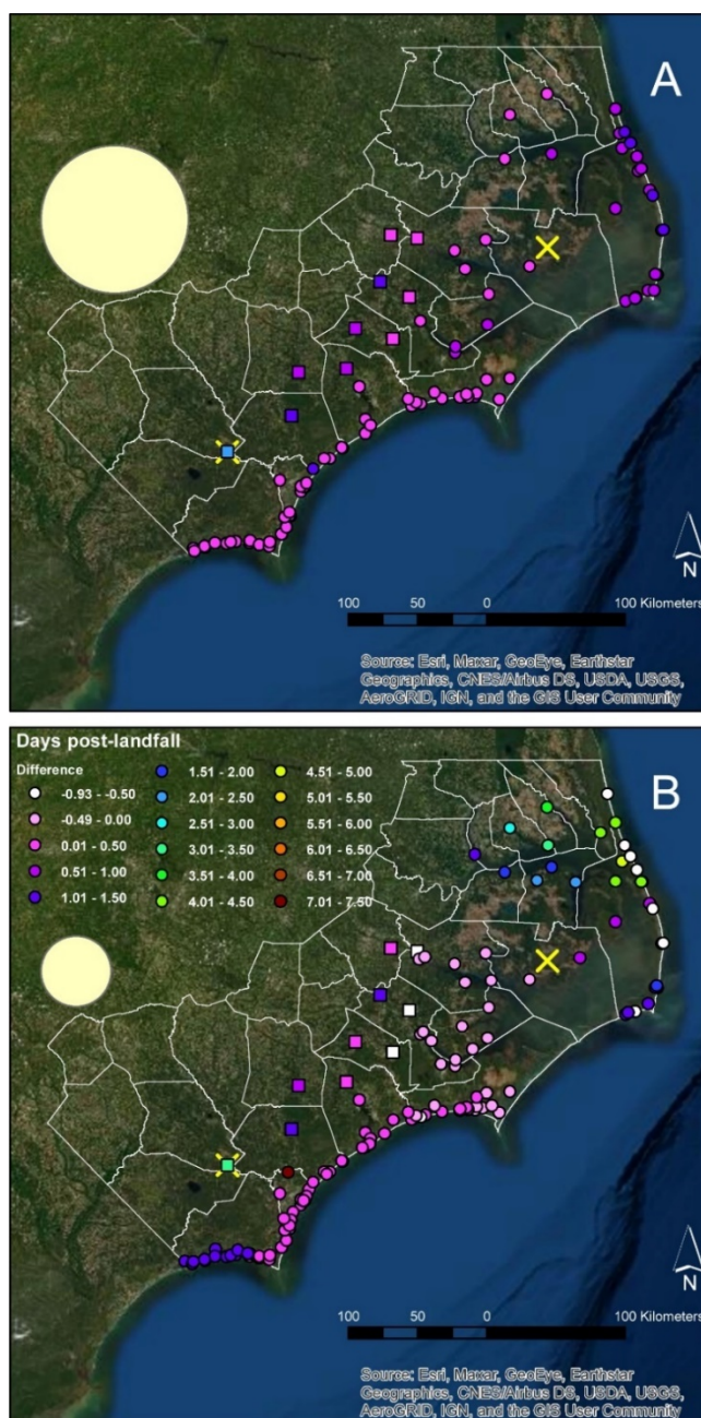
Figure 5. Maps of \Delta t_{ps-lf} (circles), time when river gauges first reached minor flood stage (squares) and locations of rain gauges (crosses). Large circles represent the area of similarity in \Delta t_{ps-lf} computed using the semivariogram range (a) as the 415 radius. A) is for Matthew and B) is for Florence.
