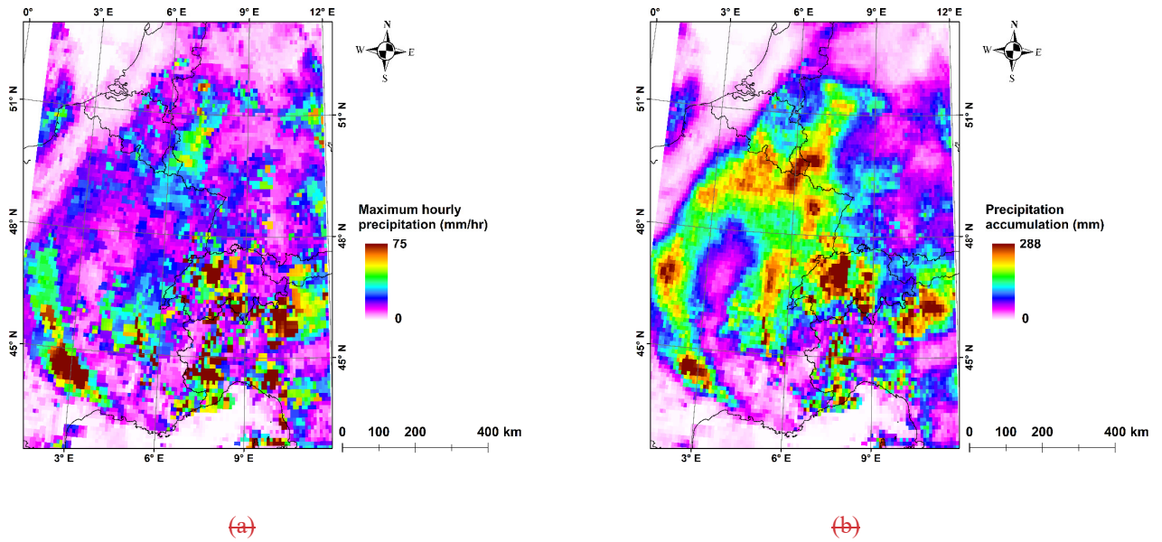
Figure 1. Spatial pattern of (a) maximum hourly precipitation and (b) precipitation accumulation during flooding period (12 to 15 July) over western Europe.
