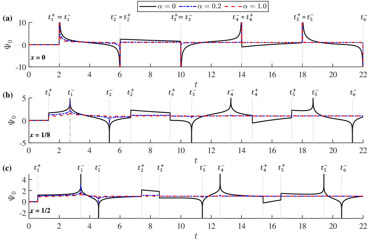
Figure 3. Function \Psi_0(x, t) at x=0 (a) x = 0, 1/8, 1/2 . (b) x = 1/8 and (c) x = 1/2 . Each panel shows graphs of the function for \alpha = 0, 0.2 , and 1.0 . Vertical dot lines represent the timing of singularities, t_m^\pm .
