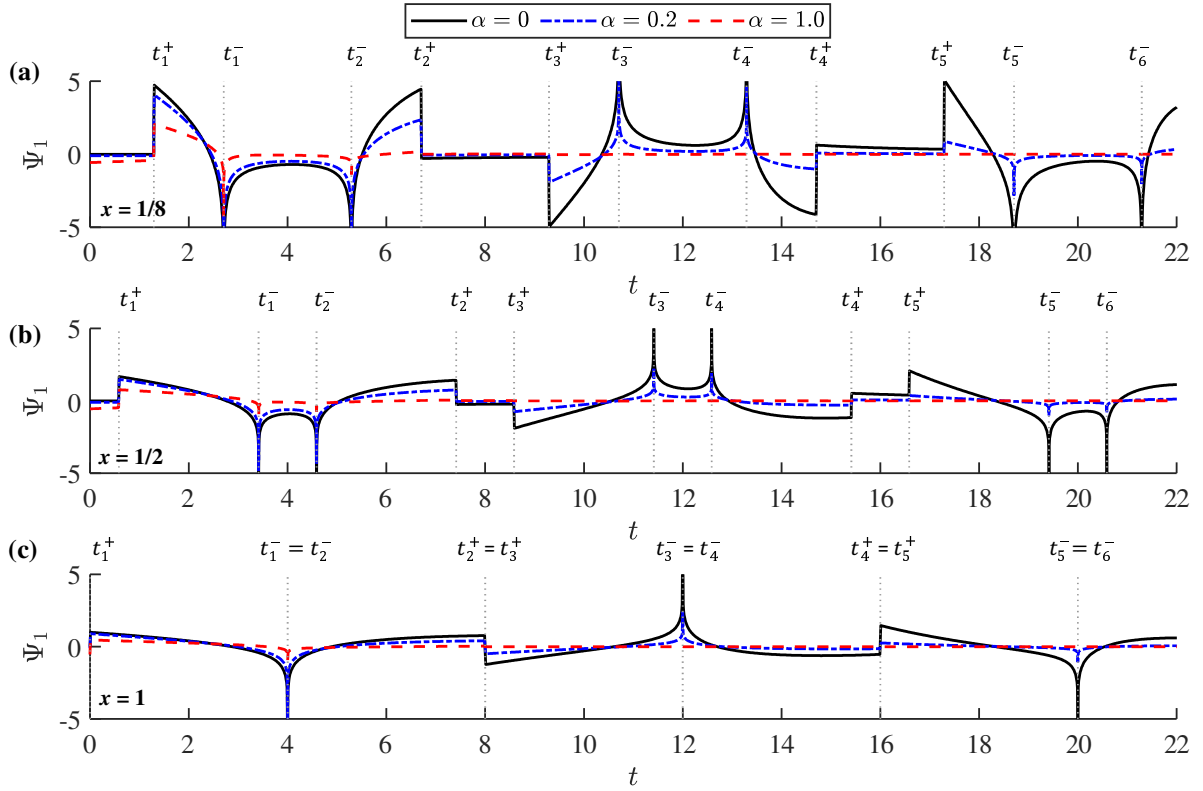
Figure 4. Function \Psi_1(x, t) at x = 1/8 (a) x = 1/8 , 1/2 , (b) x = 1/2 and (c) x = 1 . Each panel shows the graphs of the function for \alpha = 0, 0.2 , and 1.0 . Vertical dot lines represent the timing of singularities, t_m^\pm .
