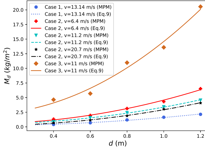
Figure 8. Evolution of the detrainment mass per unit of area with the tree diameter for different types of snow and front velocity (regular staggered forest, e = 8\text{ m} )
