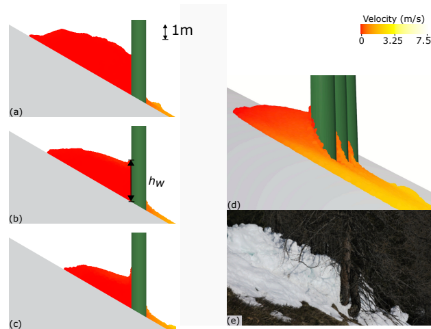
Figure 2. Cross-sectional view (passing through the center of the middle tree) of the snow stopped behind a group of three trees for different values of M : (a) M=1.2 , (b) M=1 , (c) M=0.8 ; perspective view of the stopped mass (d) in the simulation with M = 0.8 and d = 1 m and (e) from the field observation (Feistl et al., 2014)
