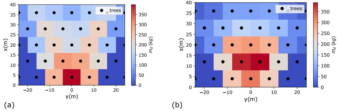
Figure 7. Distribution of the maximum detrainment mass behind each tree during the avalanche (regular staggered forest, d = 1\text{m} , e = 5.5\text{m} , snow properties: Case 2), (a) v_0 = 10\text{ m/s} , (b) v_0 = 22\text{ m/s}
