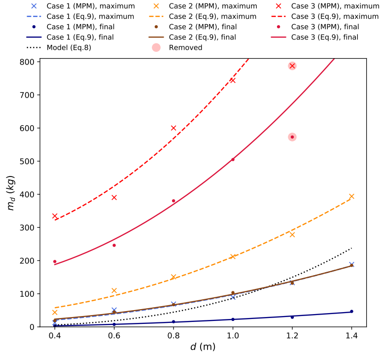
Figure 6. Evolution of the detrainment mass observed for the one tree arrangement and the fits with the tree diameter for 3 flow regimes : Case 1, Case 2 and Case 3 with respectively a front velocity of 12.5 m/s, 10.9 m/s and 10.75 m/s, ‘maximum’ refer to the maximum mass stored behind the tree and ‘final’ refer to the final mass stored. A slope of 30^\circ , and a top wedge angle of 60^\circ (from measurements Feistl et al. (2014)) are used for the theoretical model (Eq. 8). The removed point denotes a special case not considered in the proposed square relation in Eq. 9, since the entire avalanche in this case is stopped due to the low flow velocity and the high tree diameter. Please note that it is a coincidence that Case 1 maximum and Case 2 final agree well
