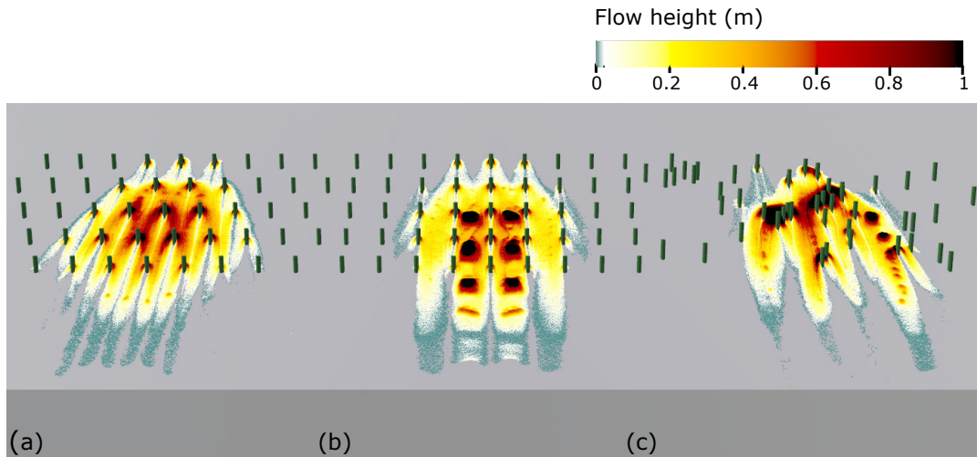
Figure 14. Flow height of the avalanche in a forest with (a) staggered arrangement, (b) aligned arrangement, (c) random arrangement, (Case 2, v_0 = 6 m/s)
