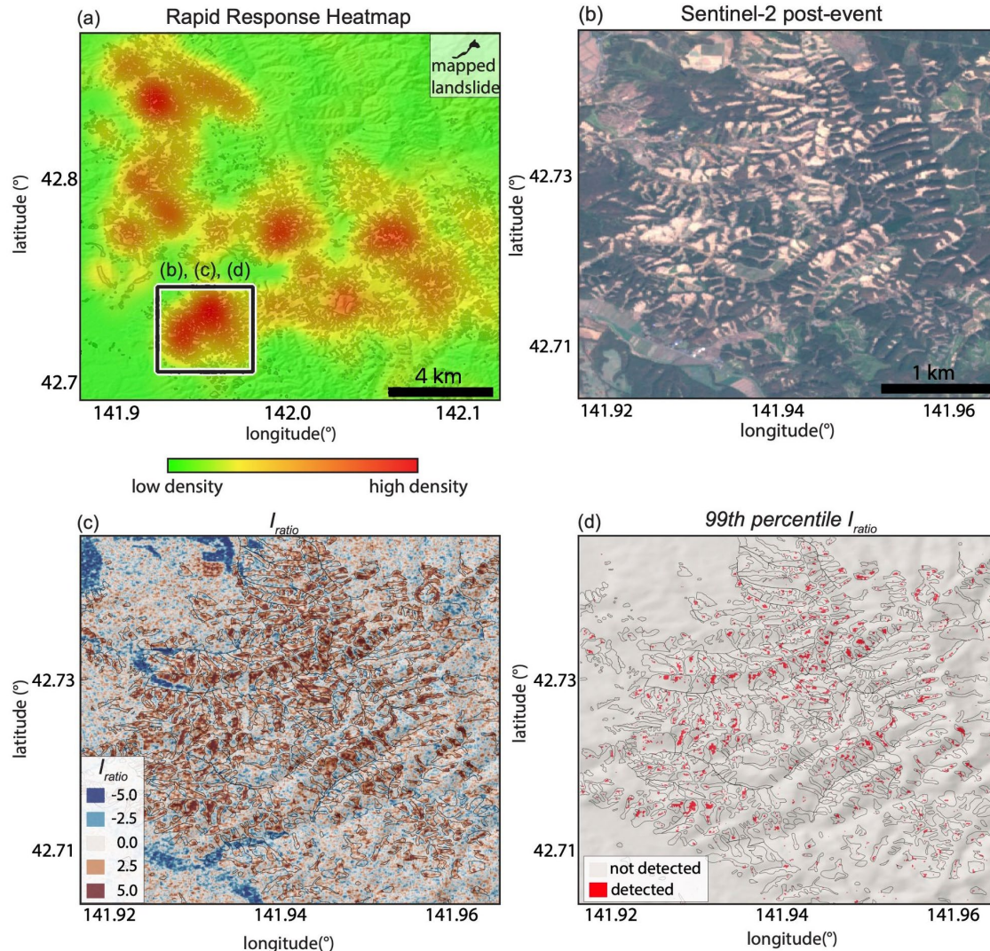
Figure 6. Simulated rapid response heatmap for the 2018 Hokkaido landslide event. (a) Heatmap with red colors showing a high density detected landslides draped over NASADEM hillshade of topography. Heatmap radius set to 100 pixels or 1 km. (b) Post-event Sentinel-2 optical image for sub-area shown in (a). (c) I_{ratio} map for sub-area. (d) I_{ratio} threshold map with red pixels that are \geq 99 th percentile I_{ratio} . Black landslide polygons in (a), (c), and (d) are from Zhang et al., (2019). SAR images made from stacks consisting of 150 pre-event SAR images collected between 01 August 2015 and 05 September 2018 and 3 post-event SAR images collected between 6-21 September 2018. DEM mask is used to remove low topographic slopes < 10^\circ in (a) and (d). No curvature mask is used because the landslides appear to have been sourced from hilltops.
