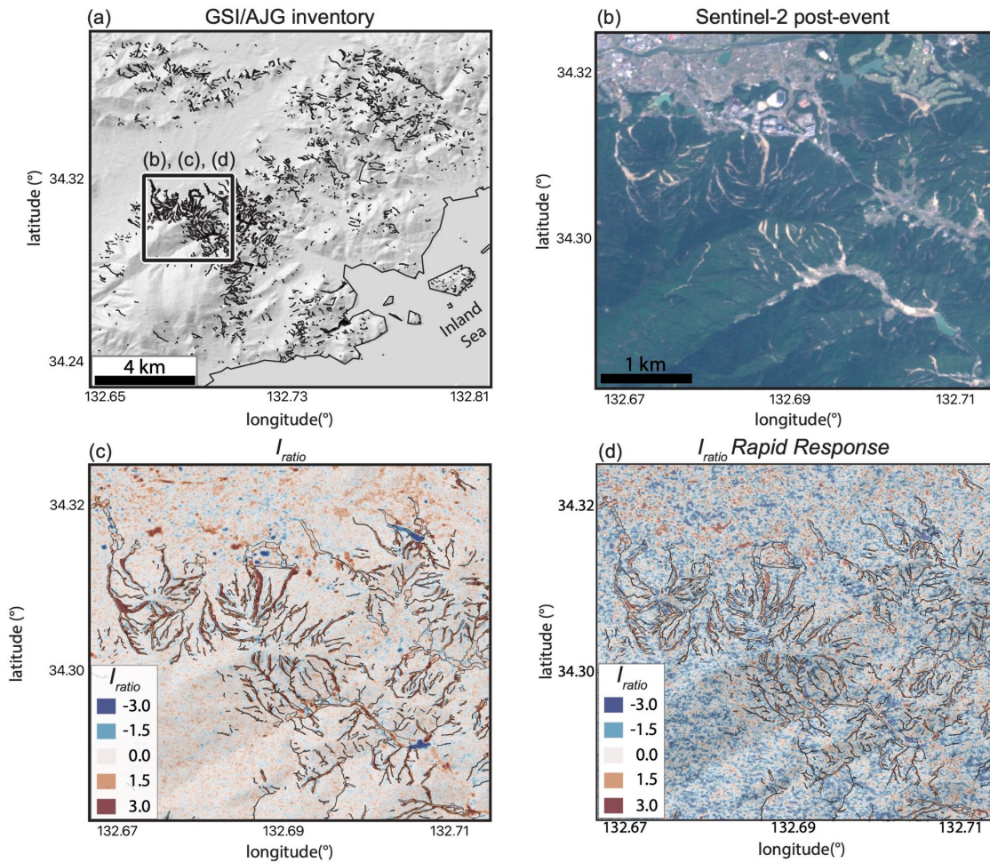
Figure 2: 2018 rainfall triggered landslides in the Hiroshima Prefecture. (a) NASADEM hillshade map for Area of interest (AOI) for our study. Black polygons show the GSI/AJG landslide inventory draped on the NASADEM hillshade map with the black box highlighting a sub-area of the AOI for plots b-d. (b) Sentinel-2 optical image showing landslide scars. (c) SAR backscatter intensity change for combined ascending & descending stacks. SAR backscatter change maps were created from stacks made from 142 combined ascending & descending pre-event SAR images collected between 01 May 2015 and 29 June 2018 and 133 post-event SAR images collected between 09 July 2018 and 29 May 2020 and represent our best case landslide identification. (d) SAR backscatter intensity change for simulated rapid response consists of stacks made from the same 142 pre-event SAR images and 5 post-event SAR images collected between 9-24 July 2021. Red colors correspond to a decrease in post-event backscatter intensity (positive I_{ratio} values). Black polygons in (c) and (d) show the GSI/AJG landslide inventory. No DEM mask is applied to (c) or (d).
