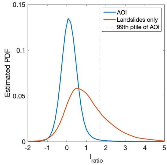
Figure A1A2: Kernel density function of I_{ratio} values for the 2018 Hiroshima landslide event. I_{ratio} distribution for the full AOI including both landslide and non-landslide areas. (b) I_{ratio} distribution for the true landslides mapped by GSI/AJG. I_{ratio} calculated using combined ascending & descending stacks from 142 pre-event SAR images collected between 01 May 2015 and 29 June 2018 and 133 post-event SAR images collected between 09 July 2018 and 29 May 2020. This plot corresponds to our “best case” landslide detection described in section 4.1.
