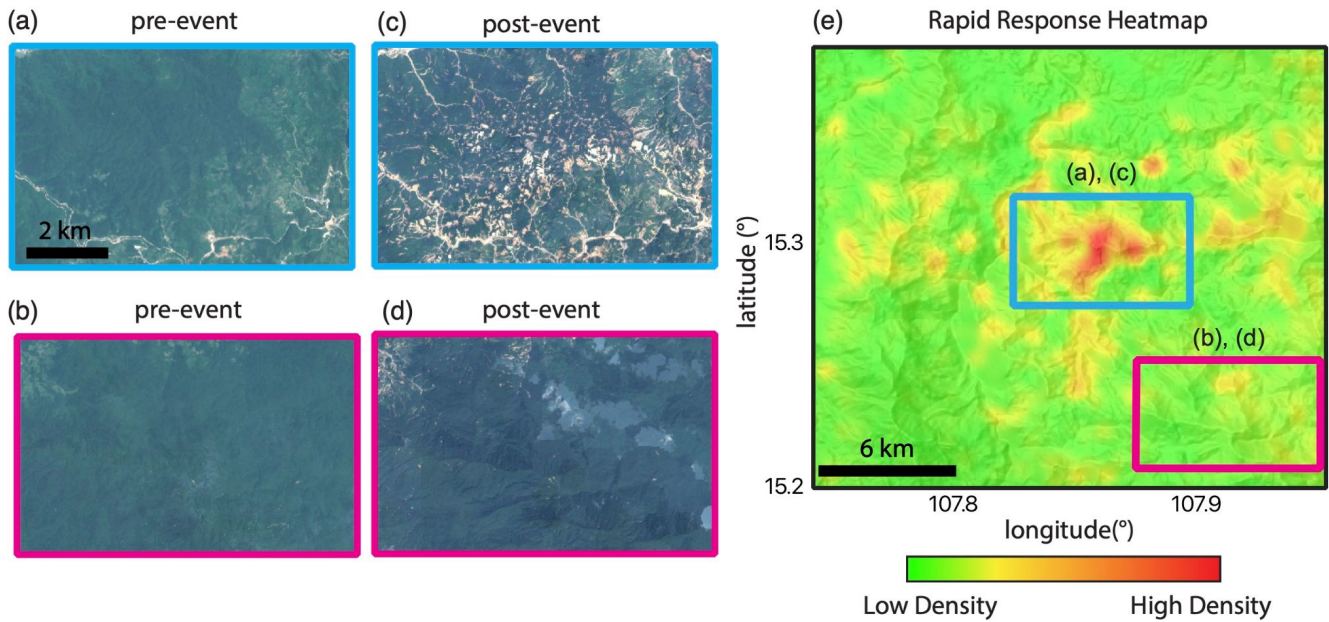
430 Figure 8. Simulated rapid response heatmap for Quang Nam, Vietnam. (a-d) Pre- and post-event Sentinel-2 optical images for high and low landslide density zones identified with the heatmap. (e) Heatmap draped over the NASADEM hillshade of the topography with red colors corresponding to areas with high potential landslide density. Heatmap made from stacks consisting of 253 pre-event SAR images 435 2020. Heatmap radius set to 100 pixels or 1 km. DEM mask is used to remove low topographic slope < 10^\circ and convex curvature > -0.005 \text{m}^{-1} . Blue and magenta rectangles show zoomed in areas in (a-d).
