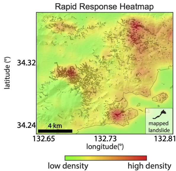
375 Figure 5: Simulated rapid response heatmap for the 2018 Hiroshima landslide event. Heatmap with red colors showing a high density of potential landslides. Black polygons are from GSI/AJG inventory. Pre-event stack created from 142 combined ascending & descending SAR images collected between 01 May 2015 and 29 June 2018 and post-event stack created from 5 SAR images collected between 9-24 July 2021. Heatmap radius set to 100 pixels or 1 km. DEM mask is used to remove low topographic slope ( < 5^\circ ) and convex curvature ( > -0.005 \text{ m}^{-1} ).
