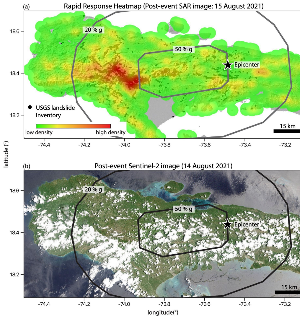
465 Figure 9. Real time rapid response heatmap for the 2021 earthquake-triggered landslides in Haiti. (a) Landslide heatmap draped over the NASADEM hillshade of the topography with red colors corresponding to areas with high potential landslide density. Heatmap made from stacks consisting of 104 descending pre-event SAR images collected between 1 August 2017 and 13 August 2021 and 1 descending post-event SAR images collected on 15 August 2021. Heatmap radius set to 300 pixels or 3 km. DEM mask is used to remove low topographic slope < 10^\circ . Black circles show USGS landslide inventory that was released and updated between 17 - 23 August 2021. The USGS inventory was made from Maxar and Planet imagery. (b) Post-event Sentinel-2 optical imagery showing high cloud cover after 470 on the day of the earthquake. (a,b) Black star shows the M_w 7.2 earthquake epicenter and contours show the peak ground acceleration data as a percentage of gravity (g) provided by the USGS (see data availability).
