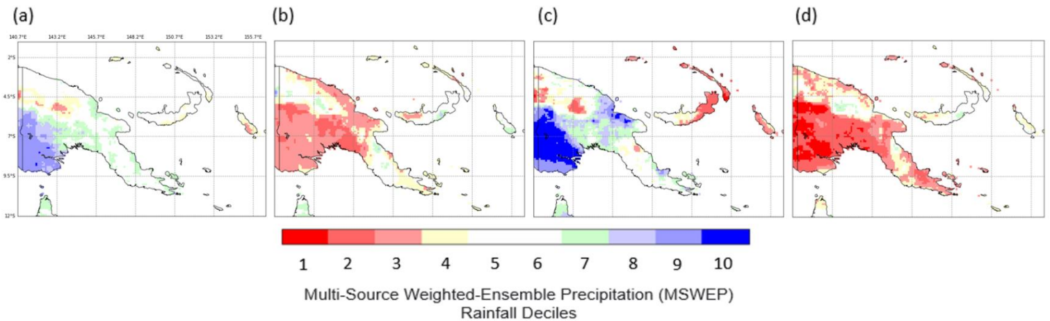
1080 Figure 2. Multi-Source Weighted-Ensemble Precipitation (MSWEP) rainfall deciles in response to various climate drivers: (a) Negative IOD phase (during 1981, 1989, 1992, 1996, 1998, 2010, 2014, and 2016 years), (b) Positive IOD phase (during 1982, 1983, 1994, 1997, 2006, 2012, 2015, and 2019 years), (c) Negative IOD phase and La Niña ENSO phase (during 1989, 1998, and 2010 years) and (d) Positive IOD phase and El Niño ENSO phase (during 1982, 1994, 1997, 2006, and 2015 years). Deciles are compared to a 1980–2020 base period. Figure adapted from Bhardwaj et al. 2021b.
