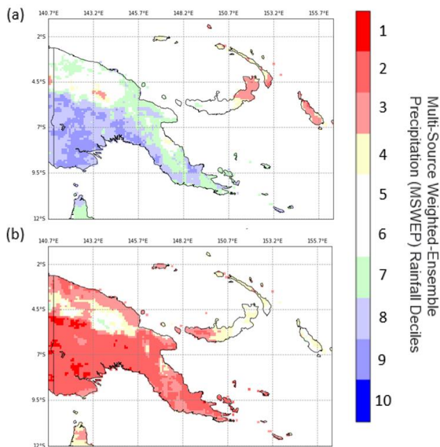
1075 Figure 1: Multi-Source Weighted-Ensemble Precipitation (MSWEP) rainfall deciles in (a) La Niña events (La Niña years being 1988, 1989, 1995, 1998, 1999, 2000, 2007, 2010, 2011 and 2020) and (b) El Niño events (El Niño years being 1982, 1987, 1991, 1992, 1994, 1997, 2002, 2006, and 2015) compared to a base period of 1980–2020. Figure adapted from Bhardwaj et al. 2021b.
