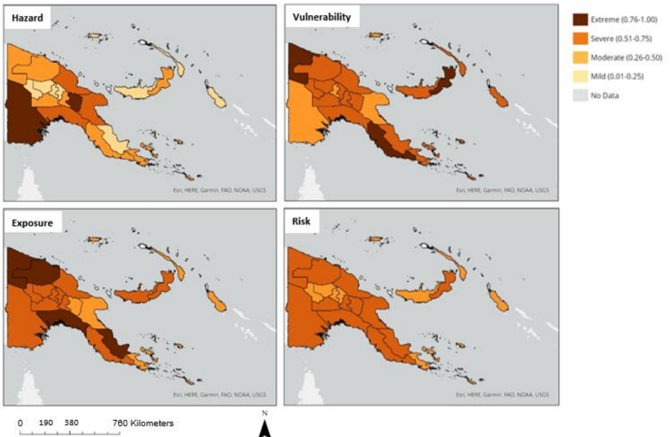
1040 Figure 5. Overall drought risk maps of PNG provinces for 2014 including a drought hazard, drought vulnerability, drought exposure and drought risk map detailing the index level of each province. The index level is classified on a deepening orange colour scale from Mild (index values from 0.01-0.25) to Extreme (index values from 0.76-1.00).
