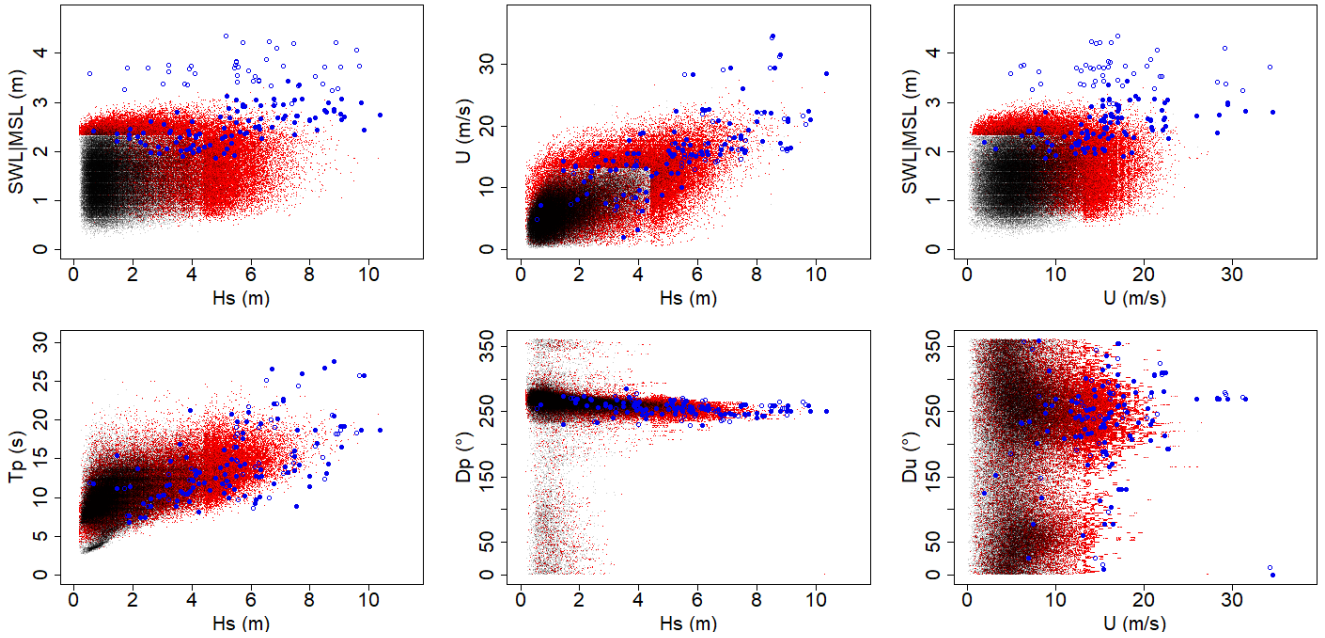
115 Figure 3: Overview of the N=50,000 randomly generated samples of offshore conditions (red dots). Black dots correspond to the hindcast conditions used to fit the statistical methods described in Sect. 3.3. Blue (open and filled) circles correspond to the n=144 training data used to set-up the GP metamodel (the selection approach is detailed in Sect. 3.2). The open circles correspond to cases that are deliberately selected outside the range of the red dots to cover a broader range of situations.
