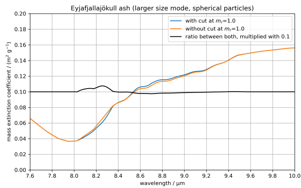
Figure B3. Mass extinction coefficients for spherical particles with the original refractive index m from Fig. B2 (orange line) and with the same refractive index m_r cut at 1 in the spectral region between 8 and 10 \mu\text{m} (blue line). The black line is the ratio between orange and blue line and has been multiplied by 0.1, meaning that a value of 0.1 corresponds to exact the same values in the two situations.
