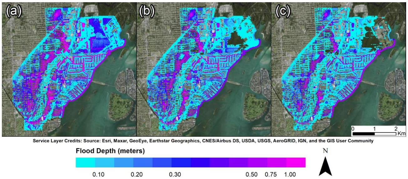
785 Figure 9. Spatial distribution of maximum inundation depths for Tropical Storm Leslie (a), Tropical Storm Andrea (b), and 25 May 2020 event (c).
