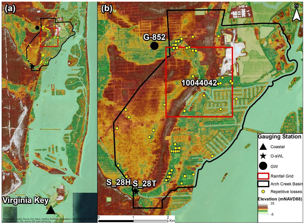
755 Figure 3. Geographical location of selected data in the study site. (a-b) Topographic map showing the location of the Arch Creek Basin (black polygon), and the distribution of closest gauging stations to the study site (black markers), rainfall grid (red square), and properties that have experience severe repetitive losses due to flooding events (yellow).
