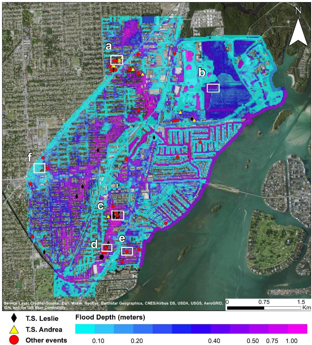
795 Figure 11. Distribution of maximum flood depths for Tropical Storm Leslie. The markers indicate repetitive loss properties caused by Tropical Storm Leslie (black), Tropical Storm Andrea (yellow) or other storm events (red). Maximum flood depths at six sample locations (white) are presented in Fig. 11.
