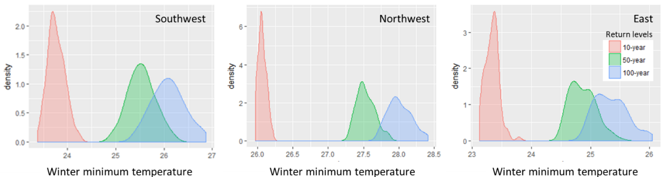
Figure 12: Density plots of 10, 50, and 100-year return periods of the winter minimum temperatures in the Southwest, Northwest, and East of Mongolia with 90% confidence intervals. Please note that the x-axis shows temperature below zero (i.e., for Southwest, the axis shows negative 23.5 to 27 Celsius degree). The data is simulated 100 times from the Siberia data. For example, the plots show that the median of 100 year return periods are -26.08, -27.99, and -25.31 Celsius degrees for the Southwest, Northwest, and East.
