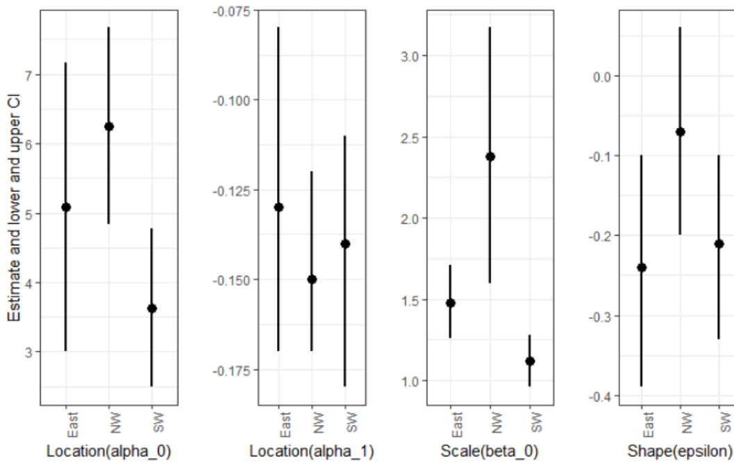
310 Figure 5: 95% Confidence intervals of parameters, using other climate variables based on the normal approximation. Also numerical values are listed in Table S.2.
