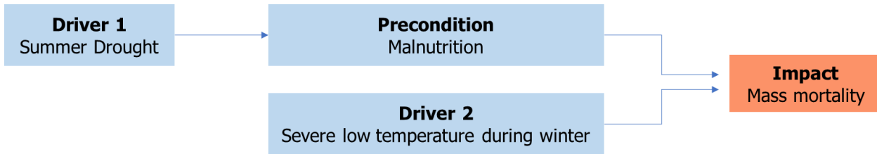
Figure 1: Dzud is a preconditioned compound event.
