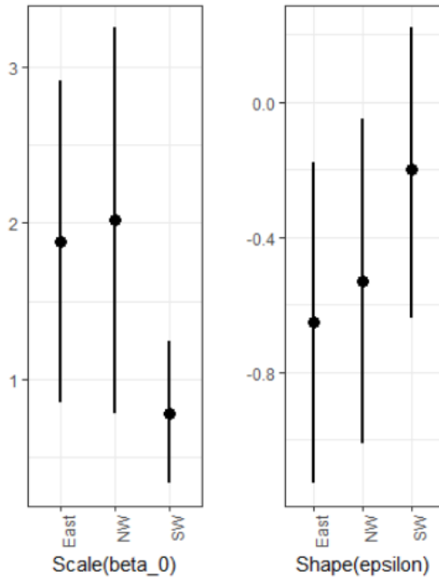
Figure 9: 95% Confidence intervals of parameters, using other climate variables based on the normal approximation.
