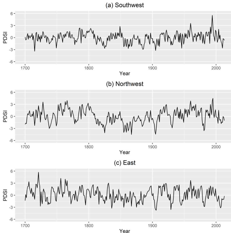
Figure 3: Time series of tree-ring reconstructed PDSI in (a) the Southwest, (b) the Northwest, and (c) the East clusters.
