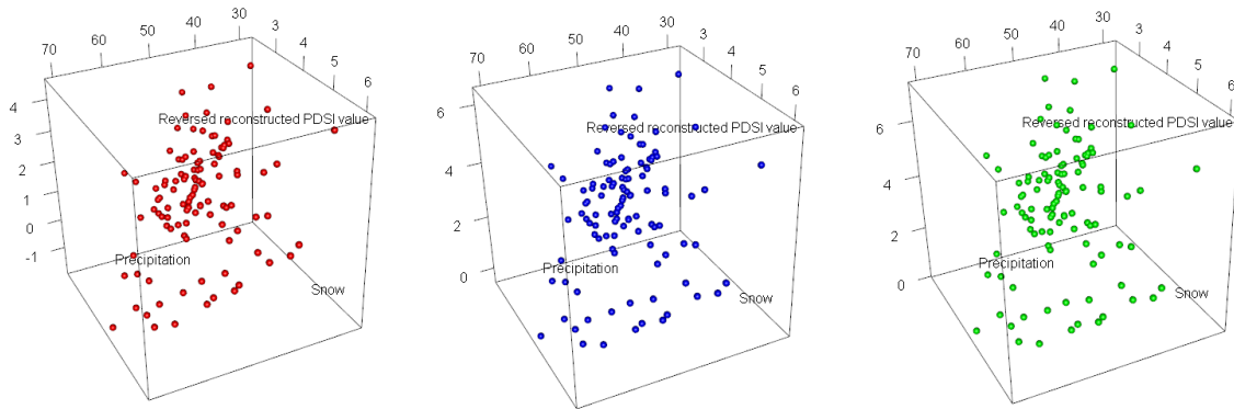
340 Figure 8: Relationship between precipitation, snow and reversed reconstructed PDSI values in the Northwest based on the best GEV model. Since the PDSI values are reversed, the positive values mean drought conditions. The x axis is precipitation, the y-axis is snow, and the z-axis is reversed reconstructed PDSI values. The left cube is for 10-year events, the central is for 50-year events, and the right is for 100-year events. Since the best GEV model contains
