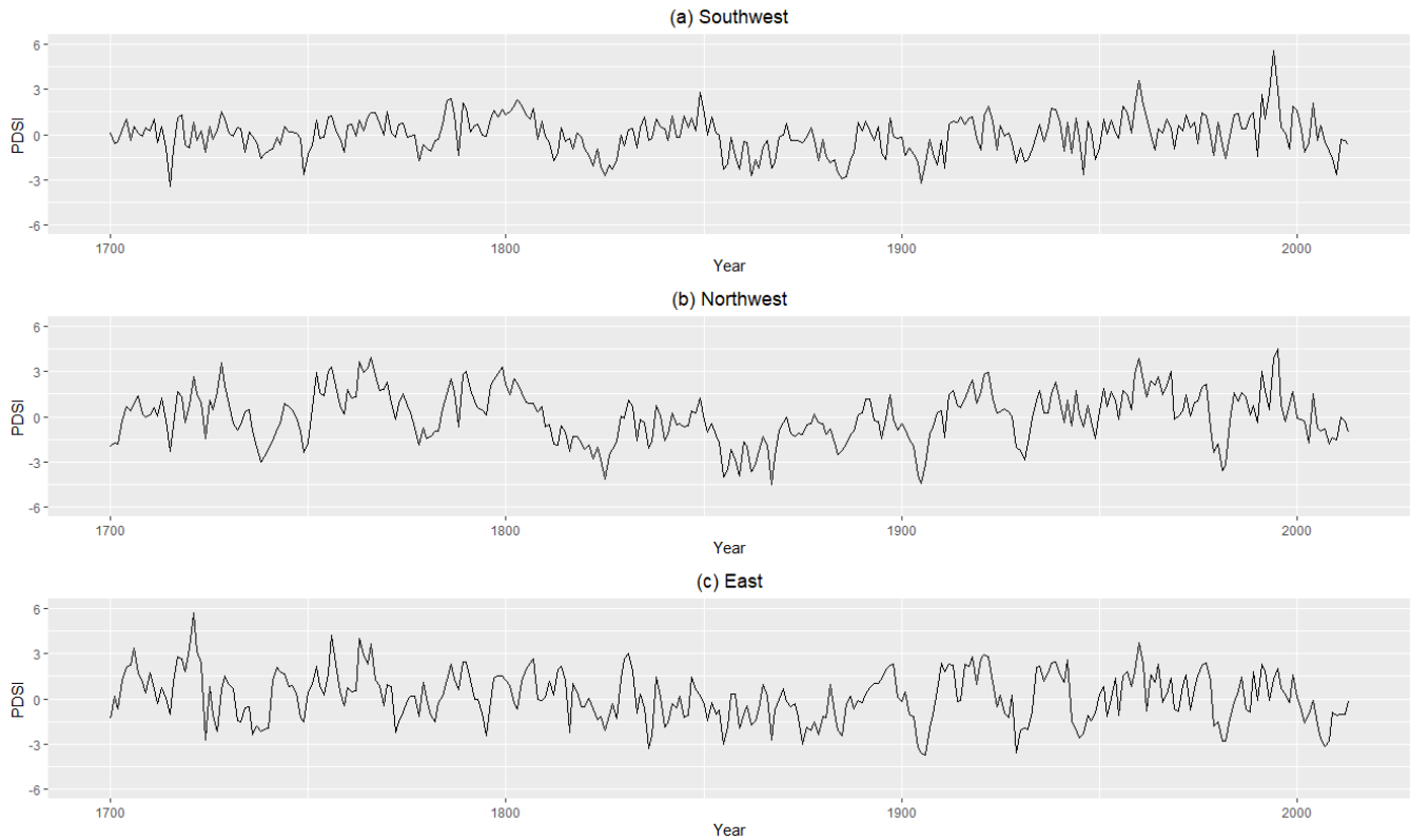
Figure 2: Time series of tree-ring reconstructed PDSI in (a) the Southwest, (b) the Northwest, and (c) the East clusters.
