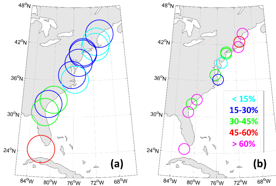
325 Figure 6. Percentage of TCs that produce surge exceeding the location's 1-yr return level and: a) are within 250 km; b) are within 100 km and whose MSLP is less than or equal to the average MSLP of all TCs within 100 km. Size of circles indicates the search radius around each location. Color coding is based on the percentage value with <15 % (light blue), 15-30 % (dark blue), 30-45 % (green), 45-60 % (red), and >60 % (magenta).
