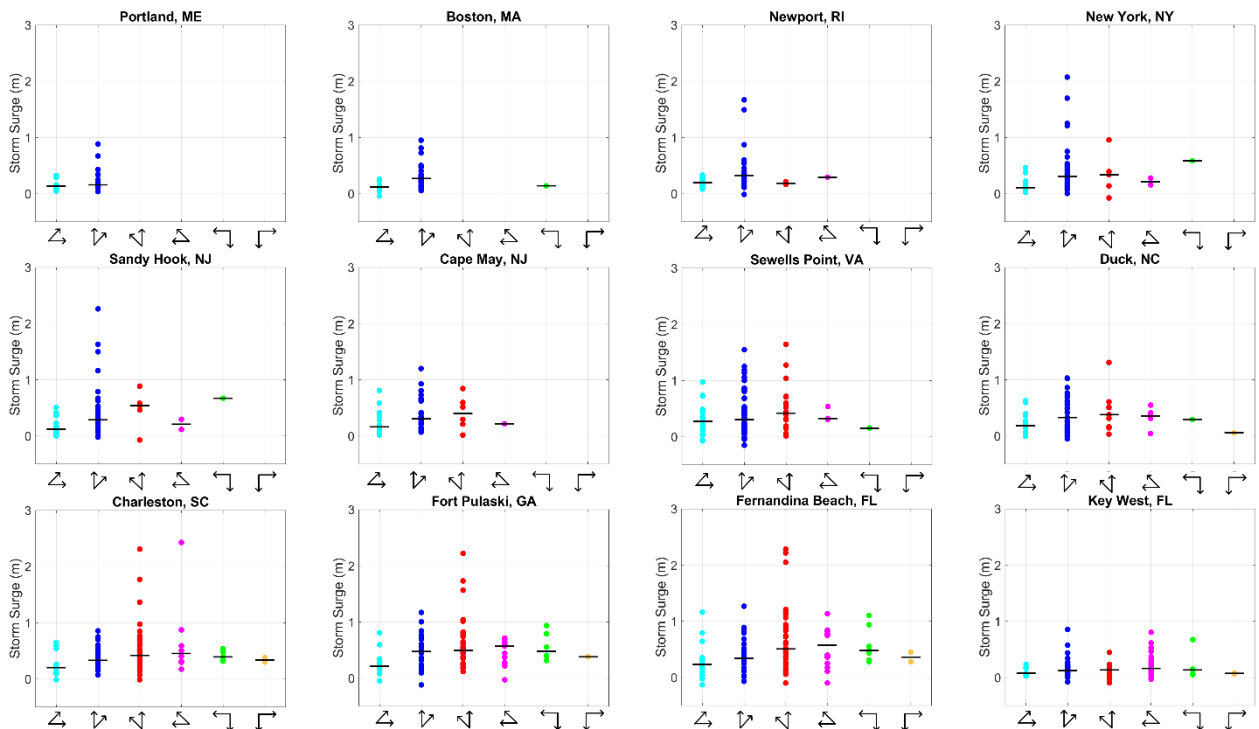
Figure 4. Storm surge (m) separated by track path angle. Arrows along x-axis indicate range of TC track movement and is similar to track path angle key in figure 1. From left to right, arrows correspond to ENE (light blue), NNE (dark blue), NNW (red), WNW (magenta), SW (green) and SE (orange). Horizontal black line indicates the median value of storm surge for each group of track path angles.
