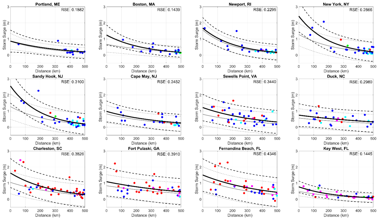
265 Figure 5. Exponential fit (black solid line) between storm surge (m) and TC proximity (km) for only strong TCs within 500 km with 95 % confidence intervals (dashed black line). Exponential fit (gray solid line) and 95 % confidence intervals (dashed gray line) from Figure 2 is also included for comparison to all TCs regardless of intensity. Data points are color coded based on average track path angle as outlined in Figure 4. Residual standard error (RSE) is provided for the exponential fit.
