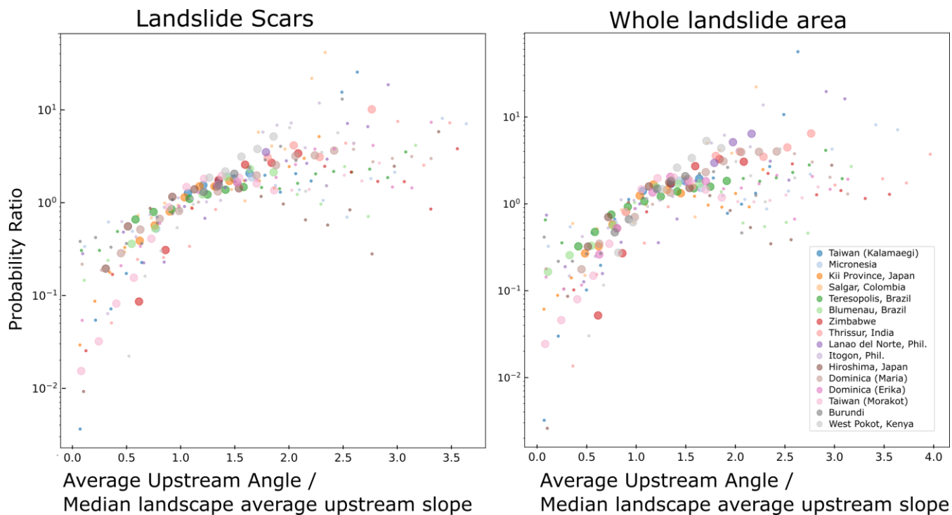
Figure 5: Landslide probability ratio against the average upstream angle normalized by the median of the local landscape, for the scar area (left) and the whole landslide area (right). The size of the points depends on whether the difference between landslide and topography exceeds the calculated confidence interval for that bin interval; larger points indicate significant deviation ( p > 0.95 ), and small points indicate the difference is not significant at that probability level.
