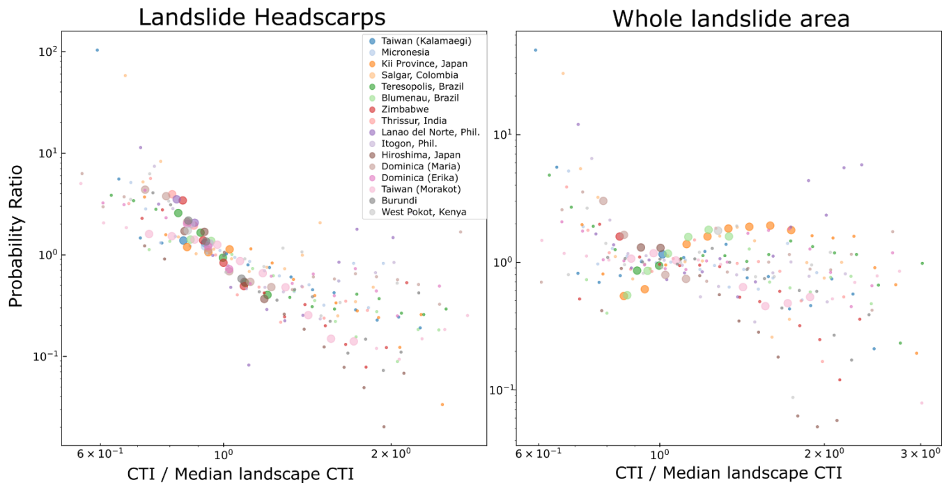
820 Figure 6: Same as Figure 4 but for the Compound Topographic Index (CTI). Note that the x-axis is a logarithmic scale.
