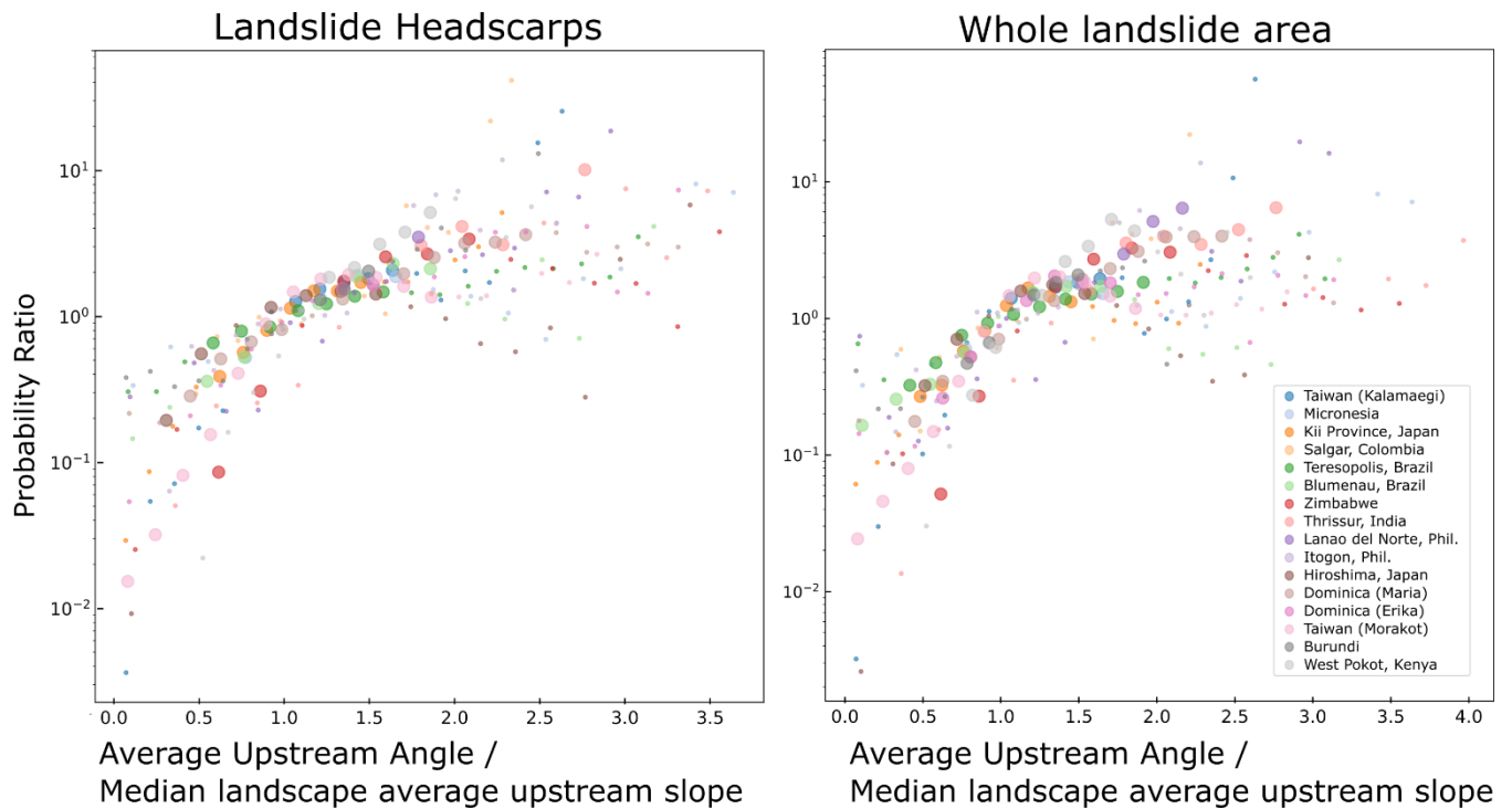
Figure 5: Landslide probability ratio against the average upstream angle normalized by the median of the local landscape, for the scar area (left) and the whole landslide area (right). The size of the points depends on whether the difference between landslide and topography exceeds the calculated confidence interval for that bin interval; larger points indicate significant deviation ( p > 0.95 ), and small points indicate the difference is not significant at that probability level.
