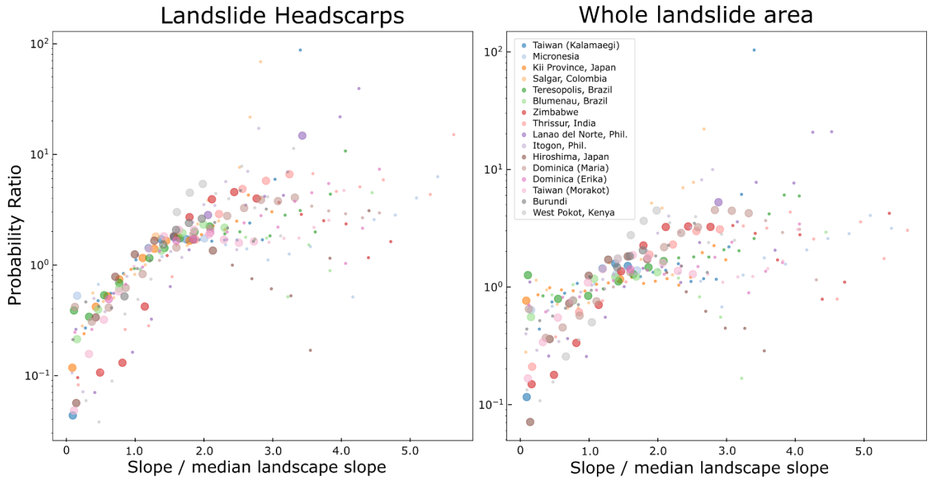
Figure 4: Landslide probability ratio against the slope normalized by the median of the local landscape, for the scar area (left) and the whole landslide area (right). The size of the points depends on whether the difference between landslide and topography exceeds the calculated confidence interval for that bin interval; larger points indicate significant deviation ( p>0.95 ), and small points indicate the difference is not significant at that probability level. 810
