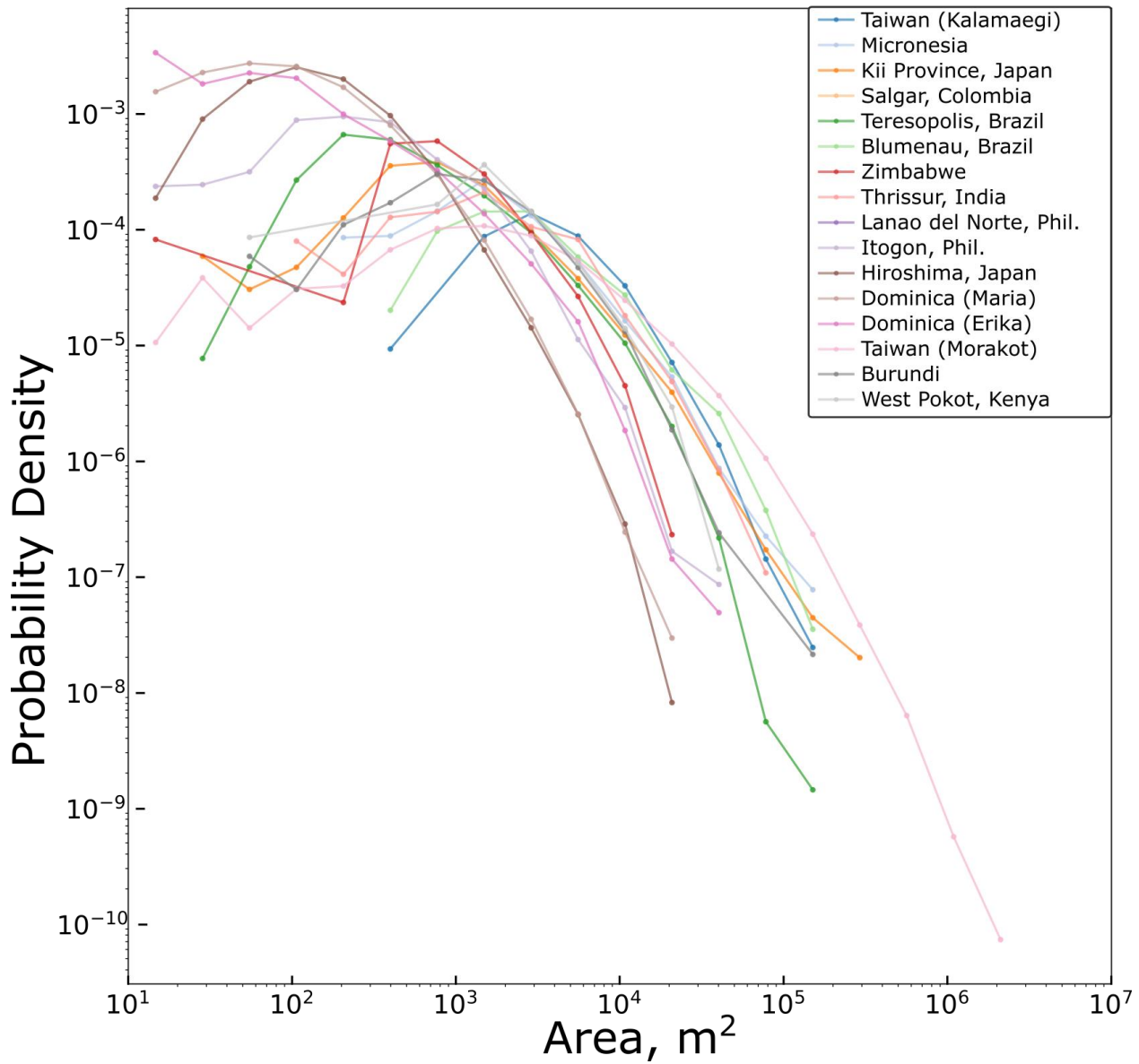
795 Figure 2: Probability density for landslides in each event inventory, obtained as the number of landslides with areas falling into logarithmic bins (consistent bins for all inventories), N_{[A:A+dA)} , normalized by the bin width, dA , and the total number of slides for the event, N_{tot} (see Malamud et al., 2004).
