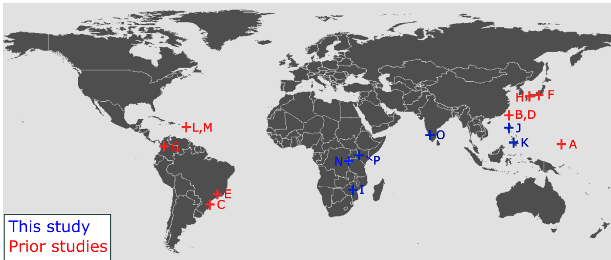
790 Figure 1: Locations of landslide inventories considered in this study. Locations labelled in red have been published previously, while those in blue are presented for the first time here. Satellite images of the newly mapped landslide inventories can be found in the Supplemental material. Table 1 contains the details of each of the inventories, organised in alphabetical order.
