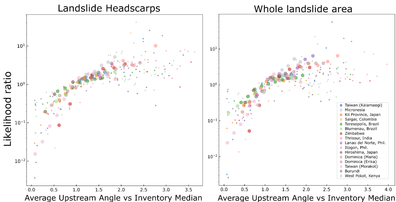
Figure 5: Landslide likelihood ratio against the average upstream angle normalized by the median of the local landscape, for the scar area (left) and the whole landslide area (right). The size of the points depends on whether the difference between landslide and topography exceeds the calculated confidence interval for that bin interval; larger points indicate significant deviation ( p > 0.95 ), and small points indicate the difference is not significant at that probability level.
