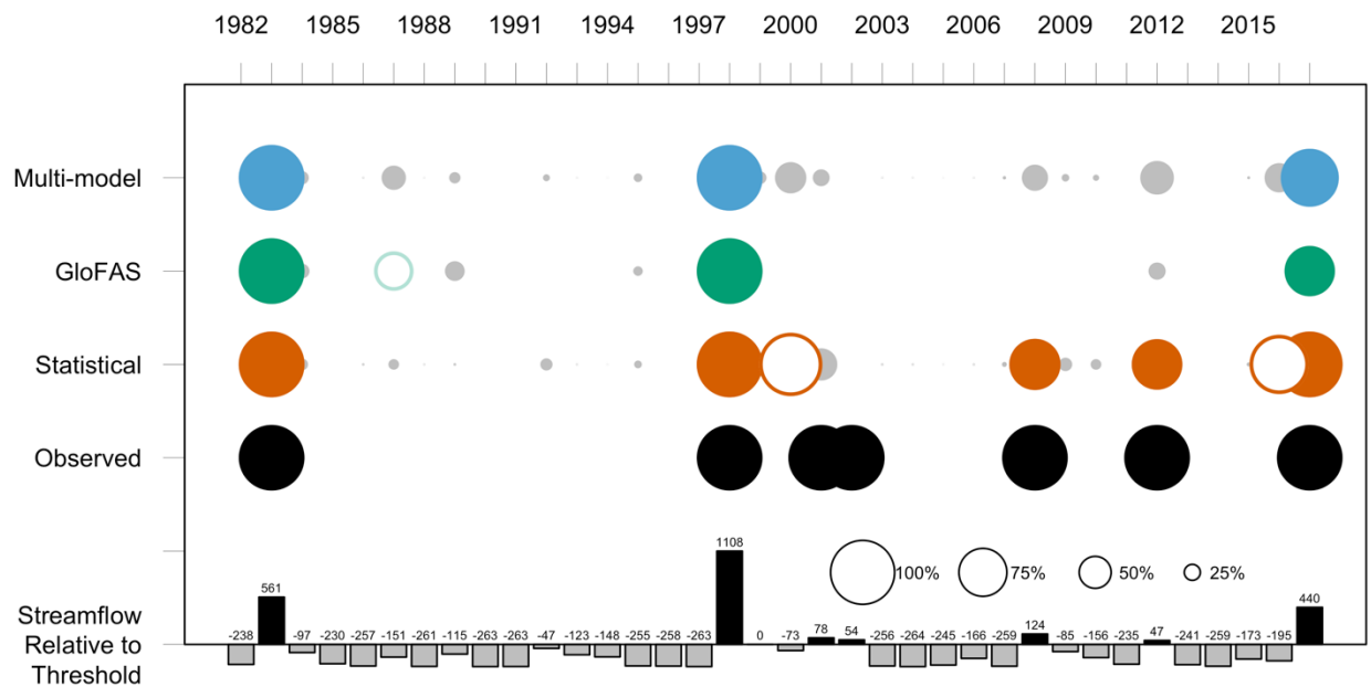
Figure 7: Same as Figure 6 for Piura River at Puente Sánchez Cerro. At Puente Sánchez Cerro, all models trigger early actions during the three largest events in 1983, 1998 and 2017 – each of which resulted in significant impacts in the Piura River basin, collectively killing over 1000 people and affecting another 3.6 million (BBC News, 2017; Caviades, 1984; EM-DAT, 1988; French and Mechler, 2017; USAID, 1998) (Figure 7). The statistical model includes two false positives in 2000 and 2016 with 93% and 87% predicted probabilities of exceedance (observed streamflow was at the 74 th percentile in 2000). Additional historical years (2001, 2002, 2008 and 2012) also meet the criteria for early action with evidence of flooding in the Piura province, collectively resulting in 60 deaths and affecting 508,000 people (EM-DAT, 1988), although streamflow magnitudes were substantially lower. Of these the statistical model captured two (2008, 2012) while GloFAS failed to capture any.
