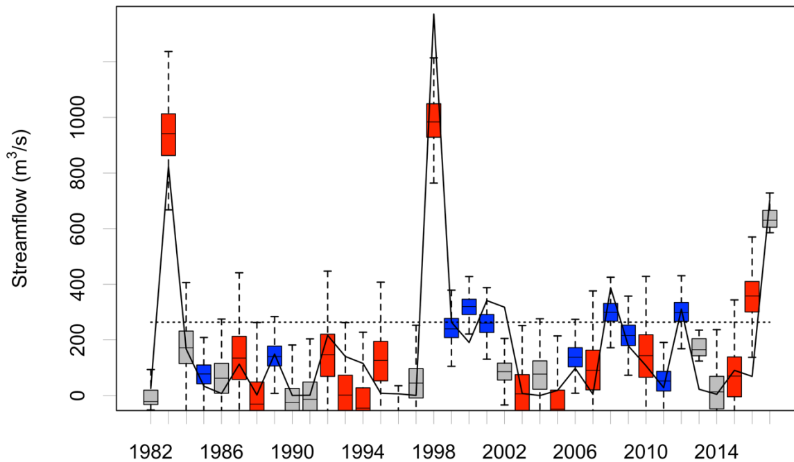
390 Figure 5: Piura River at Puente Sánchez Cerro FMA streamflow hindcast using the statistical prediction model. The black solid line illustrates observed FMA streamflow; the black dotted line indicates the 80 th percentile of FMA observed streamflow. Red (blue) boxes represent years with pre-season El Niño (La Niña) conditions.
