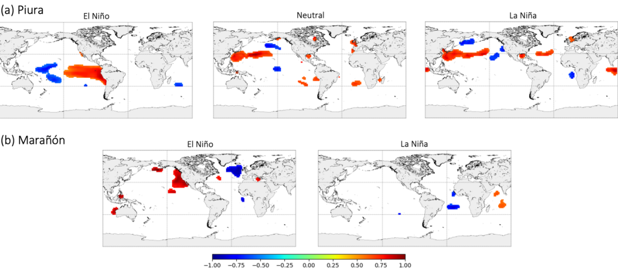
Figure 3: Correlation maps of seasonal streamflow at a) Piura (FMA) and b) Marañón (MAM) with pre-season SSTs by ENSO phase. Only regions statistically significantly correlated at p<0.05 are included.
