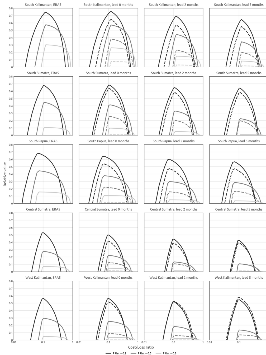
Figure 9: Relative value of active fires > 10 cases prediction for users with different cost-loss ratios. Shown are relative value of ERA5-based predictions and SEAS-based (solid lines) and climatology-based (dashed lines) predictions at different lead times (columns) for different sub- regions (rows). Line shading (legend) indicates different fire prediction probability thresholds at which the relative value curves are calculated.
