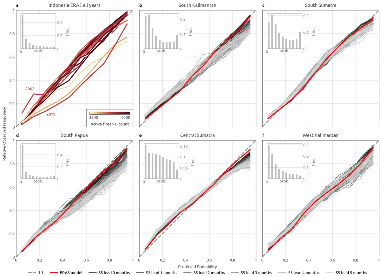
435 Figure 4: Reliability diagrams of active fire counts > 0 case occurrence probability predictions. Inset axes show ERA5-based probability prediction frequency histograms. a) ERA5-based prediction for all of Indonesia reliability curves for each year in the record. The colour of the lines corresponds to active fire > 0 cases mean count for the year. (b-f) Mean reliability curves for the sub-regions (Fig. 1), showing ERA5 (red) and SEAS5-based ensemble mean prediction reliability curves at different lead times (shades of grey, bottom legend). Dotted lines indicate perfect reliability (1:1 fit).
