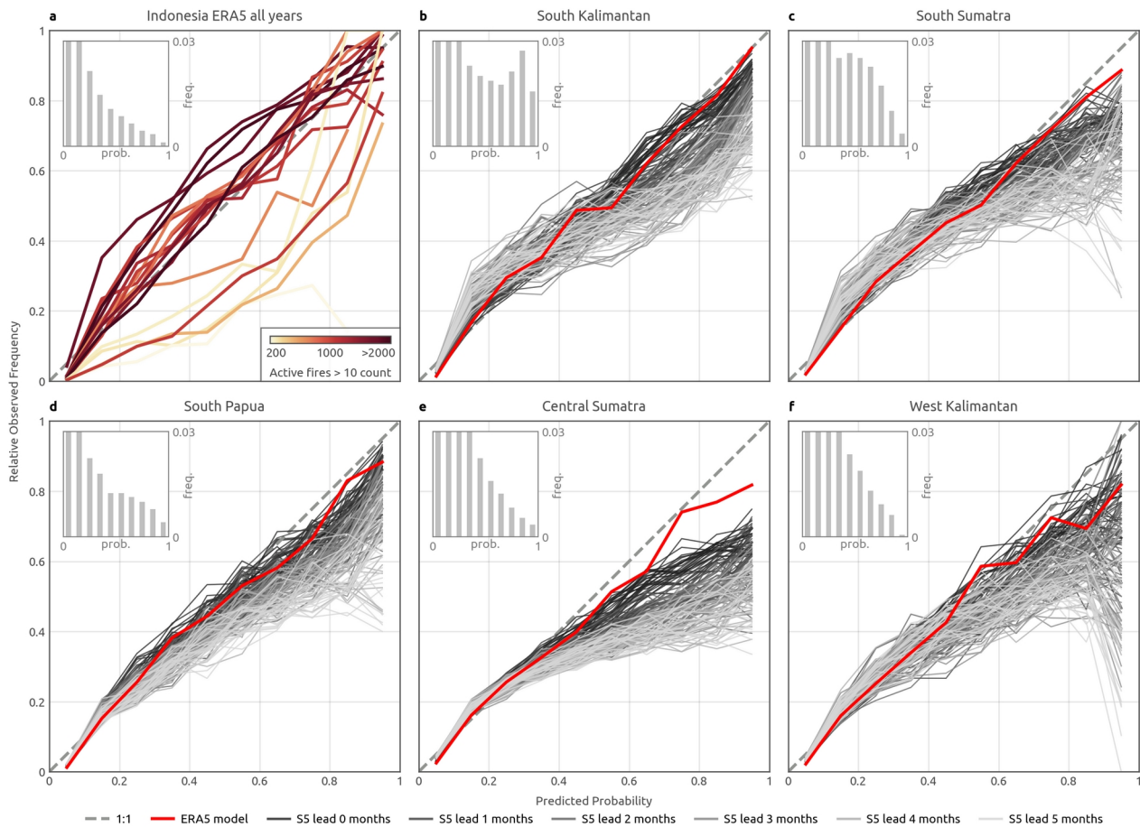
Figure 5: Same as Fig. 43. but for prediction of probability for active fire > 10 cases.
