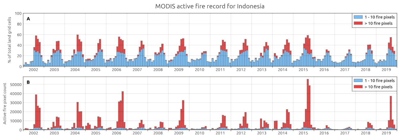
145 Figure 2: MODIS active fire record for Indonesia during 2002-2019 period. a) % of total land grid cells in the study region (n = 2080) with active fire detections. The two categories shown are for grid cells with relatively low fire counts (1-10 fire pixels per month) and higher degree of fire presence (> 10 fire pixels) in blue and red colours, respectively. b) Total monthly MODIS active fire counts attributable to grid cells of the two categories.
