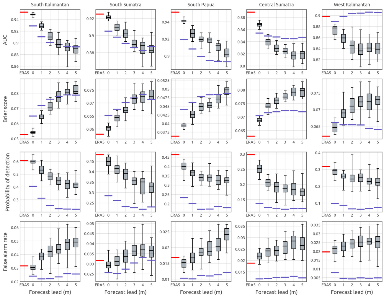
500 Figure 7: Skill scores for prediction of active fires > 10 cases. Shown are mean values of area under receiver operating characteristic curve (AUC), Brier score, probability of detection and false alarm rate (figure rows) for the different sub-regions (figure columns). ROC curves are shown in Figure S2 (Supplementary figures). The values for ERA5-based model predictions are shown as red bars, climatology-based predictions are depicted as blue bars, while boxplots indicate SEAS5 ensemble member prediction values at different lead times. For boxplots, shown are the median value (grey bar), interquartile range (boxplot body) and the full range (boxplot whiskers) of the SEAS5 ensemble member predictions at a given lead time.
