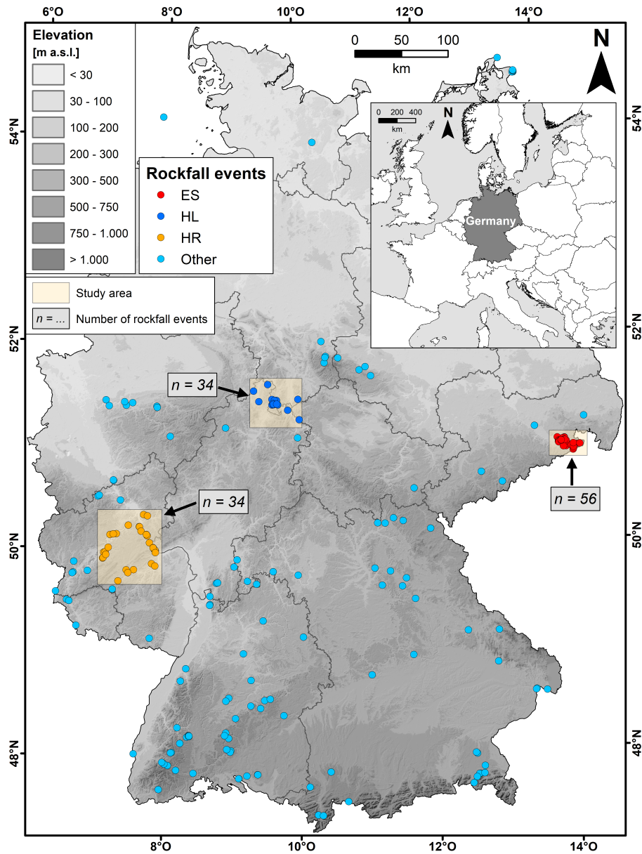
Figure 1. Location of rockfall events analysed in this study. Three distinct clusters ES (Elbe Sandstone), HL (Hesse and Lower Saxony) and HR (Hesse and Rhineland-Palatinate) are marked in red, blue and orange. All other events are coloured in light blue.
