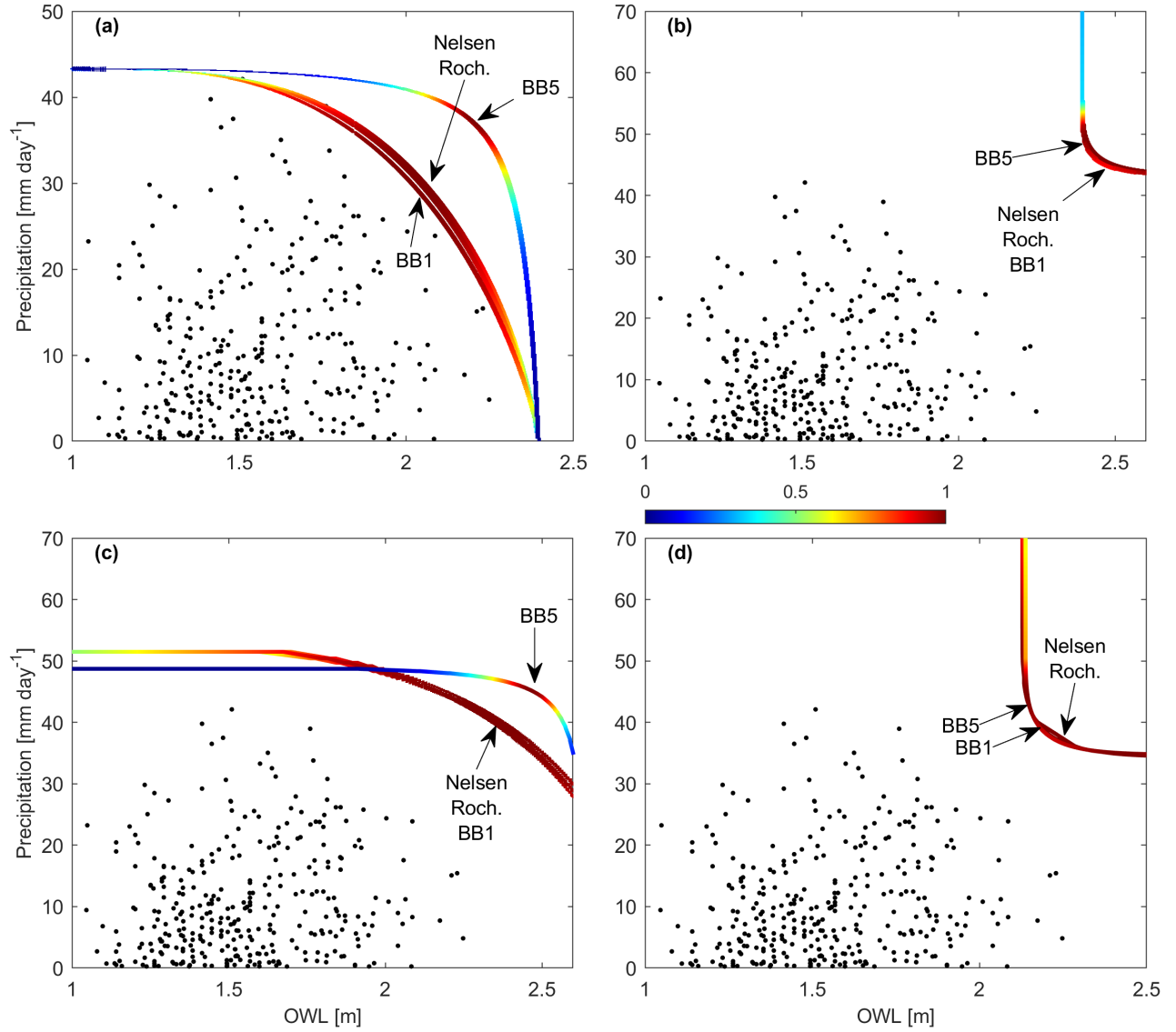
Figure 6. San Diego wet season monthly coinciding (a) AND, (b) OR, (c) SK, and (d) K hazard scenarios with the Nelsen, Roch-Alegre (Roch), BB1, and BB5 100-year isolines. Copula labels point to the mostly likely value on their respective isolines.
