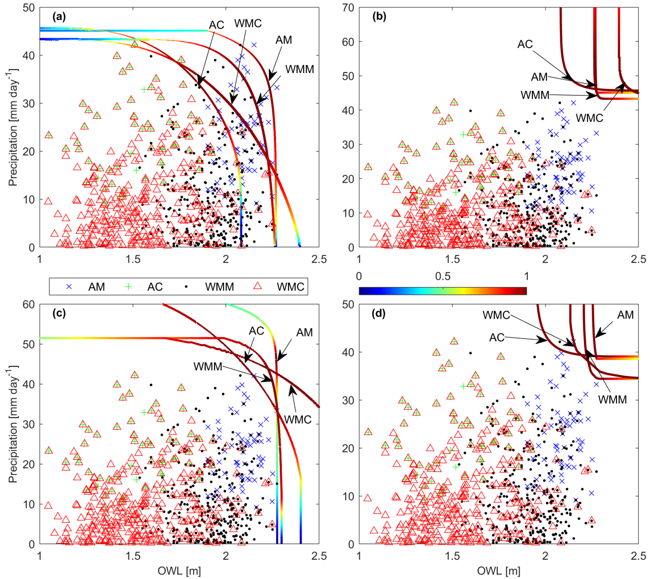
Figure 9. SD-San Diego (a) AND, (b) OR, (c) SK, and (d) K hazard scenarios for AM -annual maximum ( AM , cross), AC -annual coinciding ( AC , plus), WMM -wet season monthly maximum ( WMM , dot), WMC -wet season monthly coinciding ( WMC , triangle) data and 100-year isolines using the Fischer-Kock-BB1 copula. Sampling labels point to the mostly likely value on their respective isolines.
