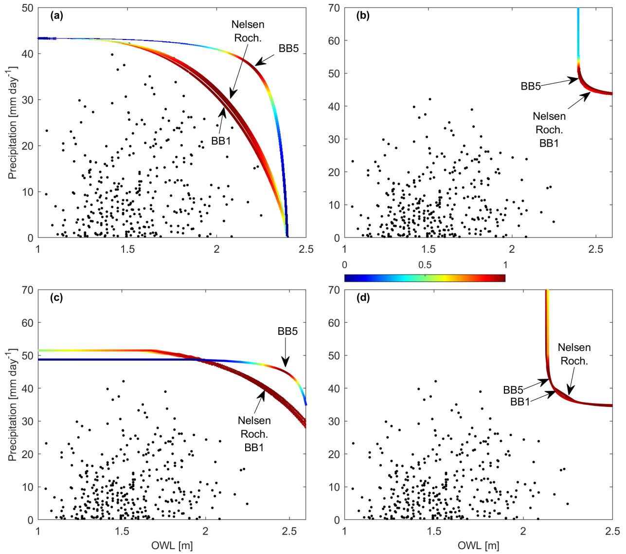
Figure 6. SD-WMC-San Diego wet season monthly coinciding (a) AND, (b) OR, (c) SK, and (d) K hazard scenarios with the Independent Nelsen , Cubic , Roch-Alegre (Roch) , Fischer-Kock BB1 , and Tawn BB5 100-year isolines. Copula labels point to the mostly likely value on their respective isolines. Most likely values outside the axis have a * with their respective copula label.
