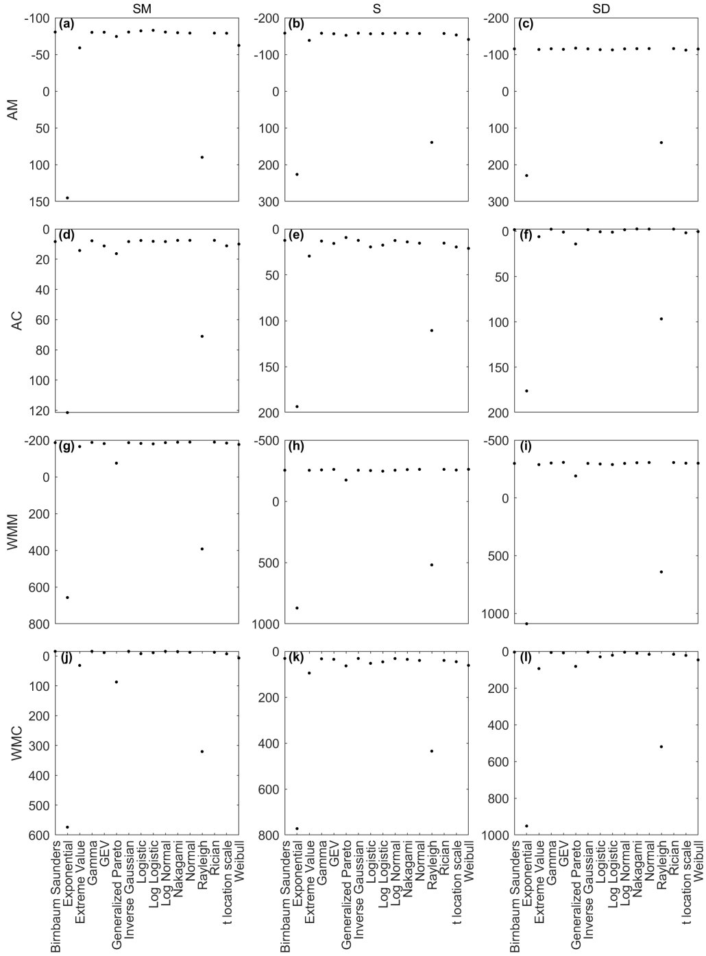
Figure A1. Marginal OWL BIC values per fitted copula for SM-Santa Monica (left column), S-Sunset (middle column), and SD-San Diego (right column) -Annual-Maximum-using annual maximum ((a), (b), (c); -Annual-Coinciding- , annual coinciding ((d), (e), (f); -Wet-Season Monthly-Maximum- , wet season monthly maximum ((g), (h), (i); - , and -Wet-Season Monthly-Coinciding- , wet season monthly coinciding ((j), (k), (l)). The Y-axis is orientated to display best BIC (top) to worst-worse BIC (bottom).
