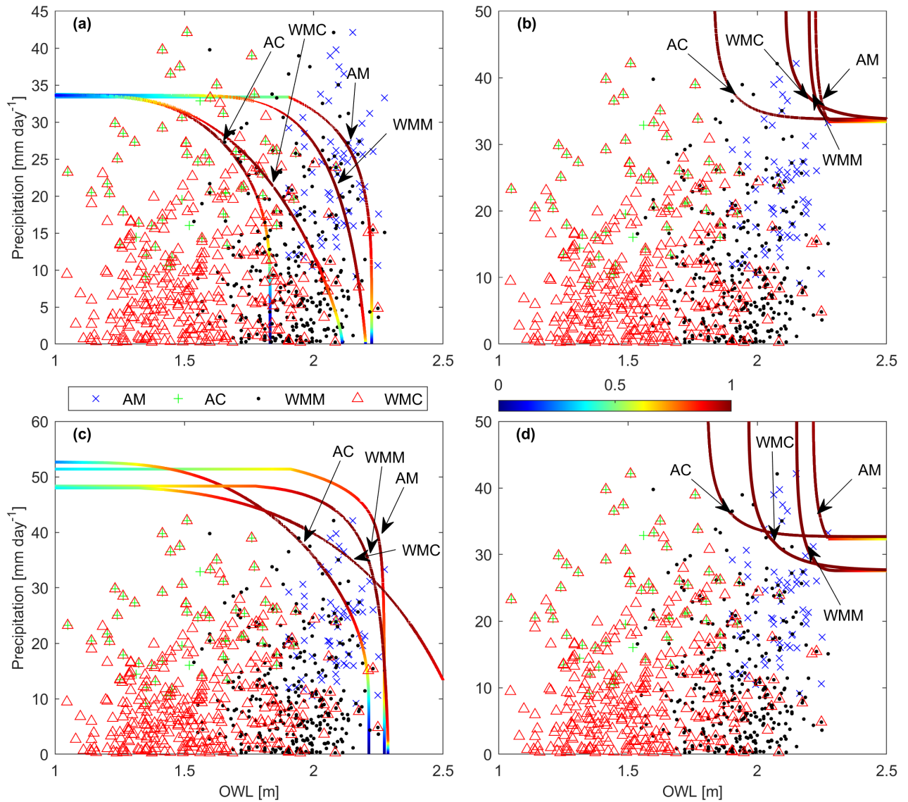
Figure 8. SD-San Diego (a) AND, (b) OR, (c) SK, and (d) K hazard scenarios for AM -annual maximum (AM, cross), AC -annual coinciding (AC, plus), WMM -wet season monthly maximum (WMM, dot), WMC -wet season monthly coinciding (WMC, triangle) data and 10-year isolines using the Fischer-Koerk-BB1 copula. Sampling labels point to the mostly likely value on their respective isolines.
