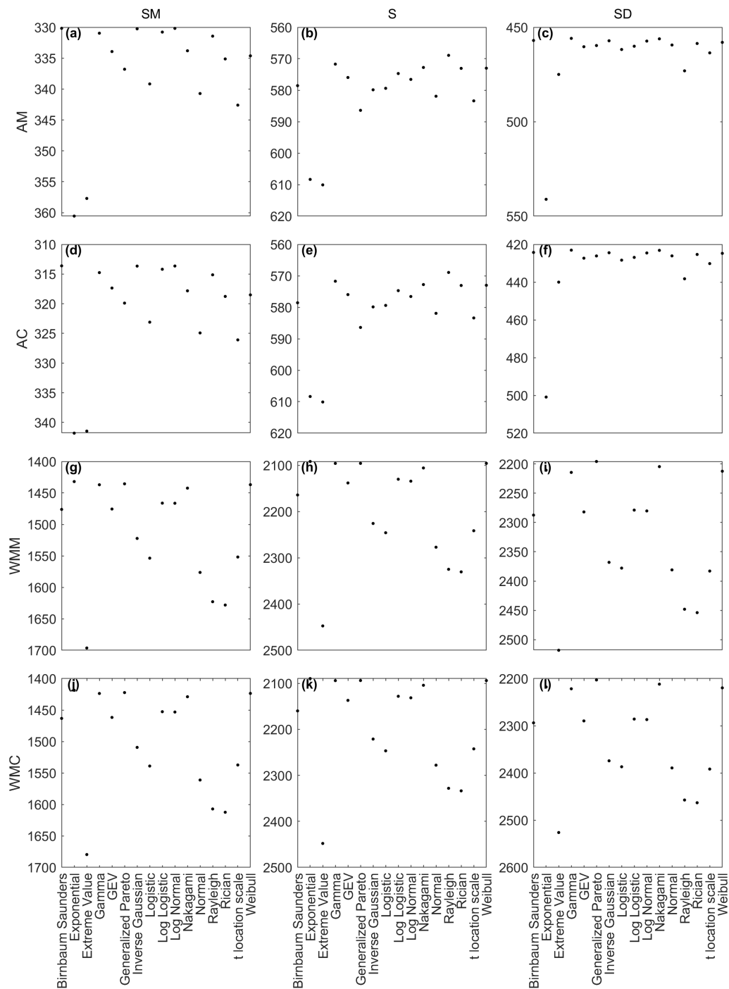
Figure A2. Marginal precipitation BIC values per fitted copula for SM Santa Monica (left column), S Sunset (middle column), and SD San Diego (right column). Annual-Maximum-using annual maximum ((a), (b), (c)), Annual-Coinciding , annual coinciding ((d), (e), (f)), Wet-Season-Monthly-Maximum , wet season monthly maximum ((g), (h), (i)), and Wet-Season-Monthly-Coinciding wet season monthly coinciding ((j), (k), (l)). The Y-axis is orientated to display best BIC (top) to worst BIC (bottom).
