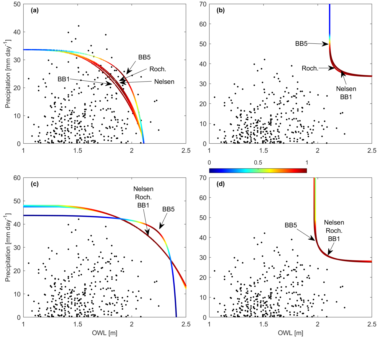
Figure 5. SD-WMC-San Diego wet season monthly coinciding (a) AND, (b) OR, (c) SK, and (d) K hazard scenarios with the Independent Nelsen , Cubic , Roch-Alegre (Roch) , Fischer-Kock BB1 , and Tawn BB5 10-year isolines. Copula labels point to the mostly likely value on their respective isolines. Most likely values outside the axis have a * with their respective copula label.
