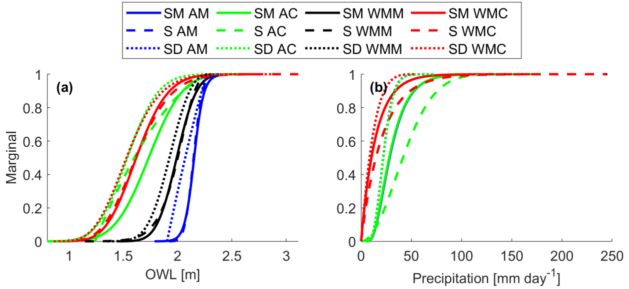
Figure 3. (a) OWL and (b) precipitation marginals for Santa Monica (SM, solid lines), Sunset (S, dashed lines), and San Diego (SD, dotted lines) using AM-annual maximum (AM, blue), AC-annual coinciding (AC, green), WMM-wet season monthly maximum (WMM, black), and WMC-wet season monthly coinciding (WMC, red) samplings.
