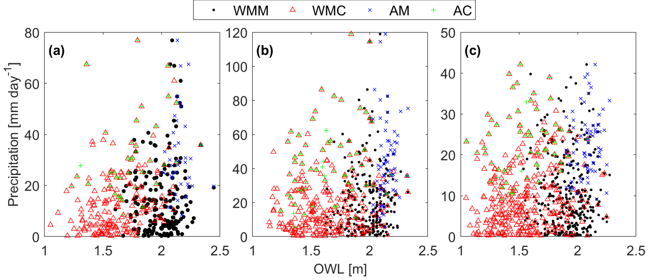
Figure 2. Data pairs for each sampling method. Annual Maximum annual maximum (AM, \times ), Annual Coinciding annual coinciding (AC, + ), Water Year Monthly Coinciding wet season monthly maximum (WMC, \triangle ), Water Year Monthly Maximum and wet season monthly coinciding (WMM, \bullet ) at (a) Santa Monica, (b) Sunset, and (c) San Diego
