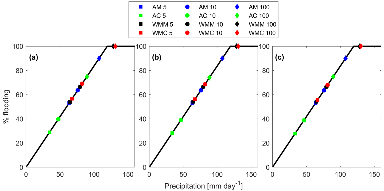
Figure 11. Structural scenario 5- (square), 10- (circle), and 100-year (diamond) return periods for AM-annual maximum (AM, blue), AC-annual coinciding (AC, green), WMM-wet season monthly maximum (WMM, black), and WMC-wet season monthly (WMC, red) data using the (a) Roch-AlegreNelsen , (b) Fischer-KoekRoch-Alegre , and (c) Tawn-BB1 copulas.
