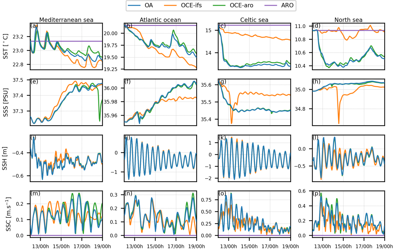
Figure 6. Temporal evolution of simulated sea surface temperature (SST, ^{\circ}\text{C} ), salinity (SSS, psu), height (SSH, m) and current speed (SSC, \text{m}\cdot\text{s}^{-1} ) extracted in the four areas presented in Figure 3d. Note that ARO does not have SSS nor SSH.
