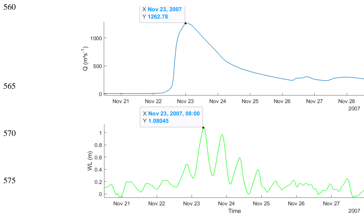
Figure D3. Validation event (22 - 25 November 2007) of river discharge at the flow gauge Swellendam (upper panel) and of the NTR at the tide gauge in Witsand (lower panel), between both peaks we estimated a time lag of 8 hours.
