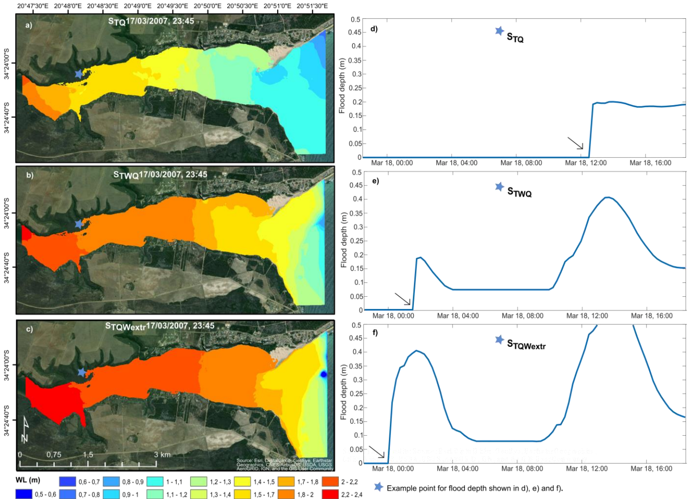
Figure 6. WLs of the scenarios S_{TQ} , S_{TQW} and S_{TQWextr} , extracted at the same time step (left panel) and time series of all three scenarios (right panel), showing the timing of the onset of the flood, extracted from the point, marked by the blue star.
