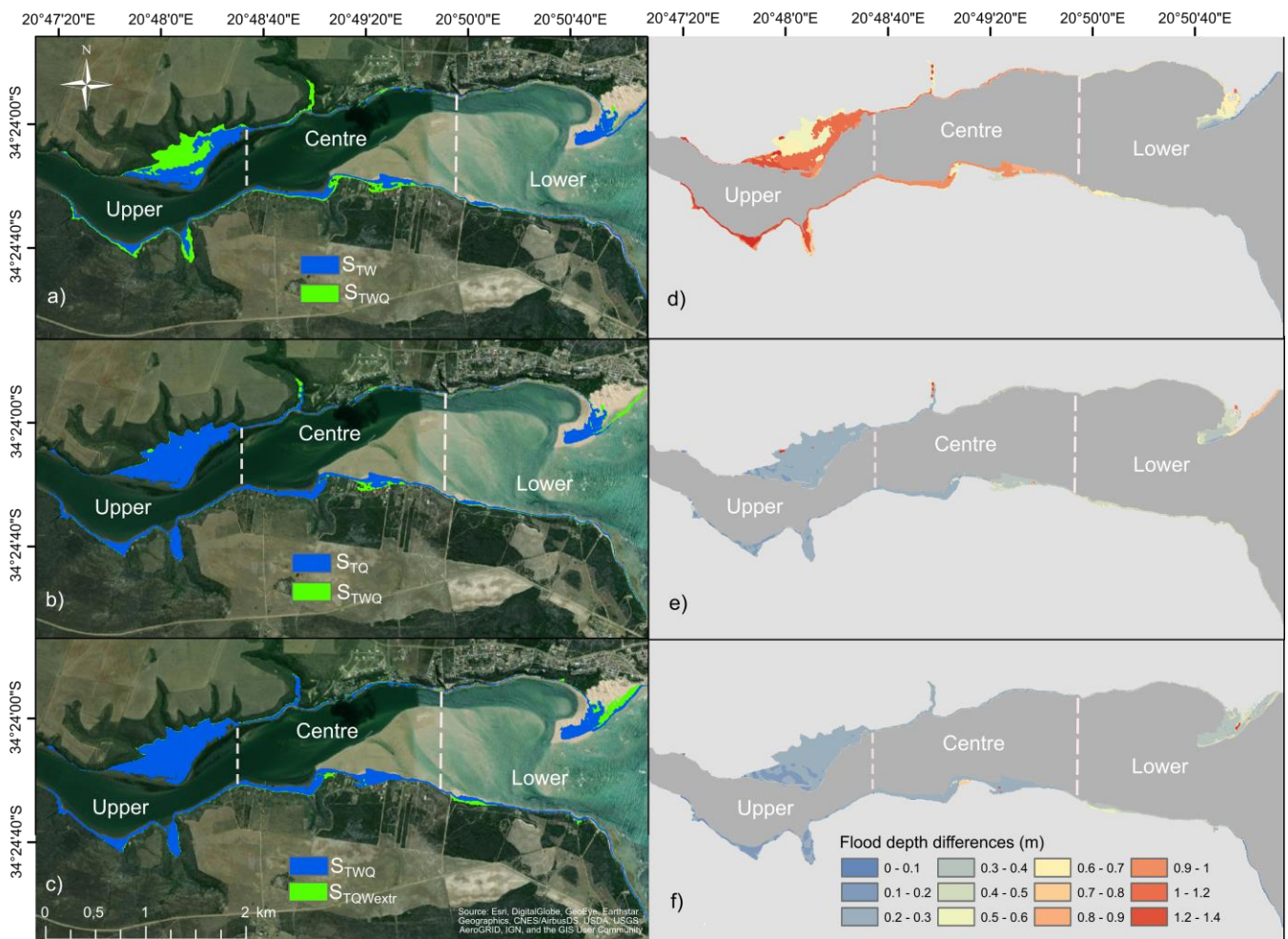
Figure 5. Comparison of flood extents of compound and excluding driver scenarios (left panel, a, b) and c)) and differences in flood depths (right panel). Panel d) shows the flood depths of S_{TWQ} - S_{TW} , e) shows S_{TWQ} - S_{TQ} and f) S_{TQW_{extr}} - S_{TWQ} .
